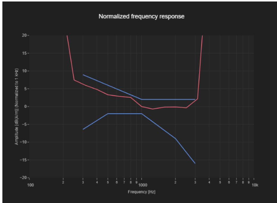
Figure B.1 Frequency Response of GSM 1900
