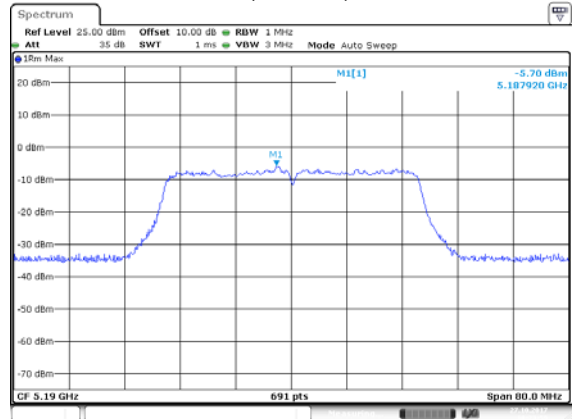
ANT 2(11N40)
