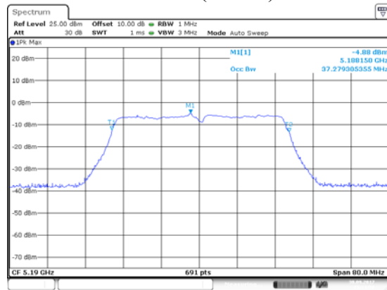
ANT 2(11N40)
