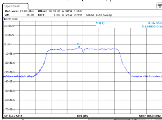
ANT 2(11N40)
