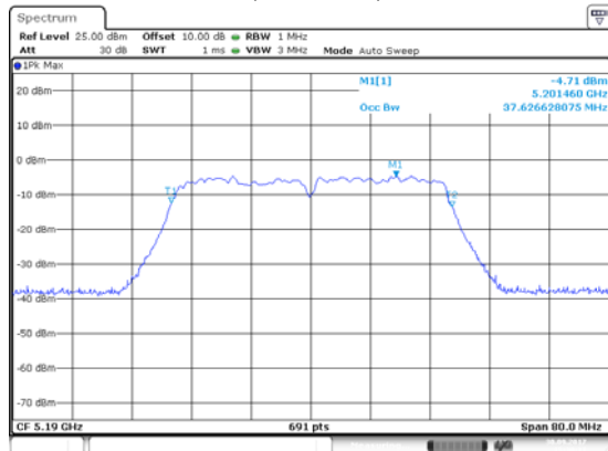
ANT 2(11AC40)
