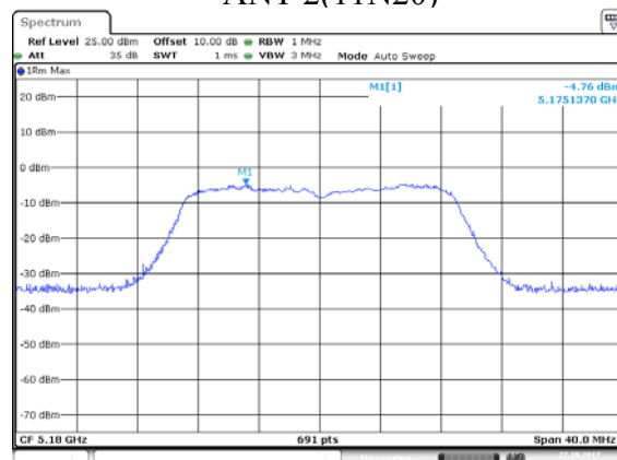
ANT 2(11N20)
