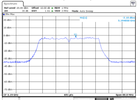
ANT 2(11AC40)
