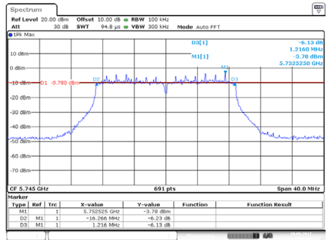
ANT 2(802.11ac20)
