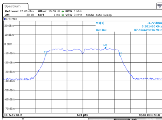
ANT 1(11AC40)
