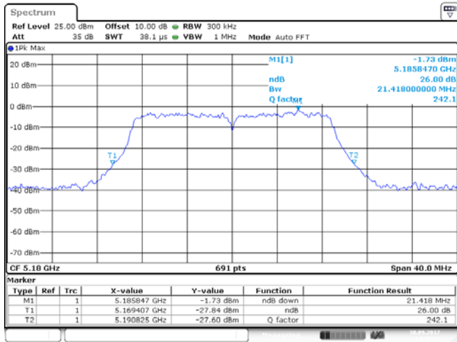
ANT 1(11N20)
