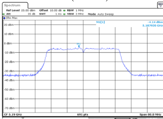
ANT 1(11AC40)
