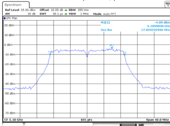
ANT 2(11N20)
