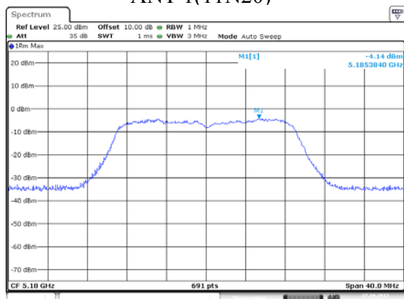
ANT 1(11N20)
