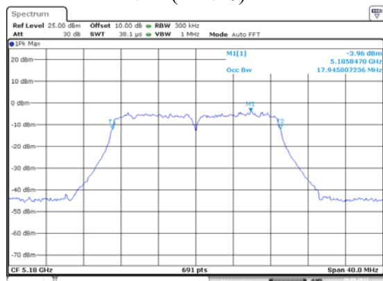
ANT 1(11N20)
