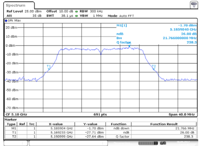
ANT 2(11N20)
