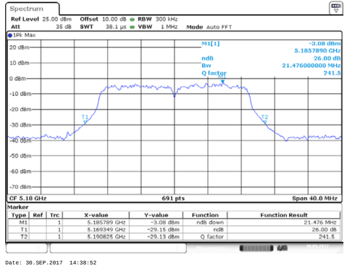
ANT 2(802.11ac20)
