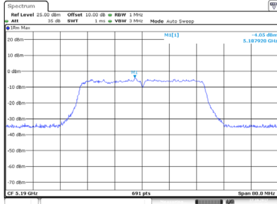
ANT 2(11AC40)
