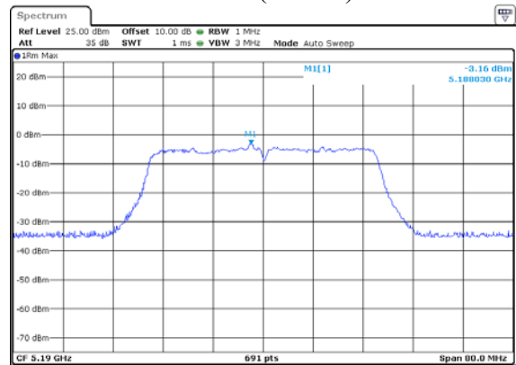
ANT 2(11N40)
