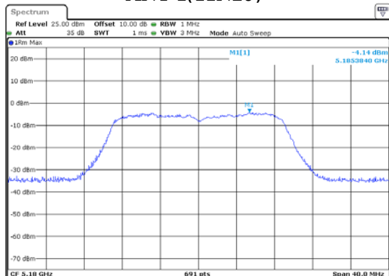
ANT 1(11N20)
