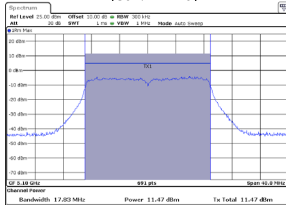
ANT 2(802.11 N20)
