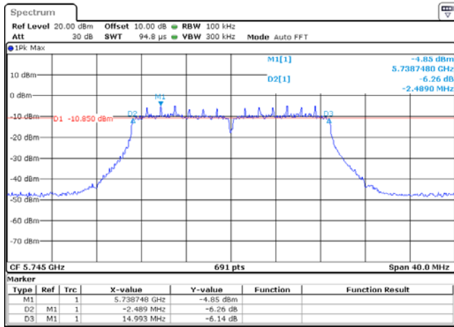
ANT 1(802.11N20)
