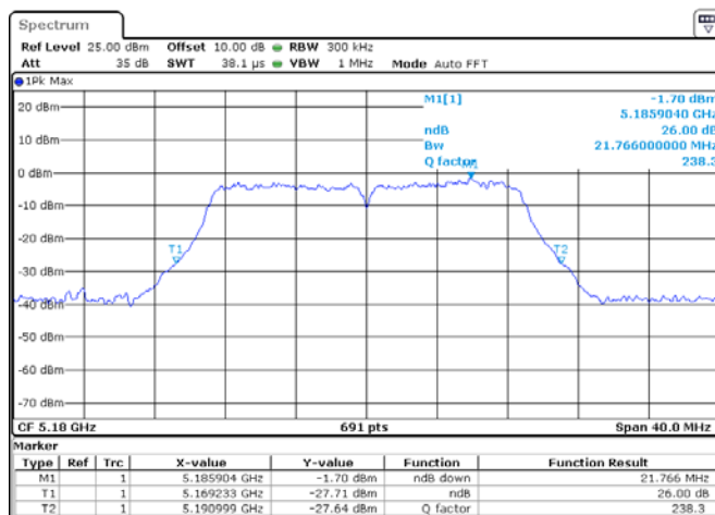
ANT 2(11N20)
