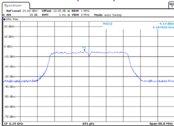
ANT 1(11AC40)
