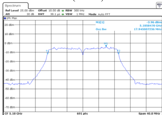
ANT 1(11N20)
