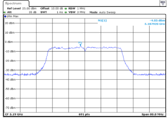
ANT 2(11AC40)
