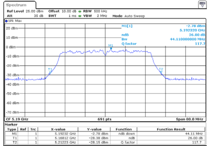
ANT 2(802.11ac40)
