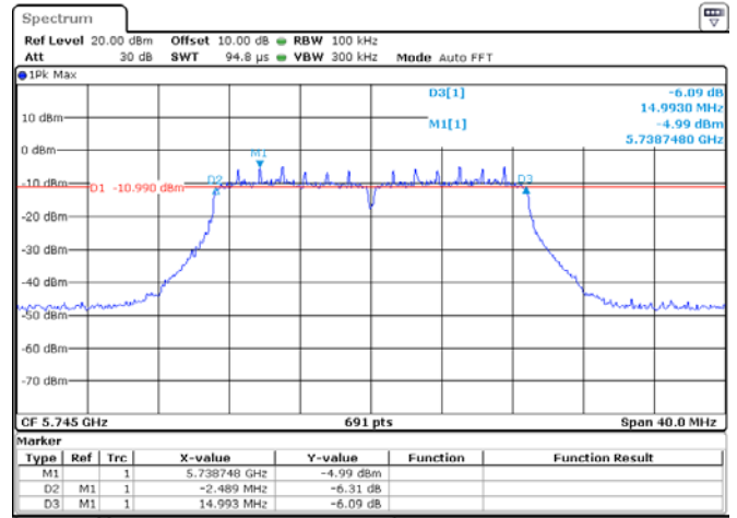
ANT 2(802.11N20)
