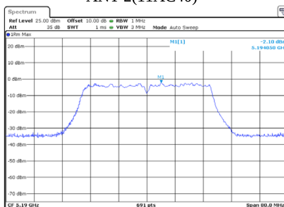
ANT 2(11AC40)
