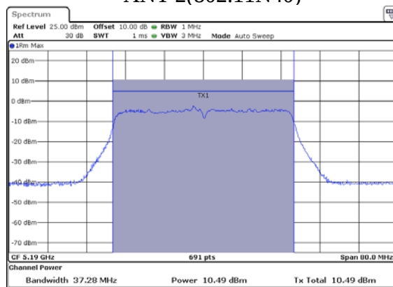
ANT 2(802.11N40)
