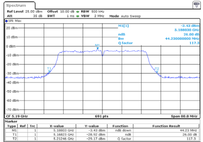
ANT 2(802.11n40)
