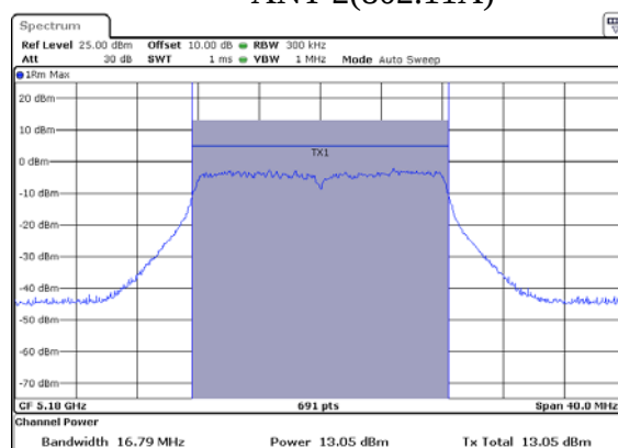
ANT 2(802.11A)
