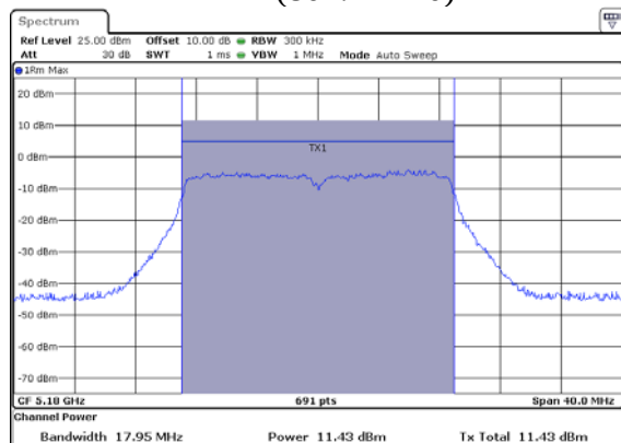
ANT 1(802.11N20)
