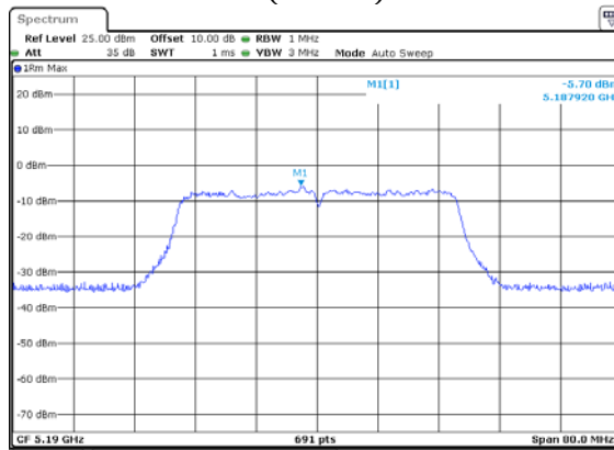
ANT 2(11N40)
