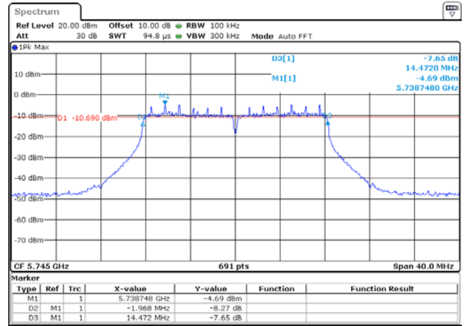
ANT 2(802.11A)
