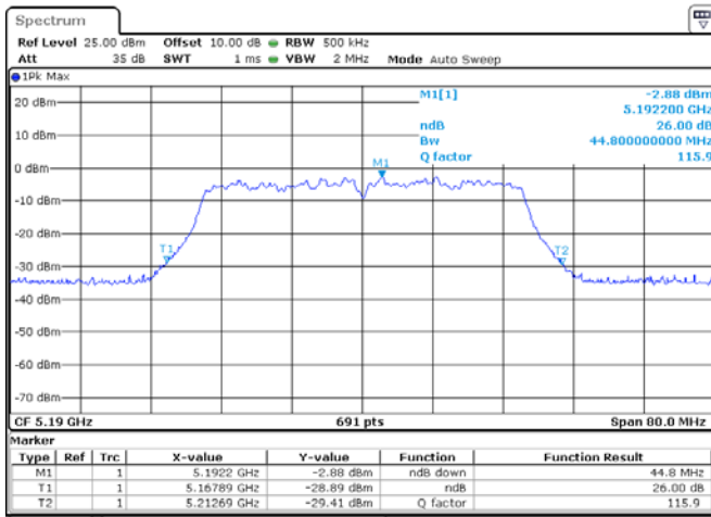
ANT 1(802.11ac40)
