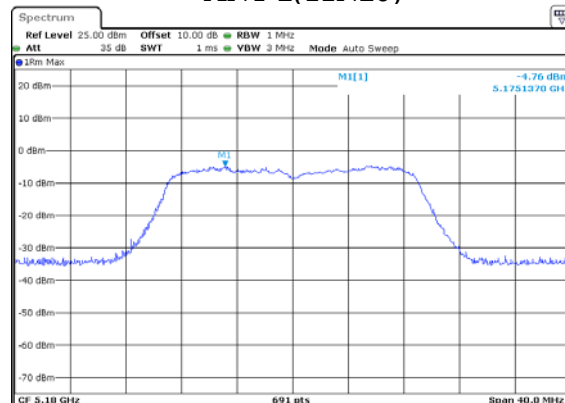
ANT 2(11N20)
