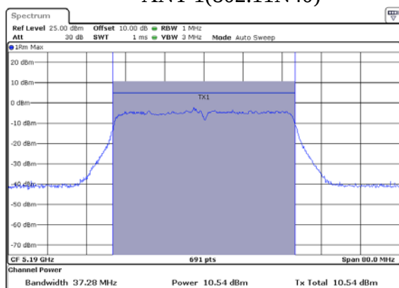
ANT 1(802.11N40)
