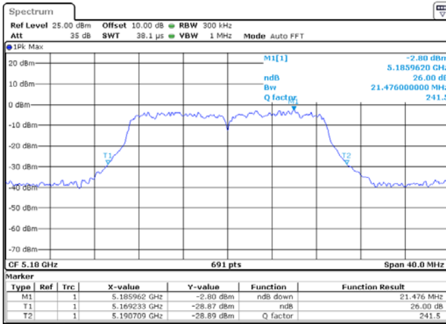
ANT 1(802.11ac20)
