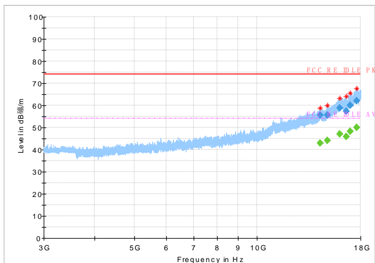
Fig.48 Radiated emission: \pi/4 DQPSK, Ch0, 3GHz~18GHz
