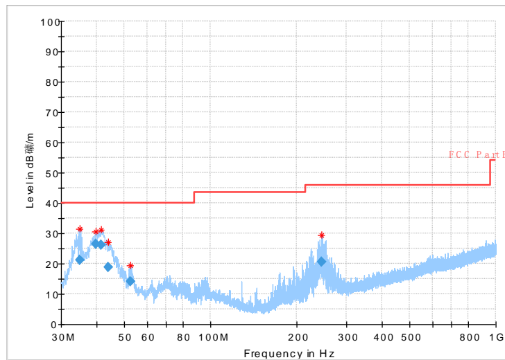
Fig.46 Radiated emission: \pi/4 DQPSK, Ch0, 30MHz~1GHz
