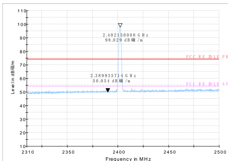
Fig.49 Radiated emission (Power): \pi/4 DQPSK, low channel
