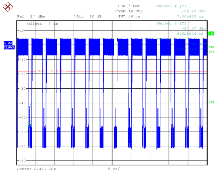
Fig.75 Number of Transmissions Measurement: Ch39, Packet 3-DH5
