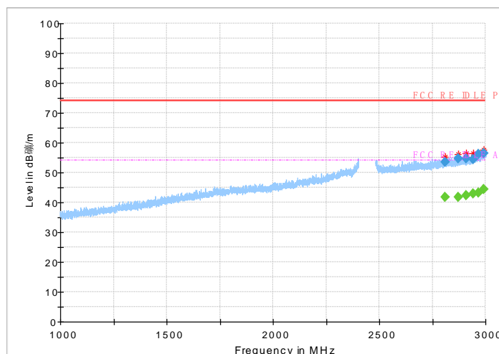
Fig.24 Radiated emission: Ch39, 1GHz~3GHz
