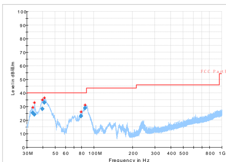
Fig.18 Radiated emission: Ch0, 30MHz~1GHz
