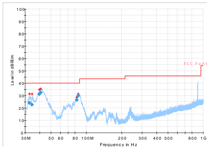
Fig.23 Radiated emission: Ch39, 30MHz~1GHz
