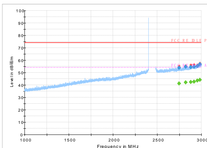
Fig.19 Radiated emission: Ch0, 1GHz~3GHz
