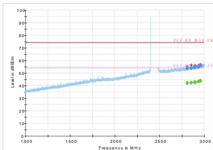
Fig.47 Radiated emission: \pi/4 DQPSK, Ch0, 1GHz~3GHz
