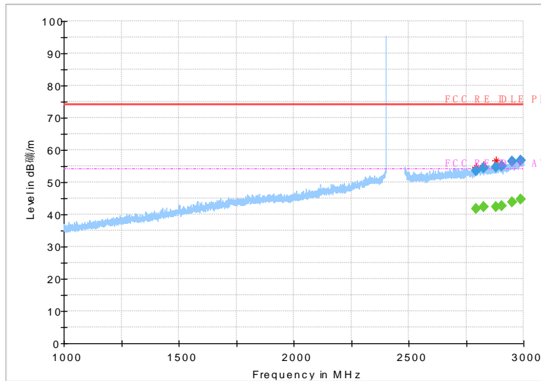
Fig.53 Radiated emission: 8DPSK, Ch0, 1GHz~3GHz
