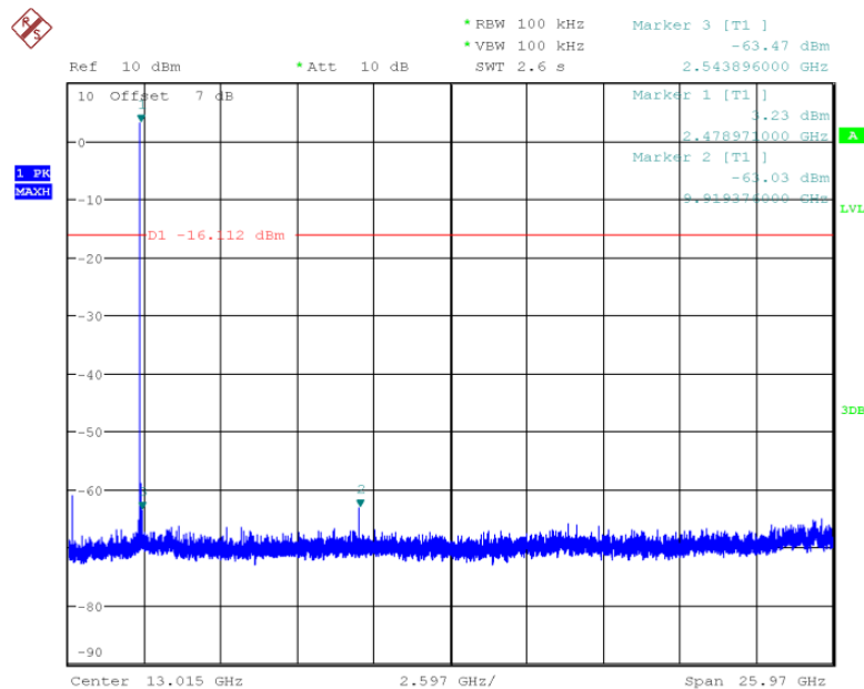
Fig.38 Conducted spurious emission: 8DPSK, Ch78, 2480MHz
