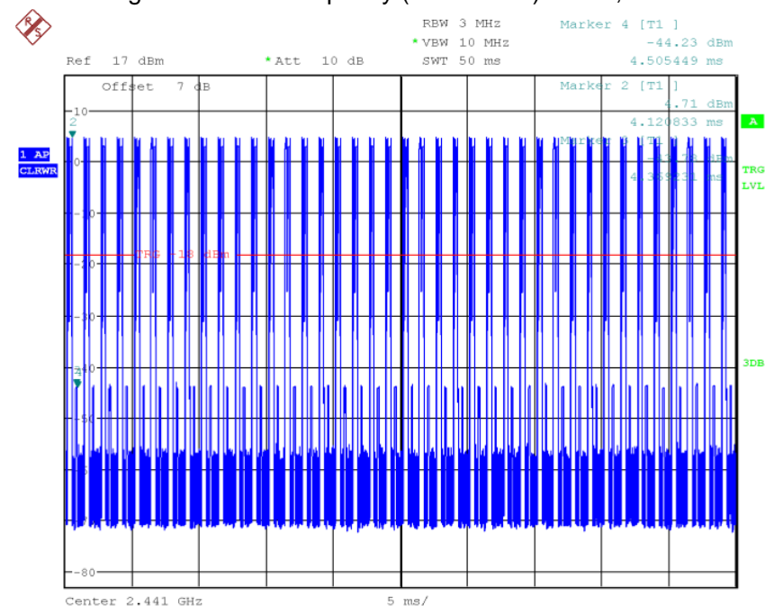
Fig.64 Time of occupancy (Dwell Time): Ch39,Packet 2-DH1
