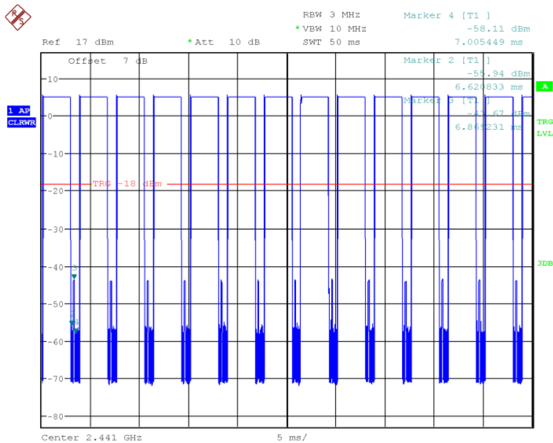
Fig.62 Time of occupancy (Dwell Time): Ch39,Packet DH5
