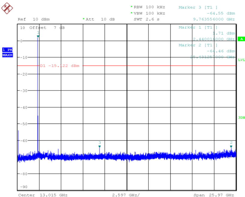
Fig.24 Conducted spurious emission: GFSK, Ch39, 2441MHz
