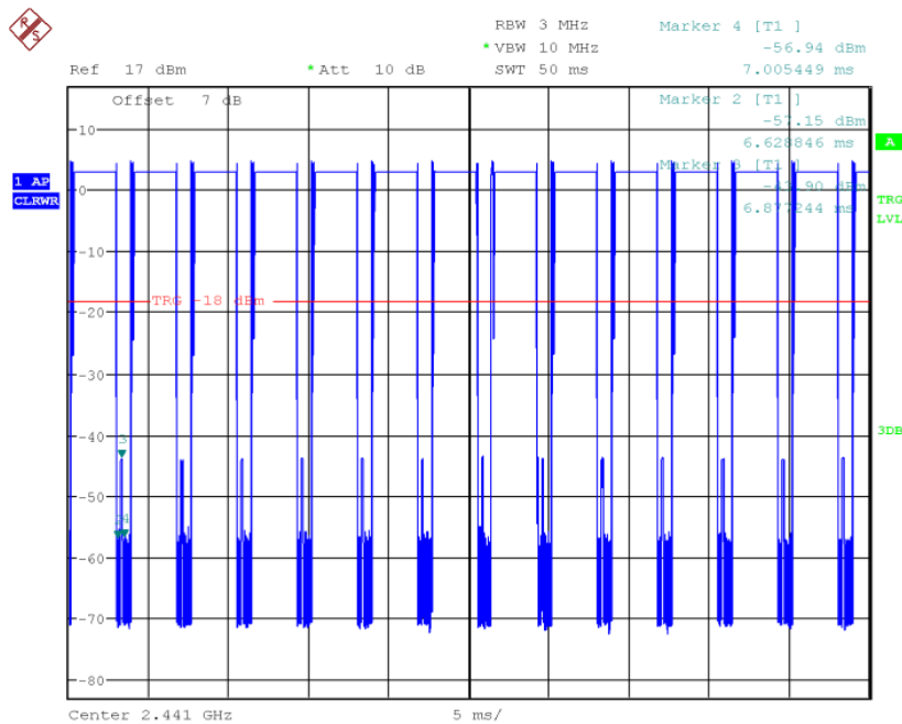
Fig.68 Time of occupancy (Dwell Time): Ch39,Packet 2-DH5
