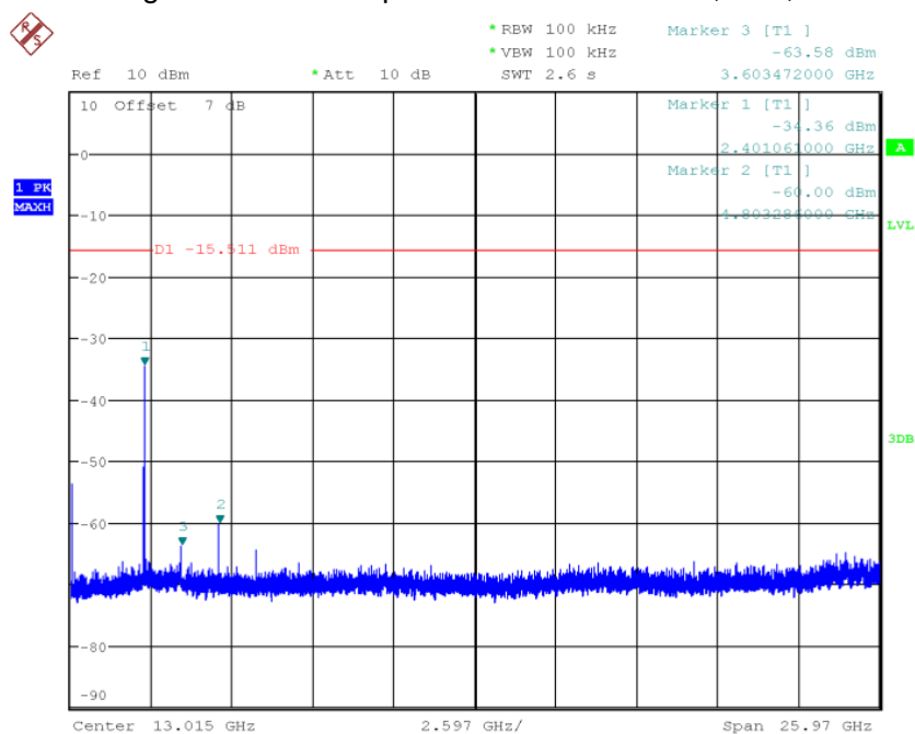
Fig.22 Conducted spurious emission: GFSK, Ch0, 2402MHz
