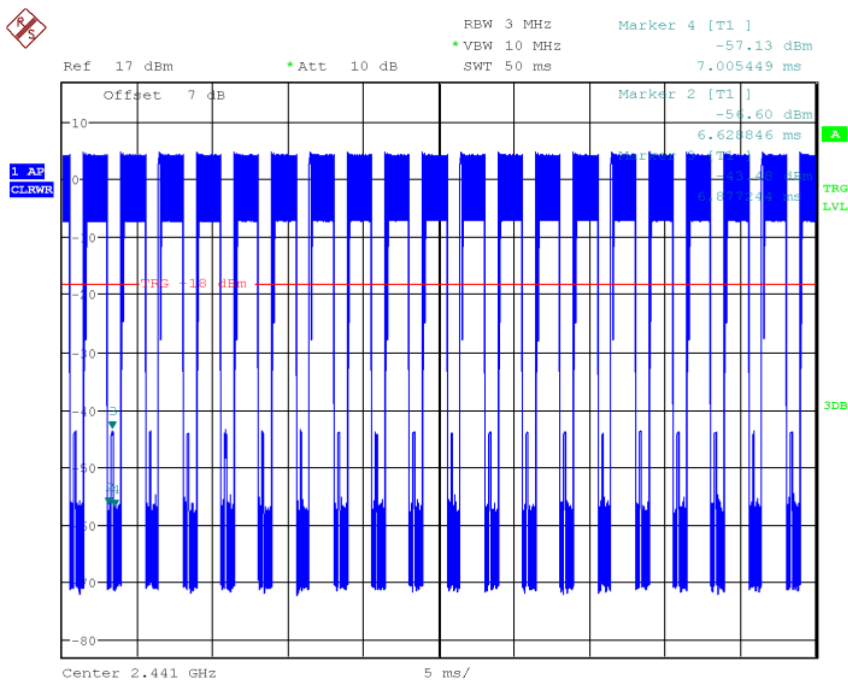
Fig.72 Time of occupancy (Dwell Time): Ch39,Packet 3-DH3
