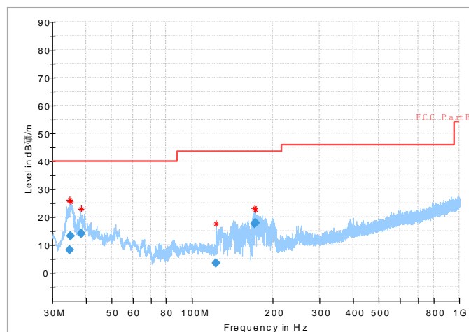
Fig.46 Radiated emission: \pi/4 DQPSK, Ch0, 30MHz~1GHz
