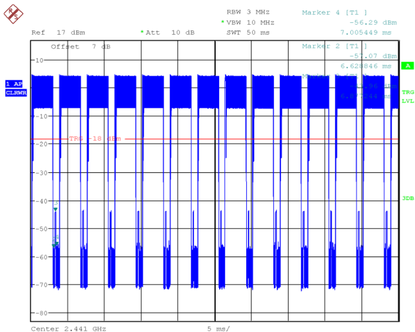
Fig.74 Time of occupancy (Dwell Time): Ch39,Packet 3-DH5
