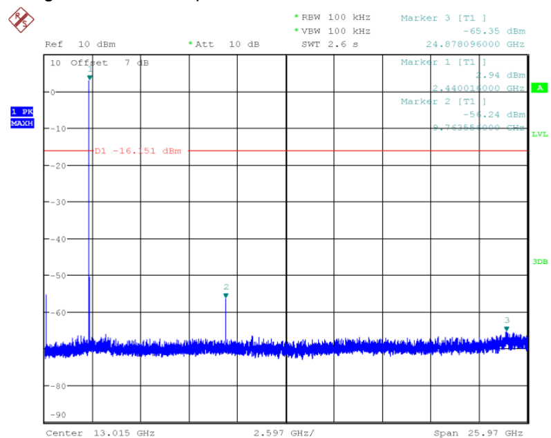
Fig.30 Conducted spurious emission: \pi/4 DQPSK, Ch39, 2441MHz
