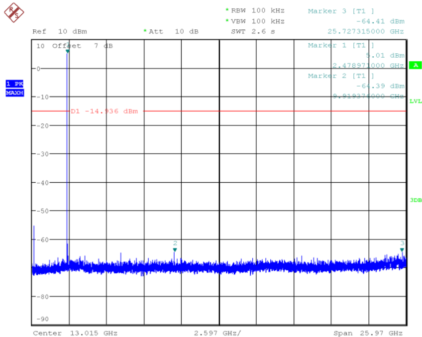
Fig.26 Conducted spurious emission: GFSK, Ch78, 2480MHz
