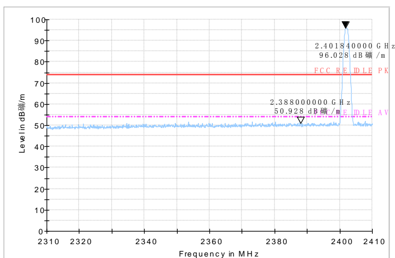
Fig.43 Radiated emission (Power): GFSK, low channel
