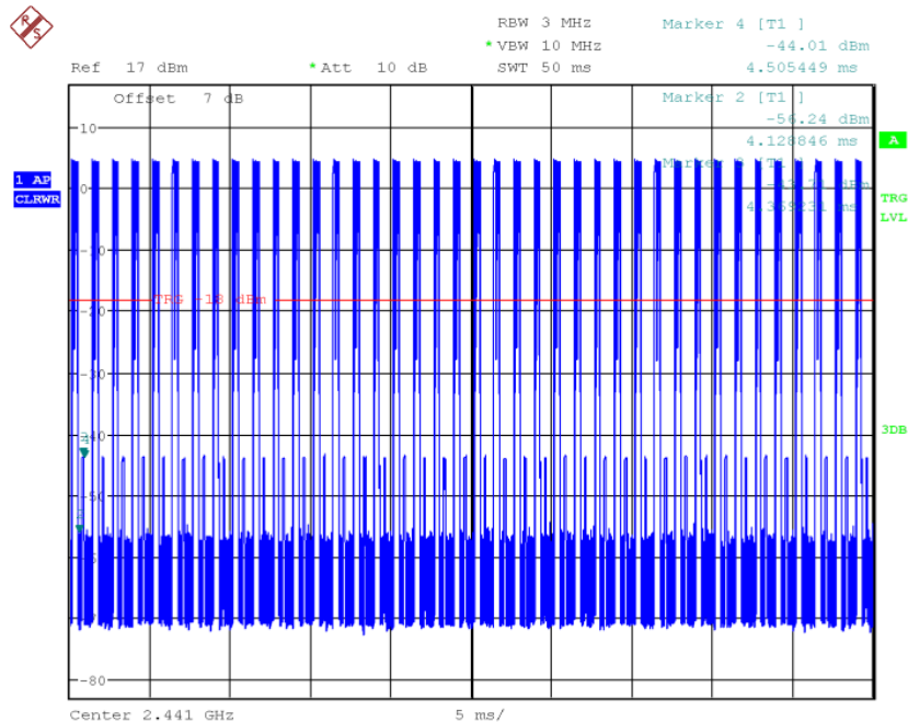
Fig.70 Time of occupancy (Dwell Time): Ch39,Packet 3-DH1
