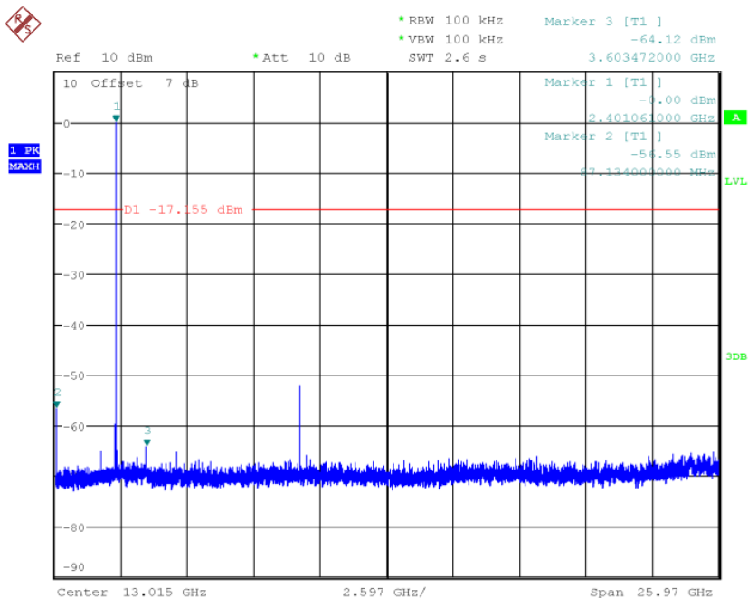
Fig.34 Conducted spurious emission: 8DPSK, Ch0, 2402MHz
