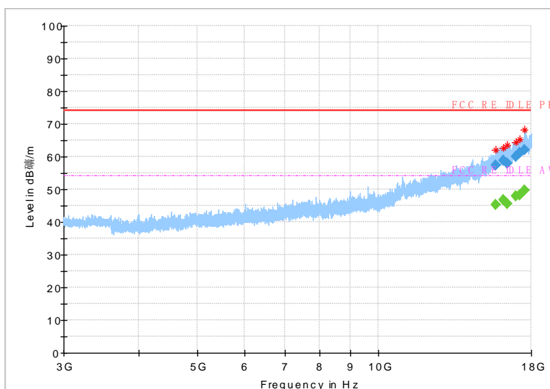
Fig.54 Radiated emission: 8DPSK, Ch0, 3GHz~18GHz
