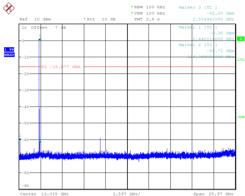
Fig.36 Conducted spurious emission: 8DPSK, Ch39, 2441MHz
