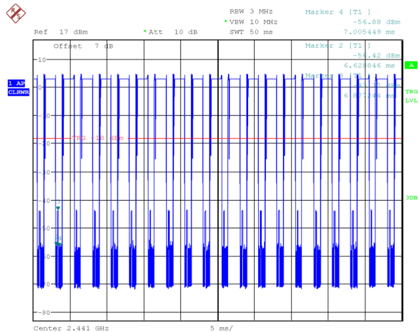
Fig.66 Time of occupancy (Dwell Time): Ch39,Packet 2-DH3
