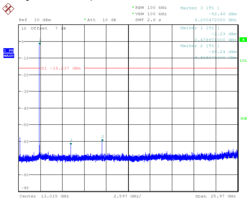
Fig.32 Conducted spurious emission: \pi/4 DQPSK, Ch78, 2480MHz
