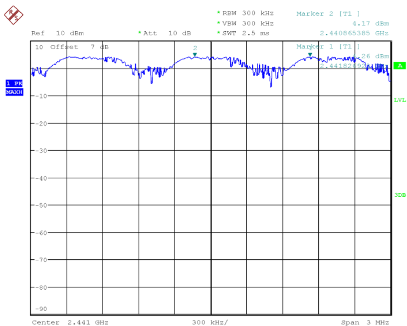
Fig.85 Carrier separation measurement: GFSK, Ch39
