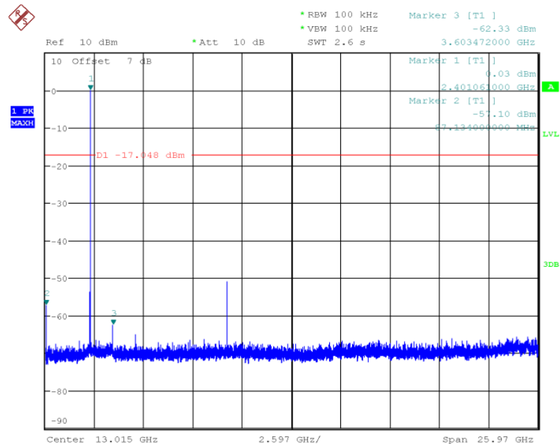
Fig.28 Conducted spurious emission: \pi/4 DQPSK, Ch0, 2402MHz
