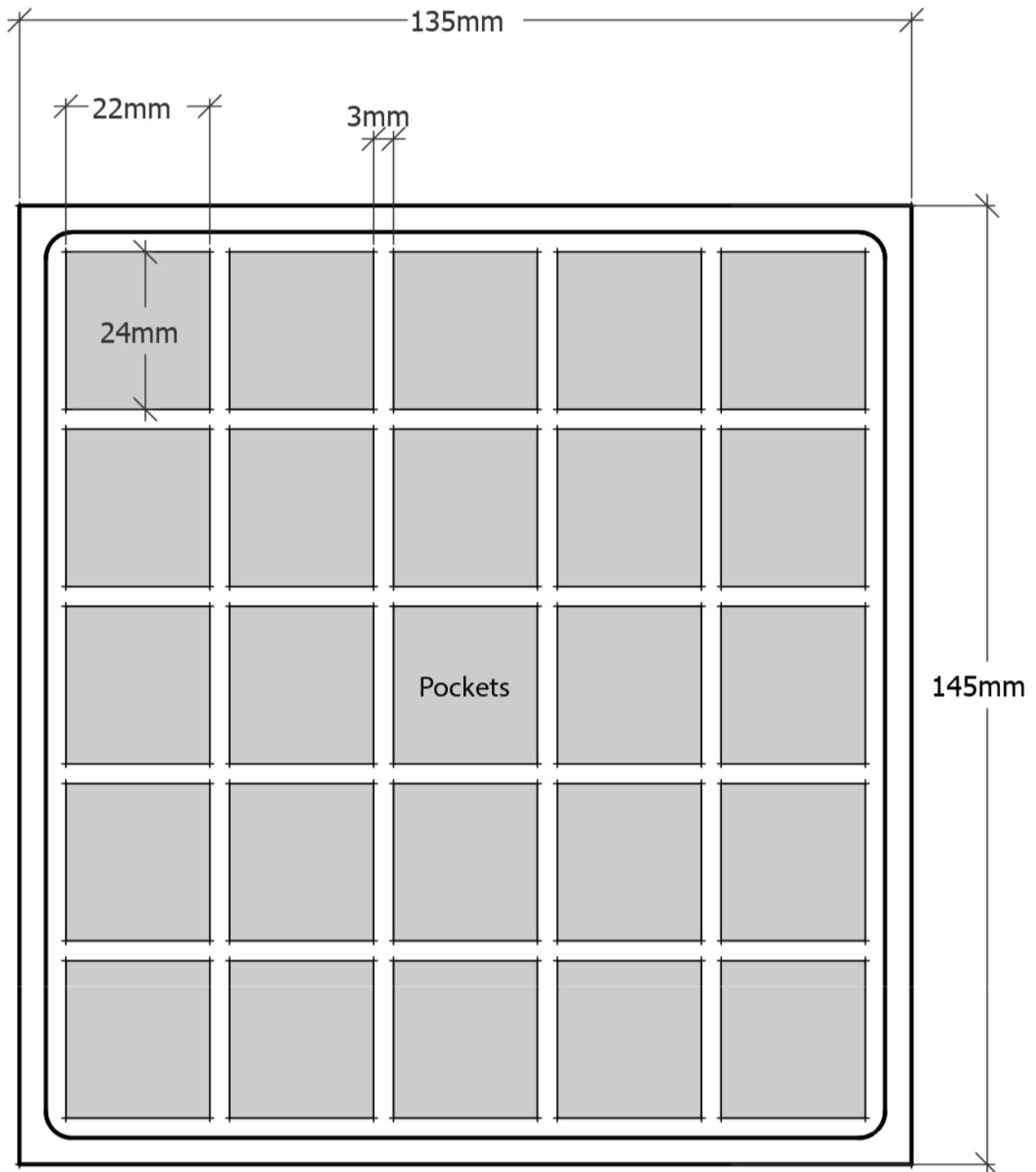
Figure: SM1251SMD Antistatic ESD Tray Dimensions for 5x5 pcs
