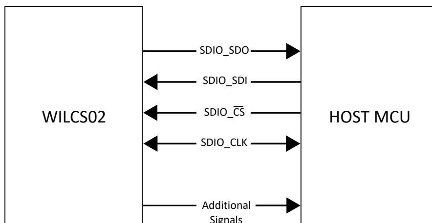
Figure 2-7. WILCS02 Module Host Interface Diagram
