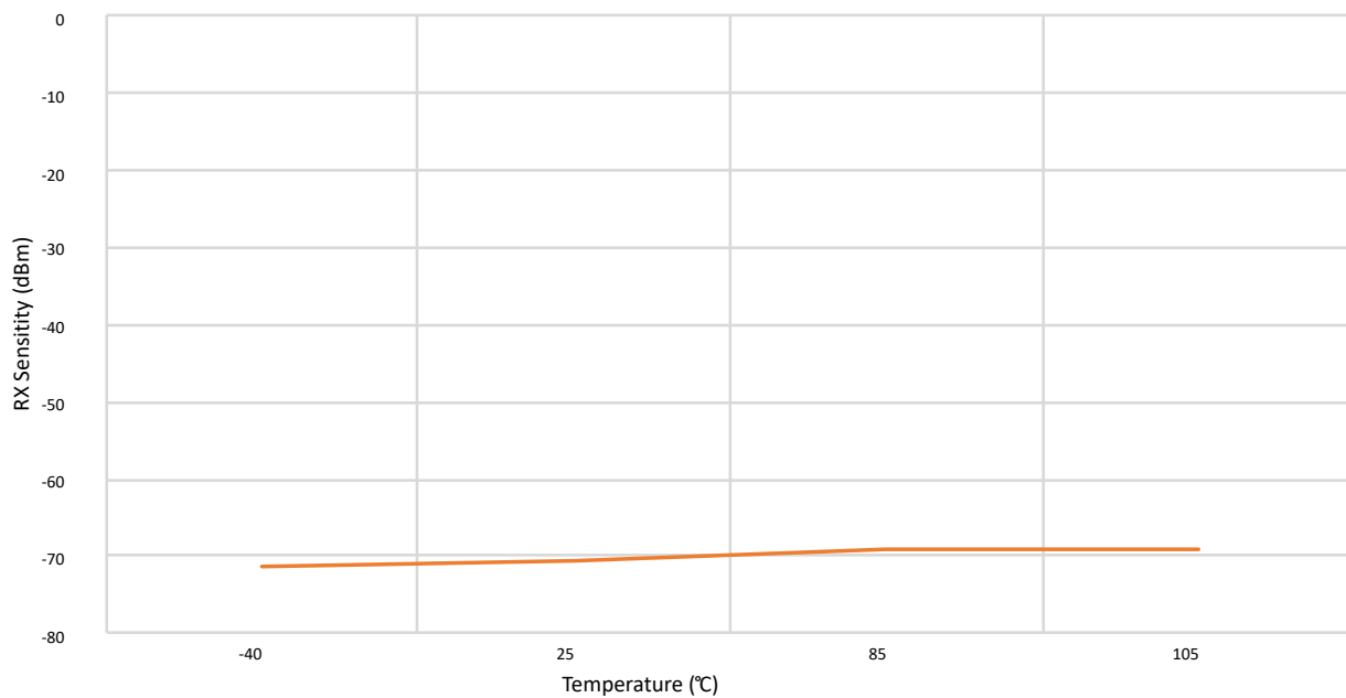
Figure 3-14. RX Sensitivity vs Temperature, MCS7, Channel 7, 3.3V
