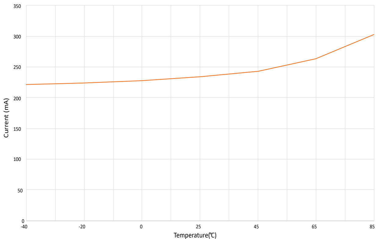
Figure 3-17. Transmit Current vs Temperature, MCS7, Channel 7, 3.3V
