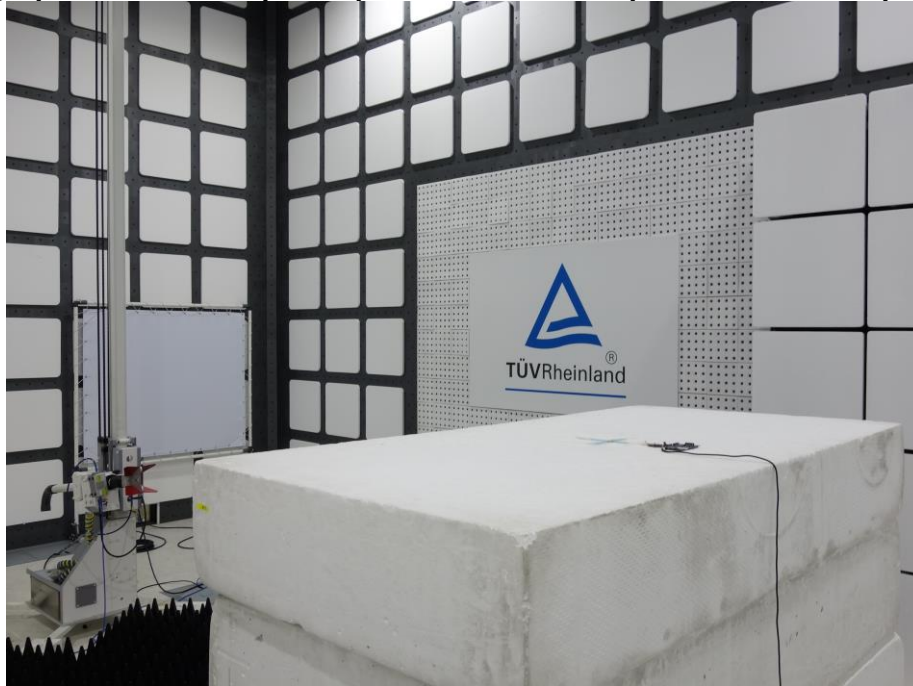
Photograph 13: Test Setup for Spurious Emissions (Back View 3, WiFi)
