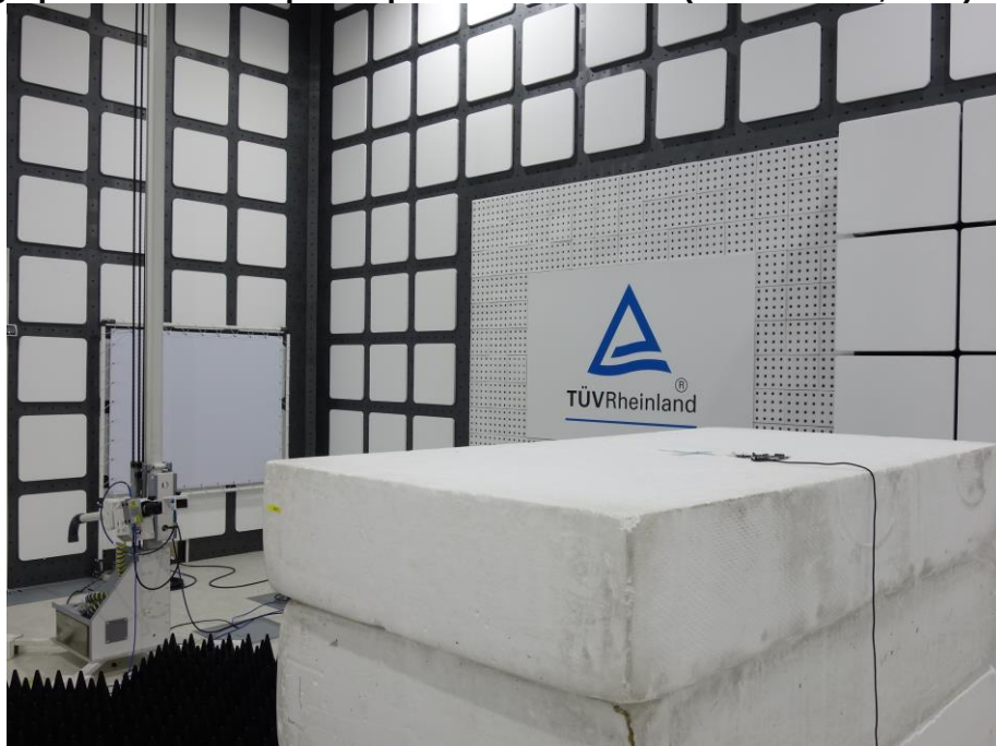
Photograph 14: Test Setup for Spurious Emissions (Back View 4, WiFi)
