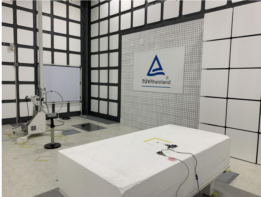
Photograph 3: Test Setup for Spurious Emissions (Back View 1, BLE)
