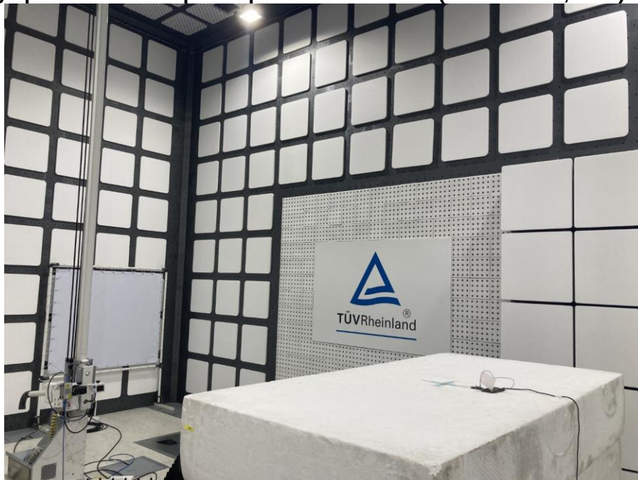
Photograph 46: Test Setup for Spurious Emissions (Back View 4, WiFi)
