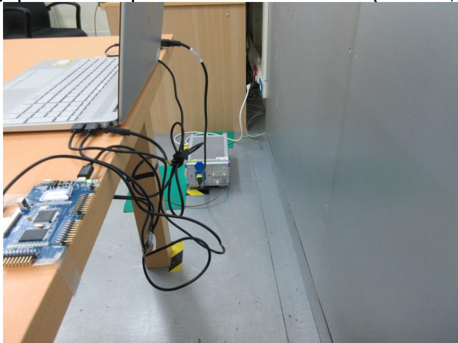
Photograph 16: Test Setup for Mains Conducted Emissions (Back View, BLE)
