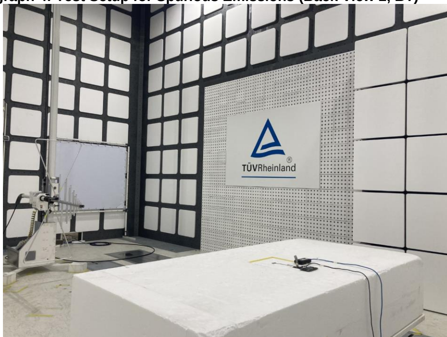
Photograph 4: Test Setup for Spurious Emissions (Back View 2, BT)
