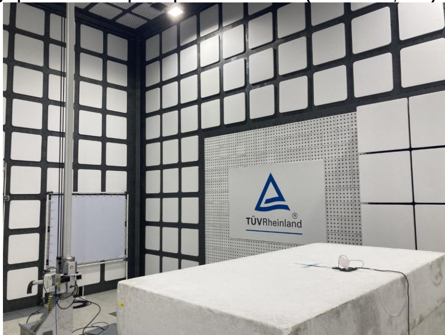
Photograph 22: Test Setup for Spurious Emissions (Back View 4, WiFi)
