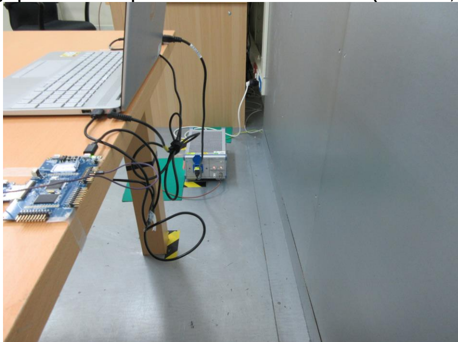
Photograph 24: Test Setup for Mains Conducted Emissions (Back View, WiFi)
