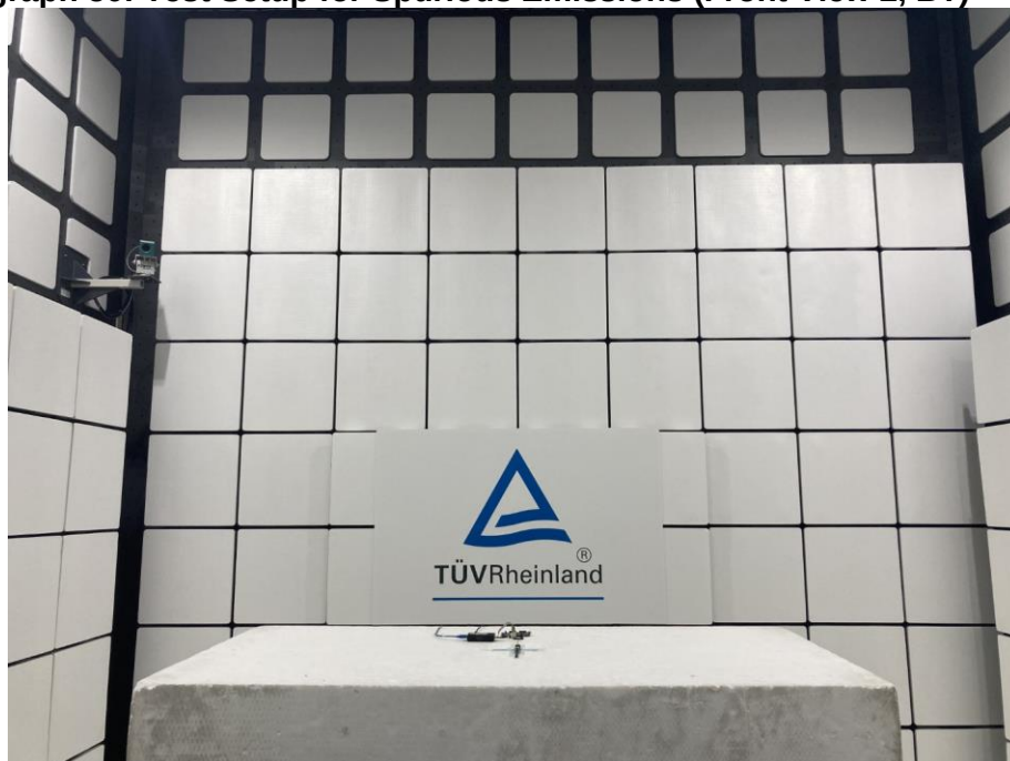
Photograph 50: Test Setup for Spurious Emissions (Front View 2, BT)
