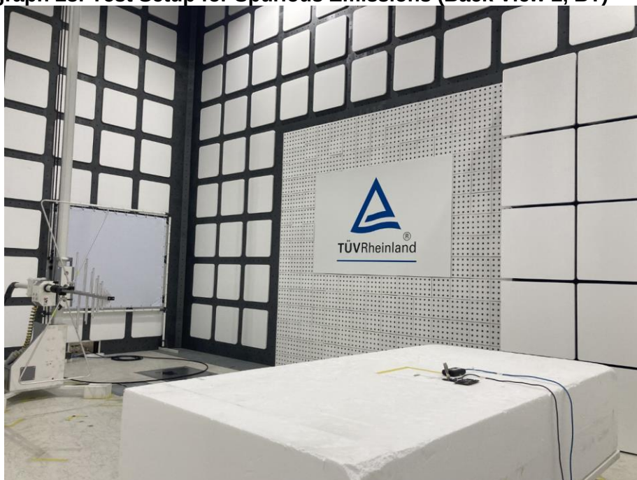
Photograph 28: Test Setup for Spurious Emissions (Back View 2, BT)
