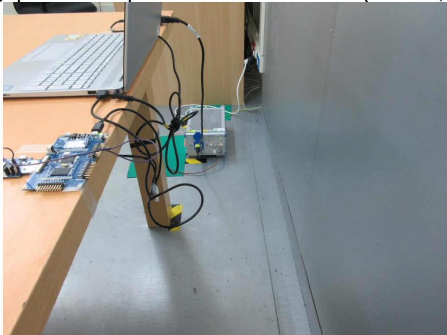
Photograph 72: Test Setup for Mains Conducted Emissions (Back View, WiFi)
