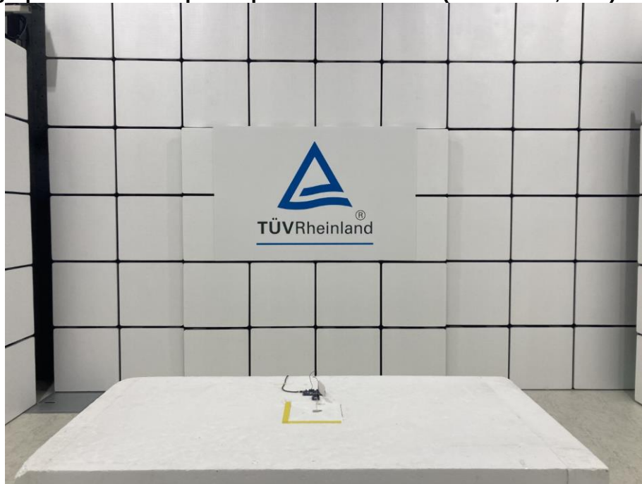
Photograph 41: Test Setup for Spurious Emissions (Front View, WiFi)
