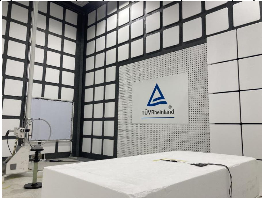
Photograph 60: Test Setup for Spurious Emissions (Back View 2, BLE)
