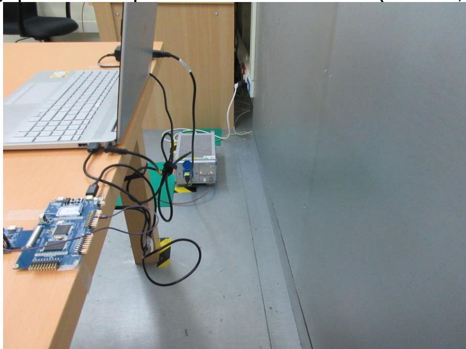
Photograph 48: Test Setup for Mains Conducted Emissions (Back View, WiFi)
