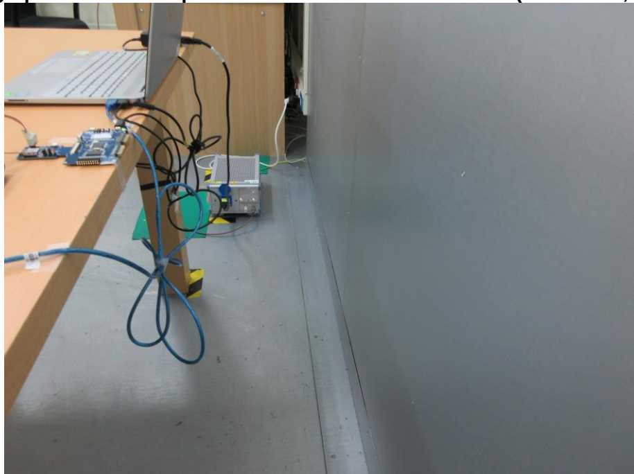
Photograph 56: Test Setup for Mains Conducted Emissions (Back View, BT)
