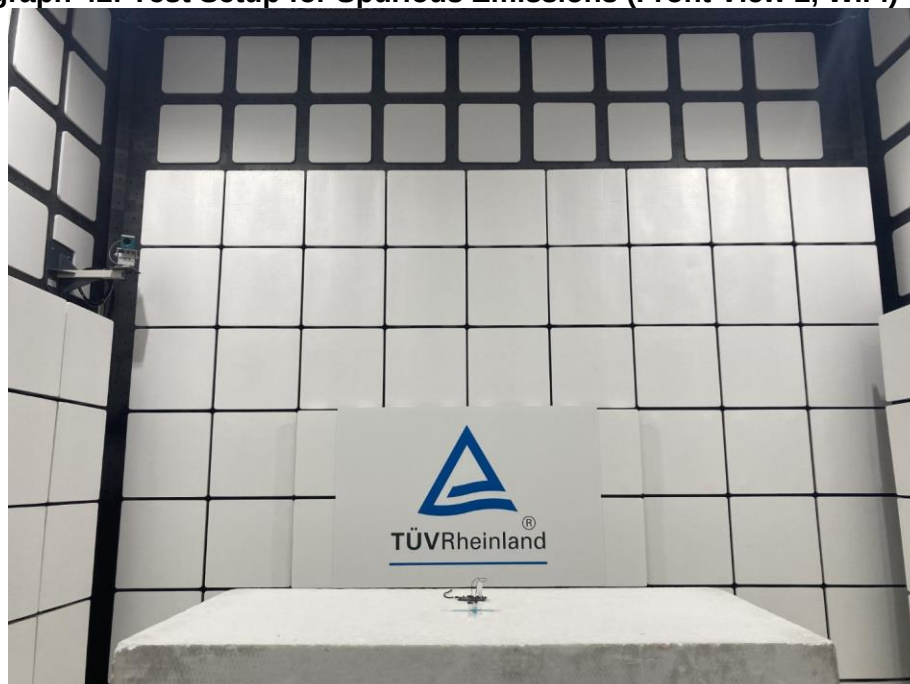
Photograph 42: Test Setup for Spurious Emissions (Front View 2, WiFi)
