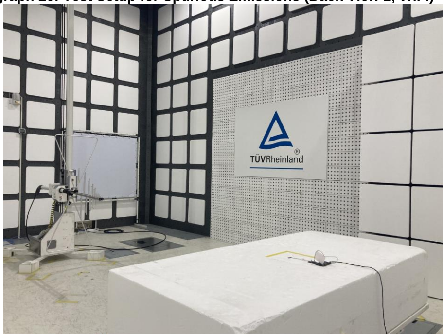
Photograph 20: Test Setup for Spurious Emissions (Back View 2, WiFi)
