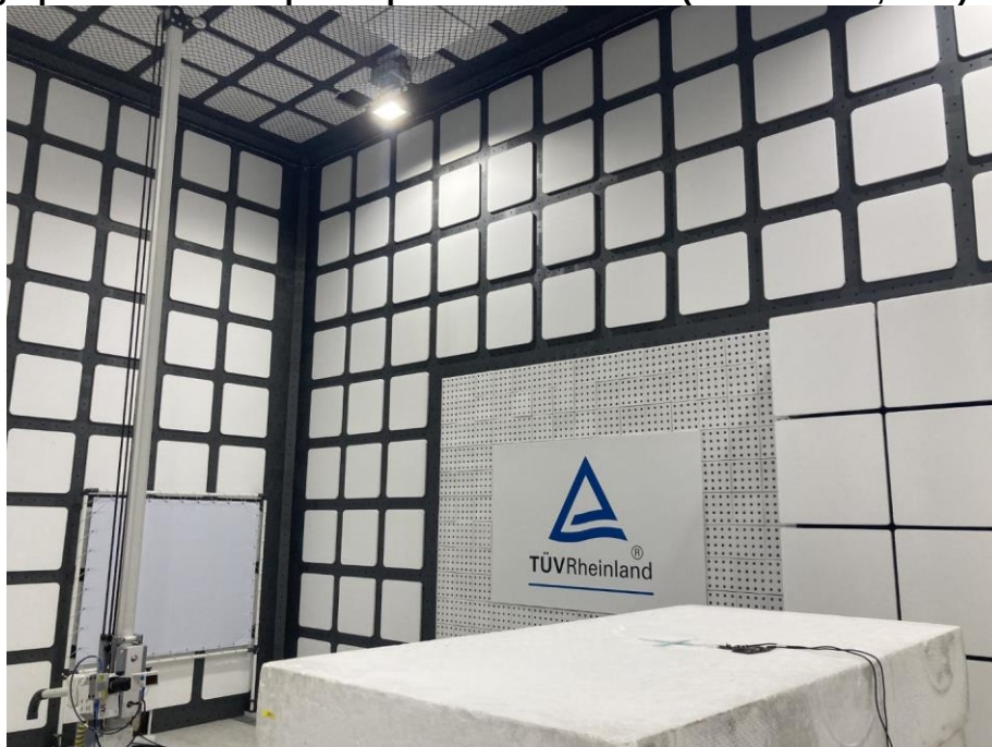
Photograph 38: Test Setup for Spurious Emissions (Back View 4, BLE)
