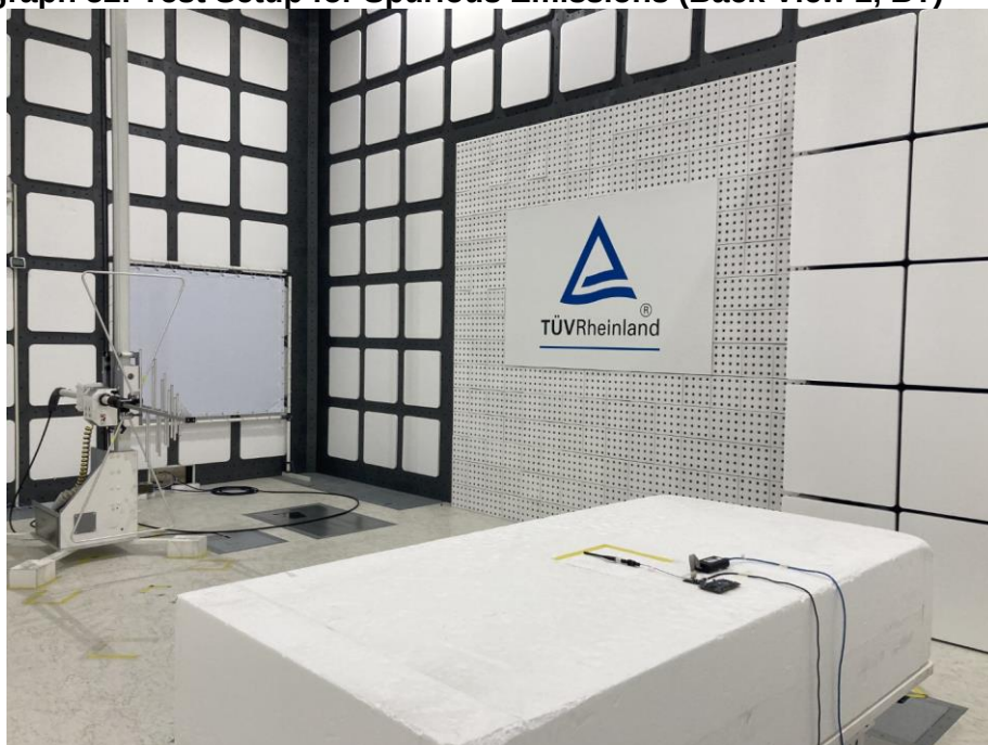
Photograph 52: Test Setup for Spurious Emissions (Back View 2, BT)
