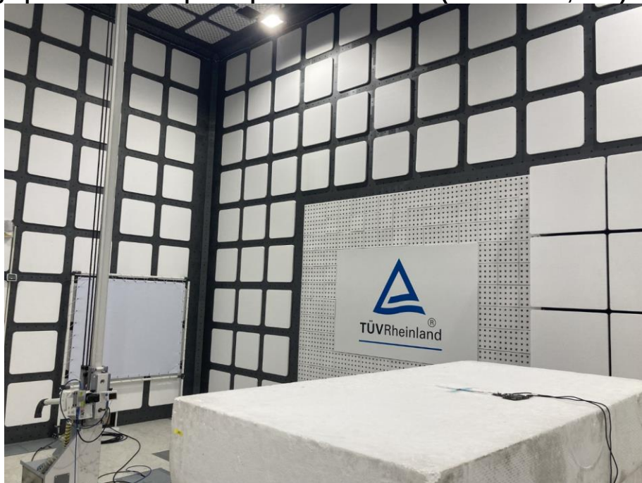
Photograph 14: Test Setup for Spurious Emissions (Back View 4, BLE)
