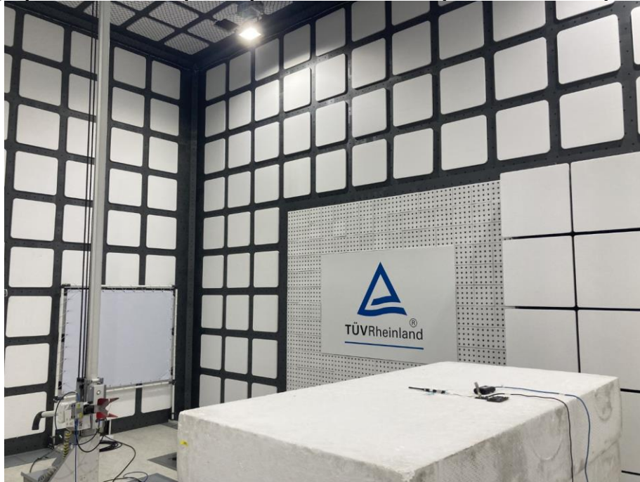
Photograph 53: Test Setup for Spurious Emissions (Back View 3, BT)
