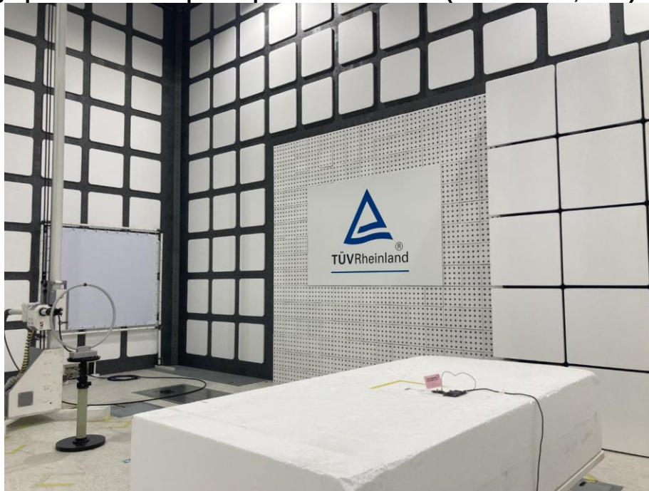
Photograph 44: Test Setup for Spurious Emissions (Back View 2, WiFi)
