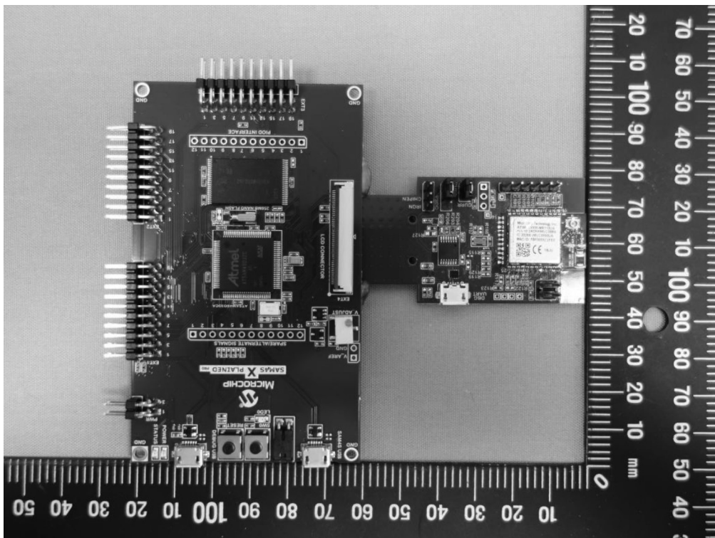
Module with test fixture
