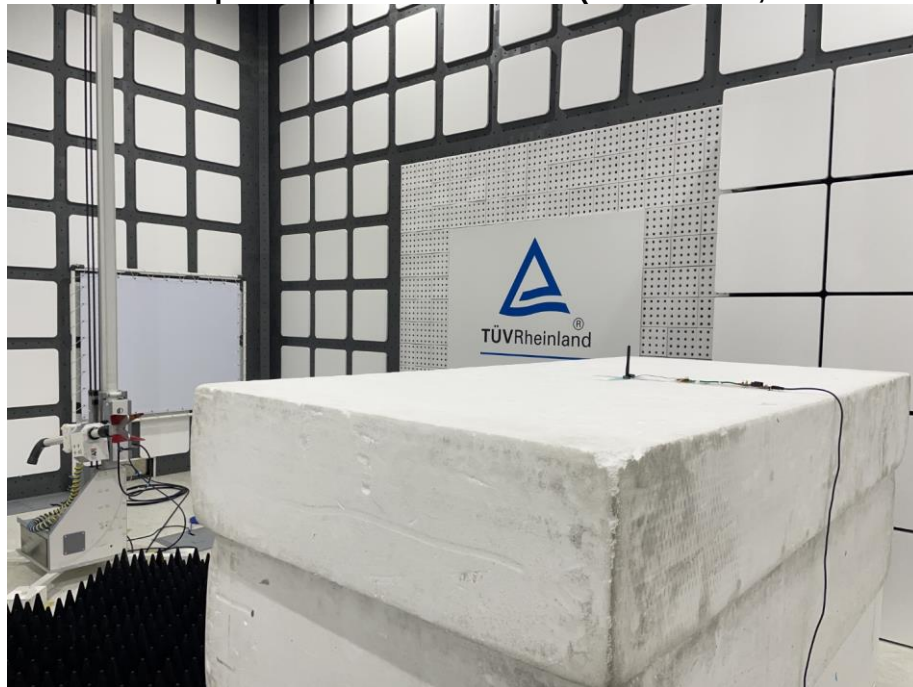
Photograph 18: Test Setup for Spurious Emissions (Back View 1, 2 nd Source)
