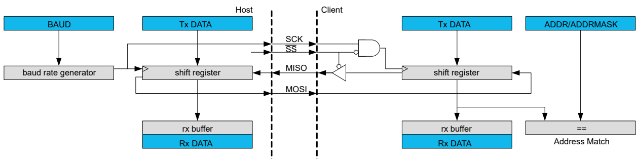
Figure 29-1. Full-Duplex SPI Host Client Interconnection
