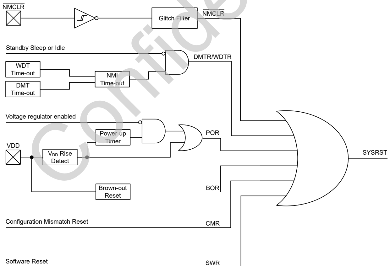
Figure 13-6. CRU-System Reset Block Diagram
