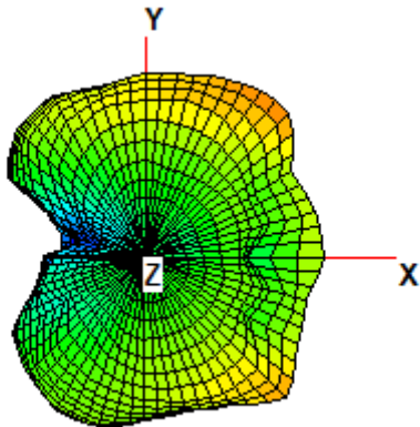
WBZ350 LGA with Ground Plane_3D_Passive
