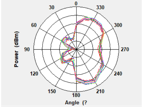
WBZ350 LGA_2D_YZ-Cut
