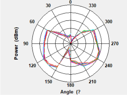
WBZ350 LGA with Ground Plane_2D_XZ-Cut
