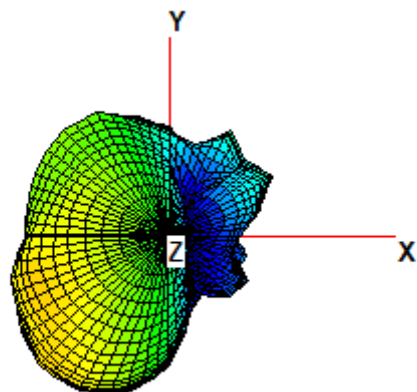
WBZ350 LGA_2D_XY-Cut
