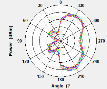
WBZ350 LGA with Ground Plane_2D_YZ-Cut
