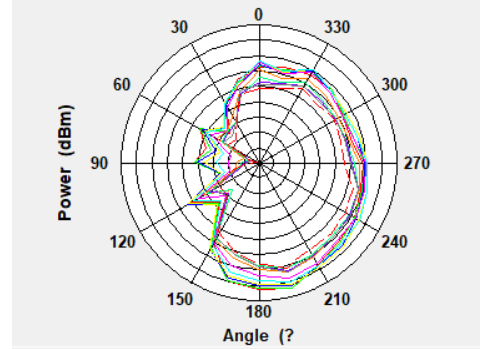
WBZ350 LGA_2D_YZ-Cut
