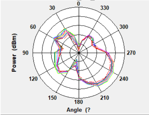
WBZ350 LGA_2D_XZ-Cut
