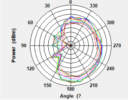
WBZ350 LGA with Ground Plane_2D_YZ-Cut
