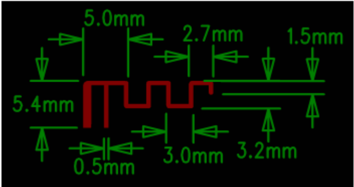
Antenna Photo & Length(mm)
