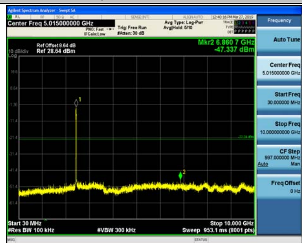
Spurious emission
