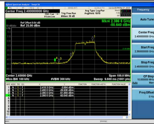
Spurious emission
