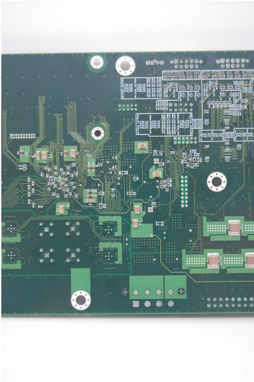
Closeup Bottom View2
