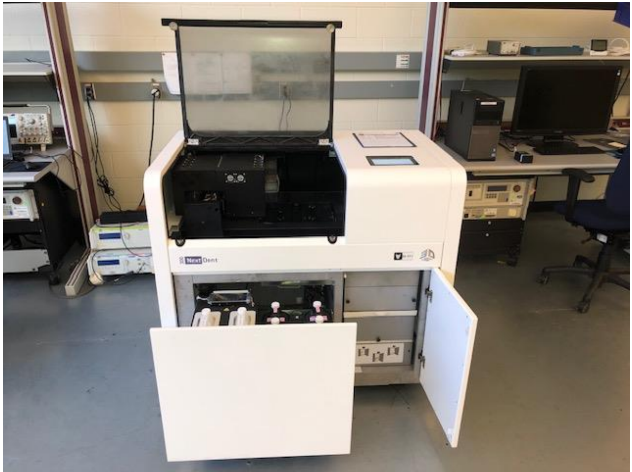
Front view of NextDent 300 Printer with doors open
