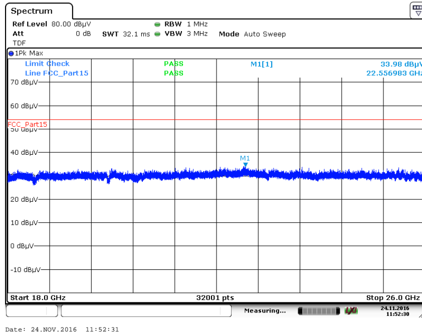
Plot 3: 18 GHz to 26 GHz, TX mode, channel 00, vertical & horizontal polarization
