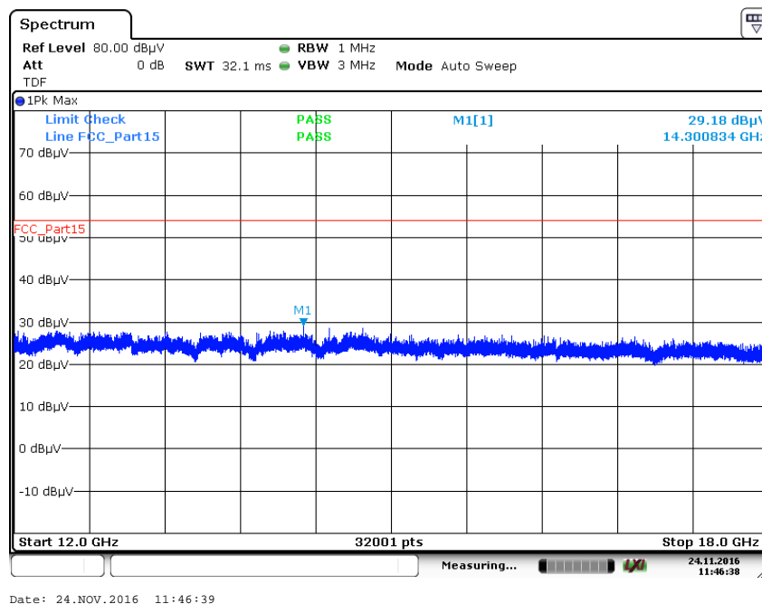
Plot 2: 12 GHz to 18 GHz, TX mode, channel 00, vertical & horizontal polarization
