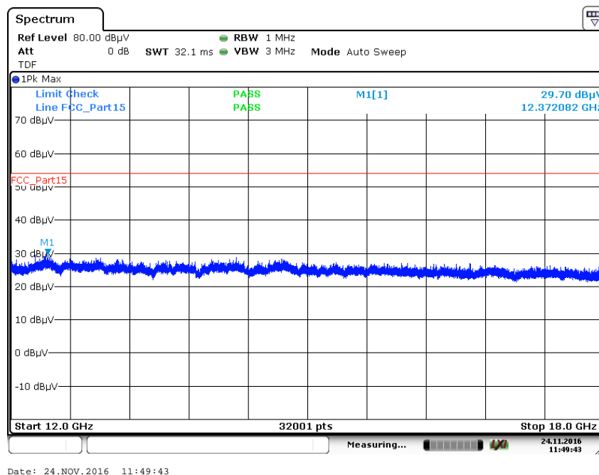
Plot 5: 12 GHz to 18 GHz, TX mode, channel 19, vertical & horizontal polarization
