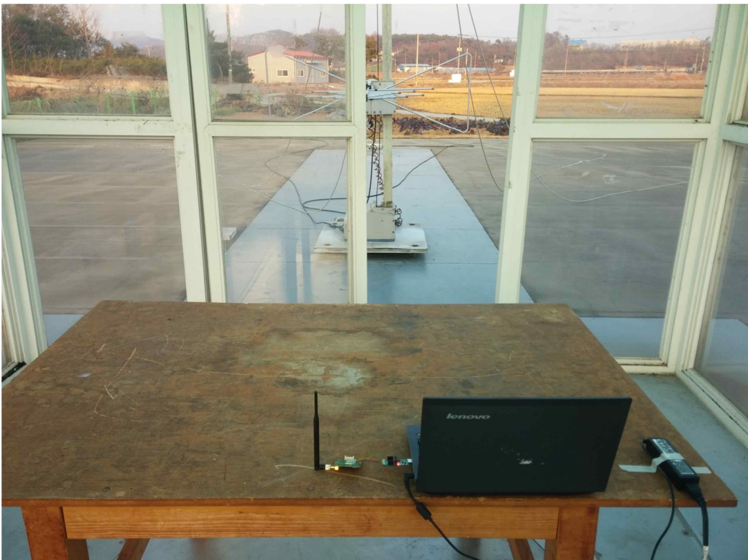
Radiated emission Test (below 1 000 MHz)
