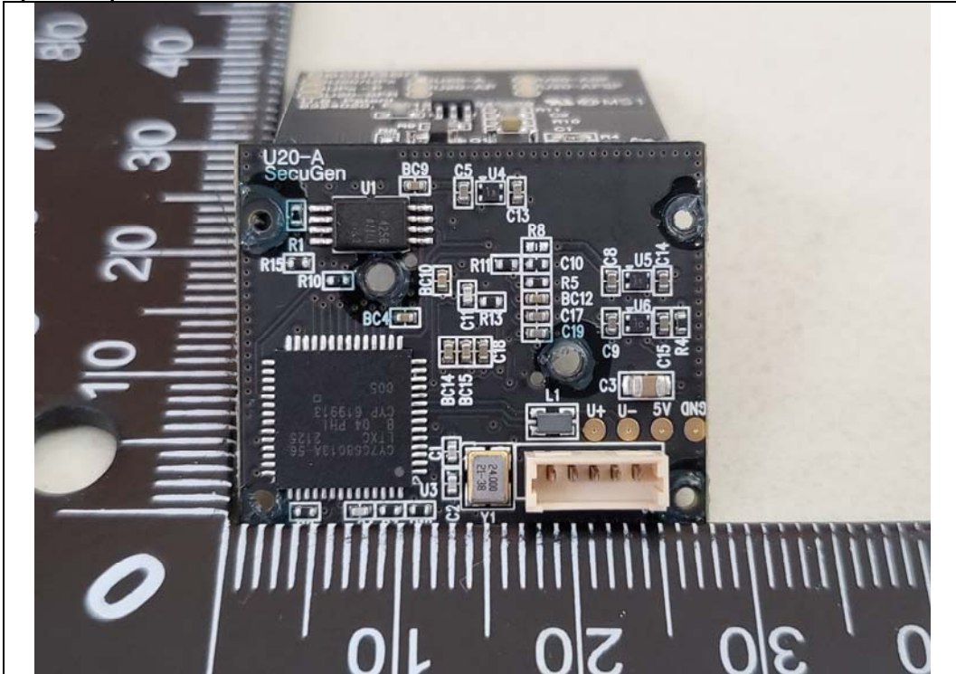
(U20-A)CMOS Sensor Board Front
