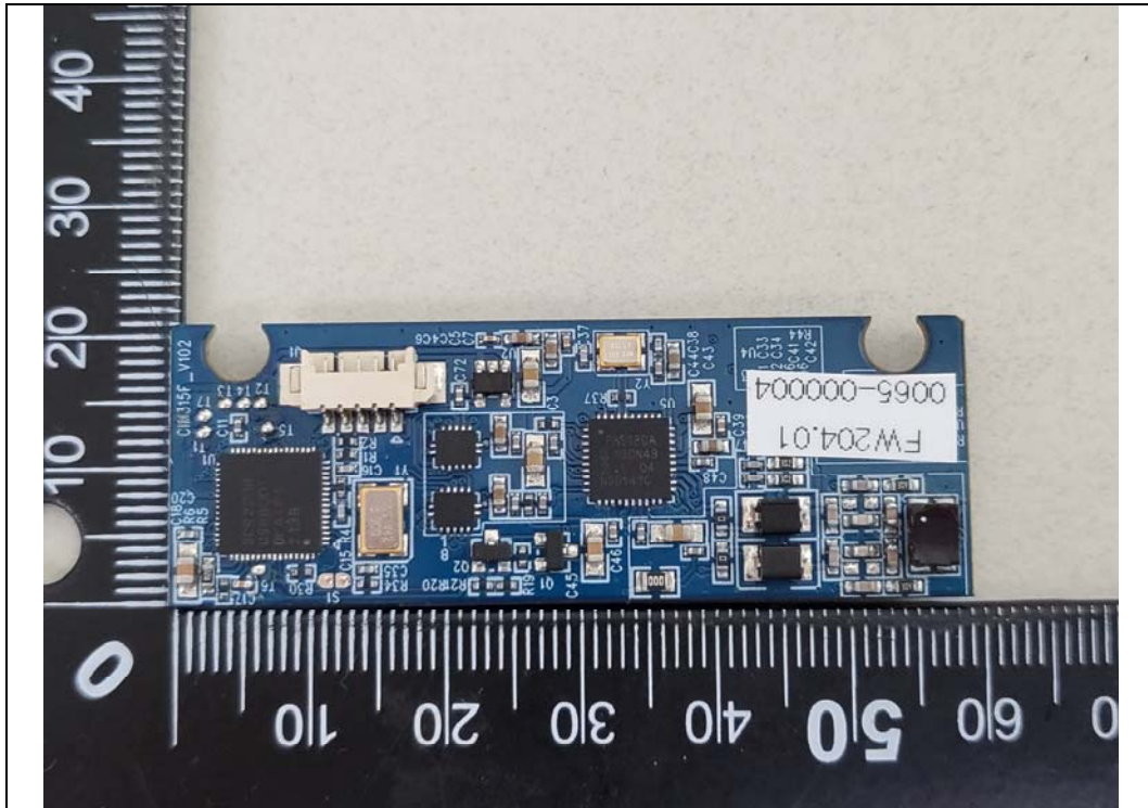
RF Card Reader Board Front
