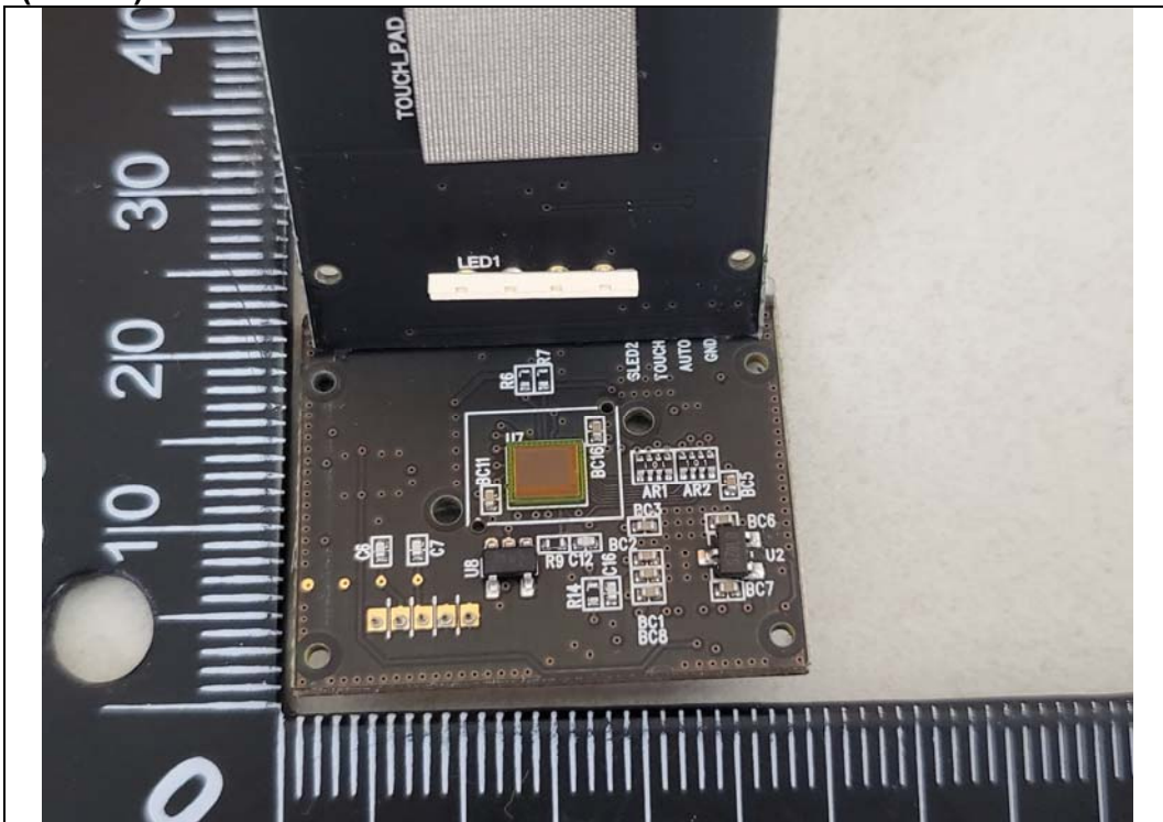
(U20-A)CMOS Sensor Board Rear
