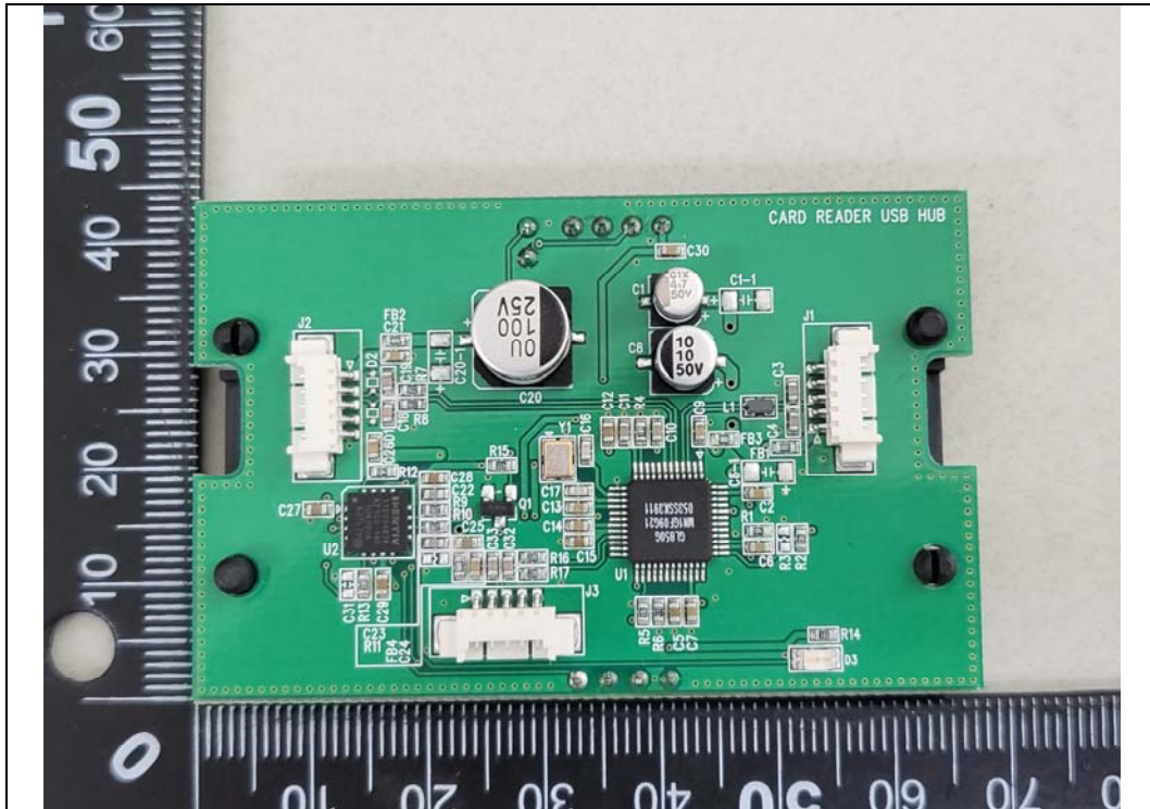
Contact Card Reader Board Front
