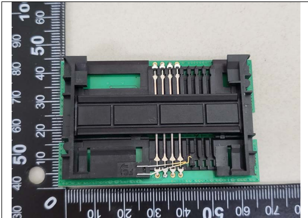
Contact Card Reader Board Rear
