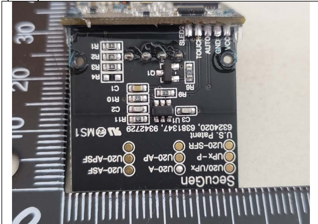
(U20-A)LED Board Front
