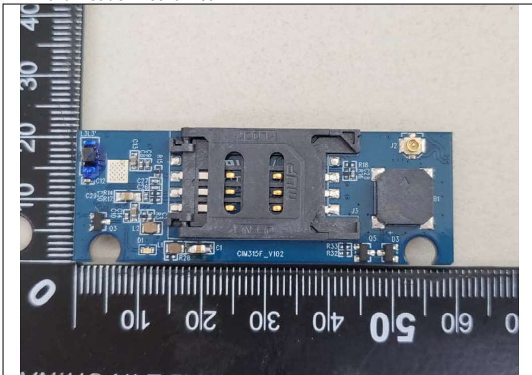
RF Card Reader Board Rear
