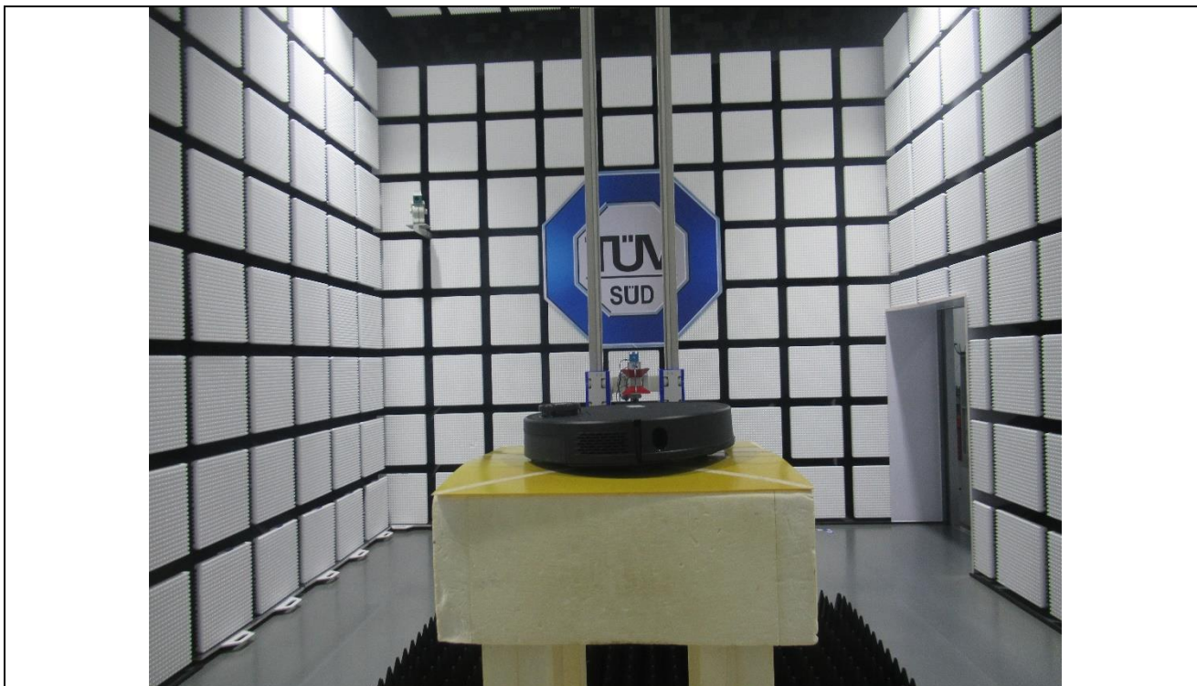
Radiated Emission test (1000MHz to 18000MHz)
