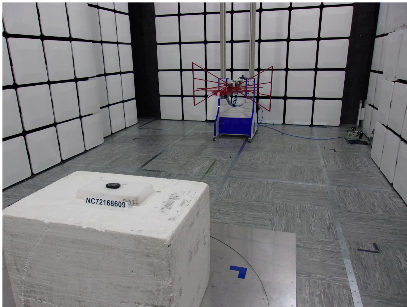
Photo 1.4-1 – Unintentional Emissions 30-1000 MHz
