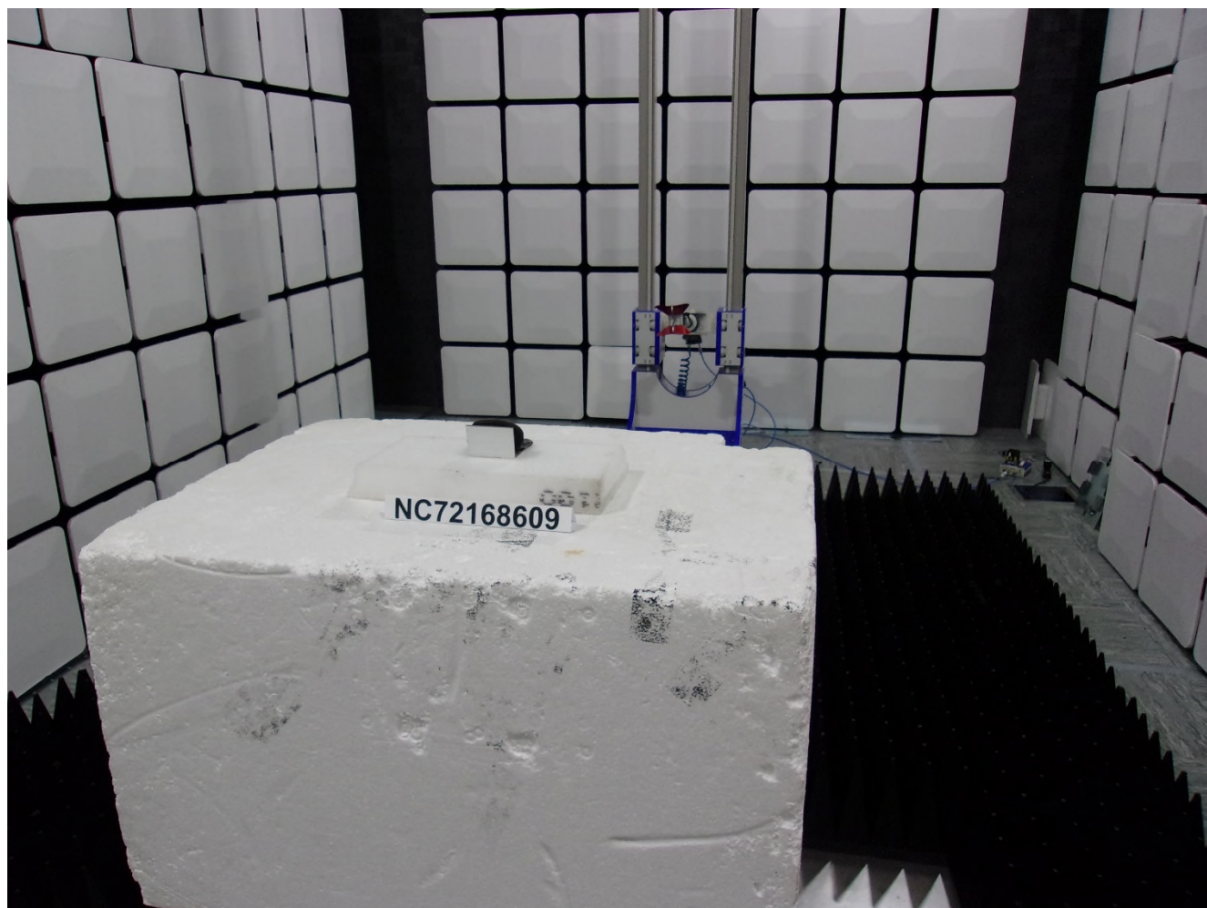
Photo 1.3-3 – RE Spurious Emissions 1-18 GHz
