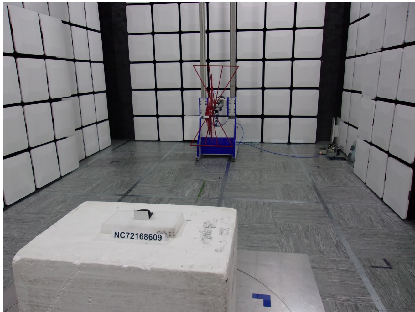
Photo 1.3-2 – RE Spurious Emissions 30-1000 MHz
