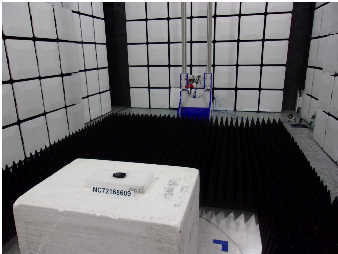
Photo 1.4-2 – Unintentional Emissions 1-18 GHz
