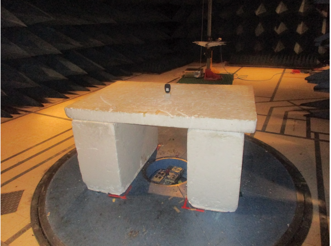
Figure 10: Radiated Emissions – Back View - 200 MHz - 1 GHz - EUT Standing
