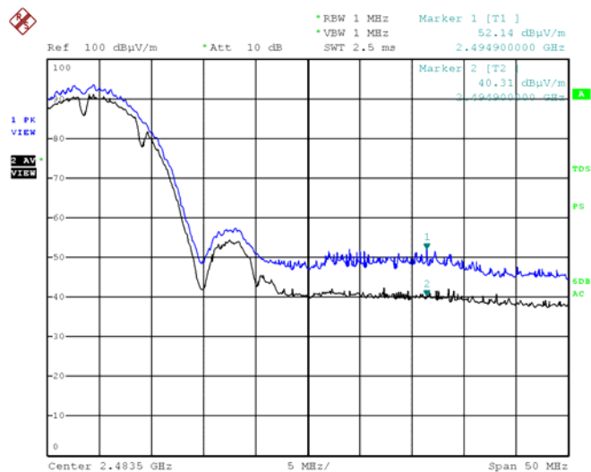
802.11b High (Horizontal)
