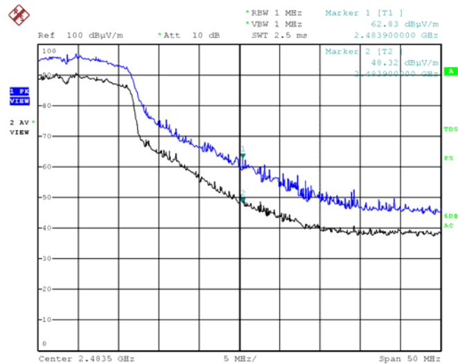
802.11g High (Horizontal)
