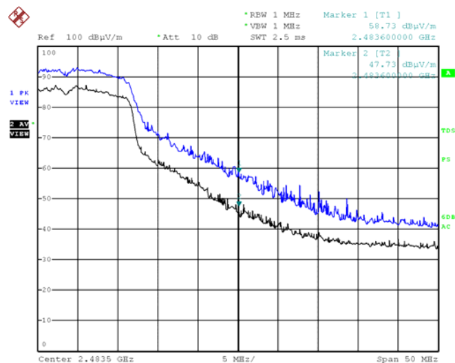
802.11g High (Vertical)
