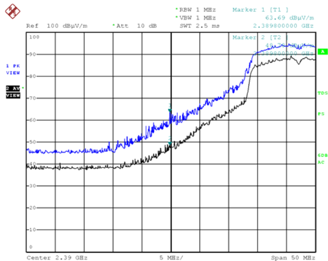
802.11g Low (Horizontal)
