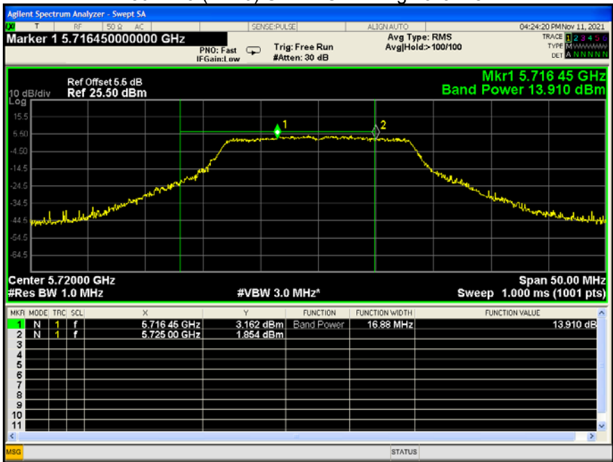
802.11a (HT20) U-NII-2C 144 High channel
