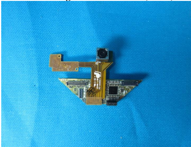
FIGURE 75: Bottom Board Full assembled (Front)
