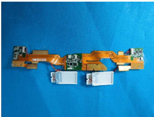
FIGURE 77: Middle Board (Front) Middle Board (Rear)
