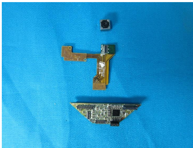
FIGURE 76: Bottom Board in parts (Front) Bottom Board in parts (Rear)
