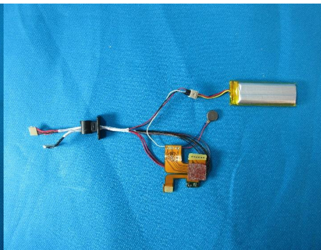
Left Temple (Rear)
