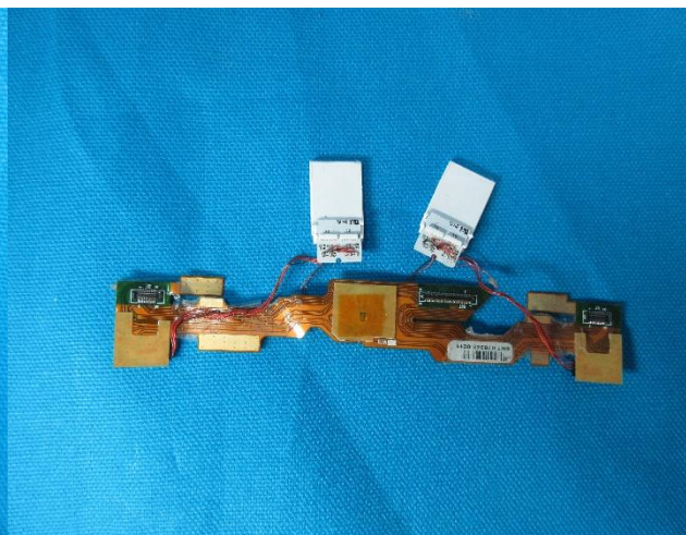
FIGURE 77: Middle Board (Front) Middle Board (Rear)
