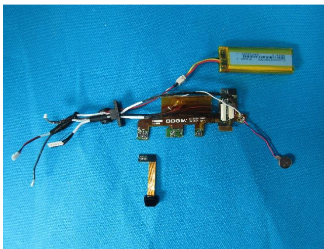
FIGURE 80: Right Temple (Front)
