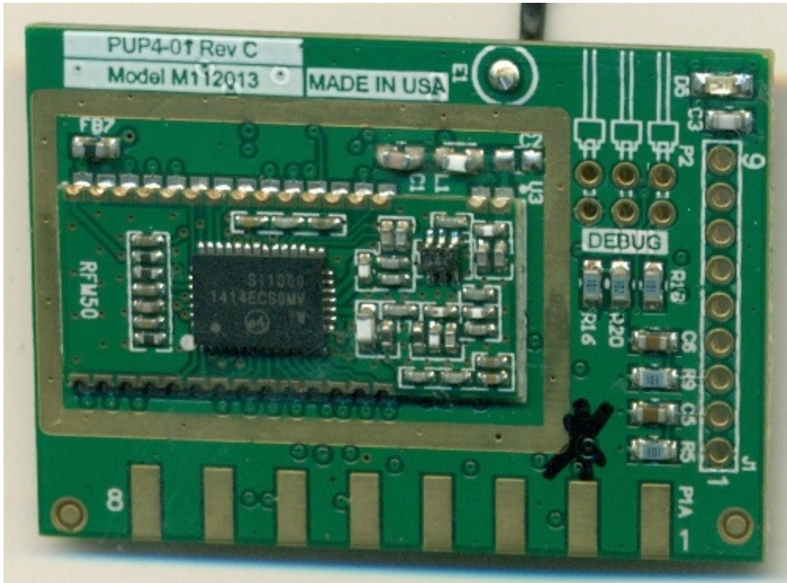
Photo 5 – Top View of the Radio Board with the Shield Removed
