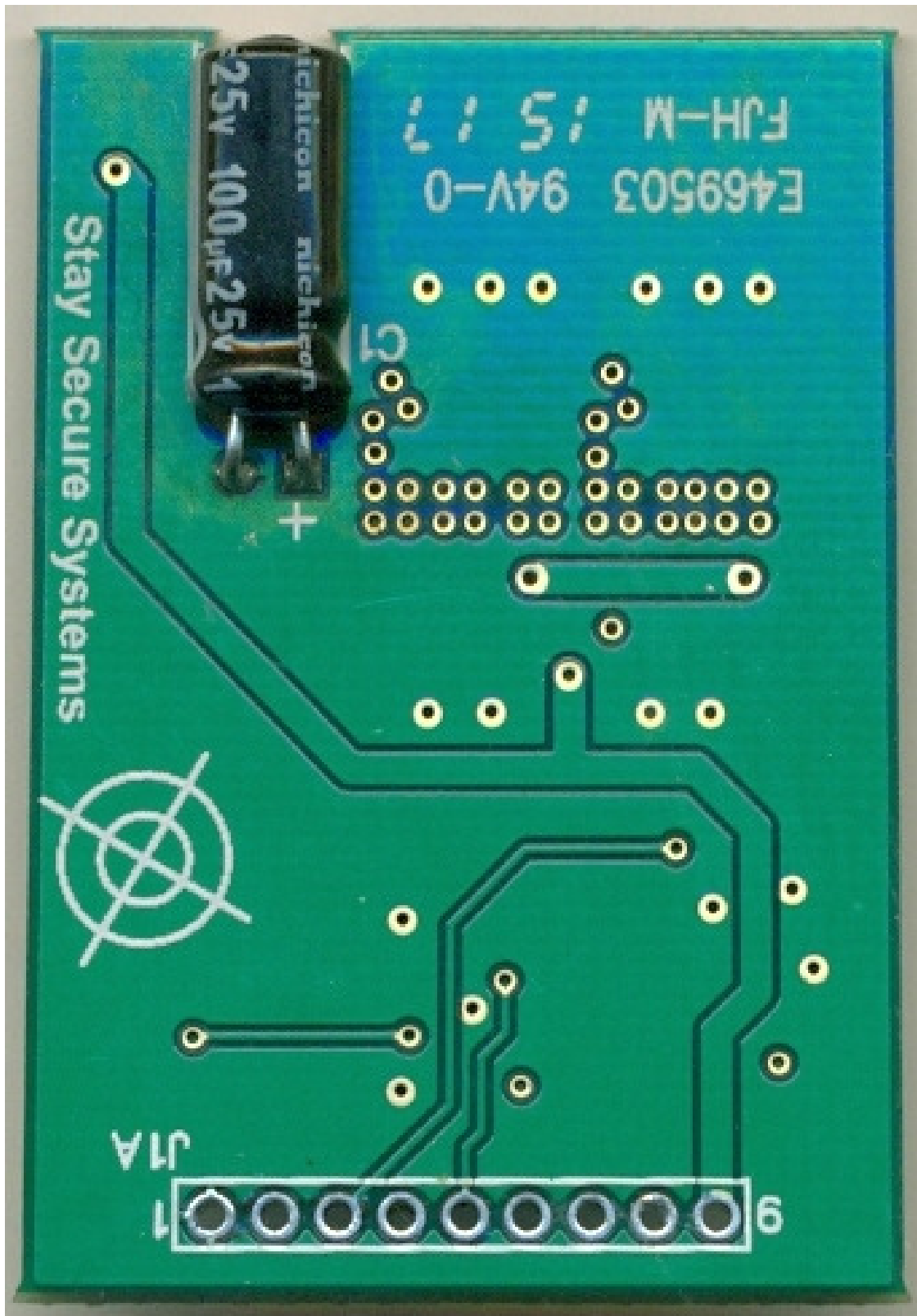
Photo 2 – Bottom Side View of the Power/Interface Board
