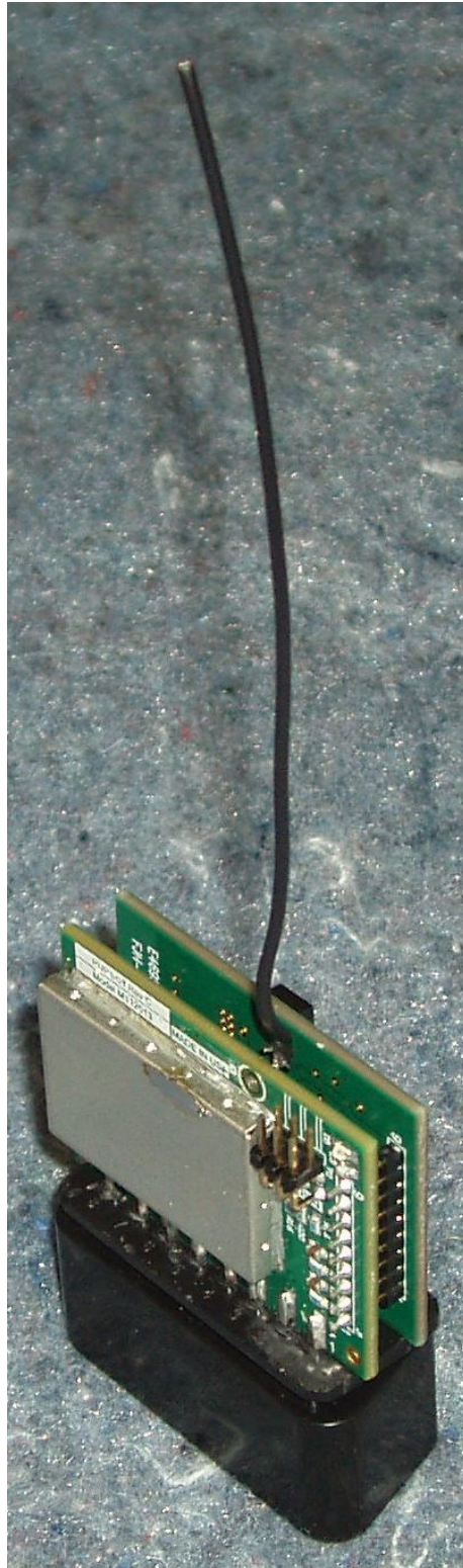
Photo 4 – Internal View with the Cover Removed
