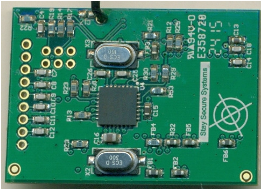
Photo 6 – Bottom View of the Radio Board
