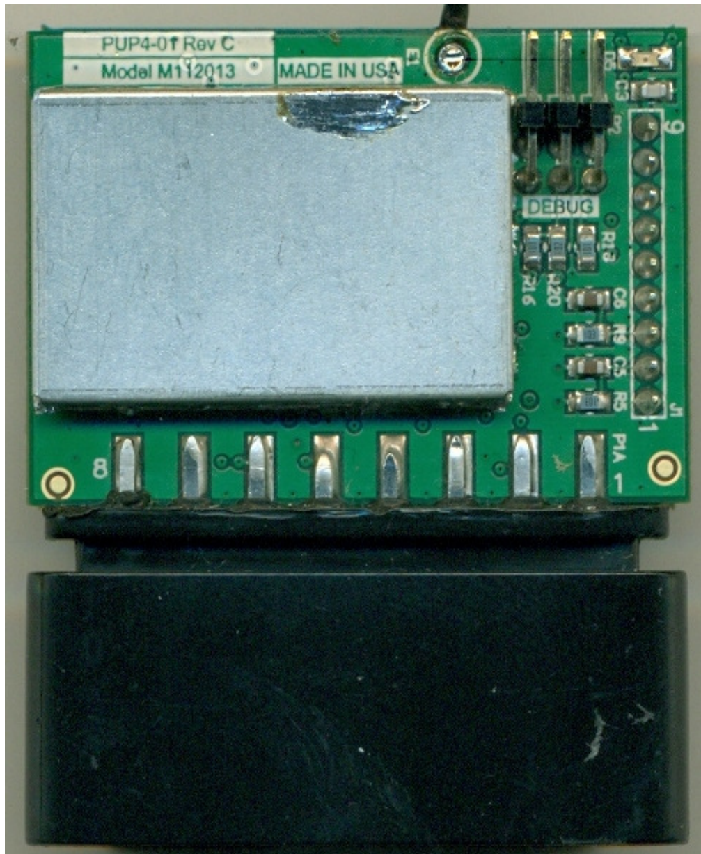
Photo 3 – Top Side View of the Radio Board with Shield On
