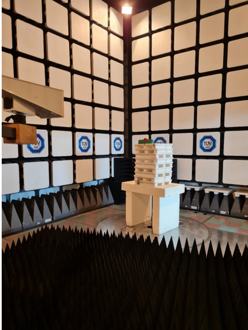
Figure 5 – Radiated Emissions Setup
