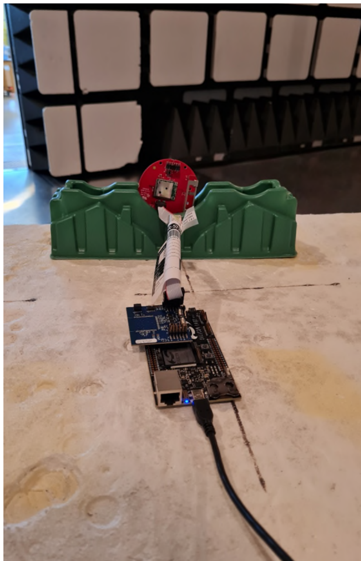
Figure 1 – Radiated Emissions Setup
