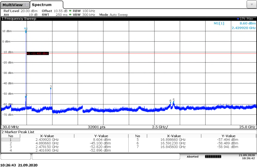
Figure 7.5.1.2-2: 30 MHz – 25 GHz – MCH
