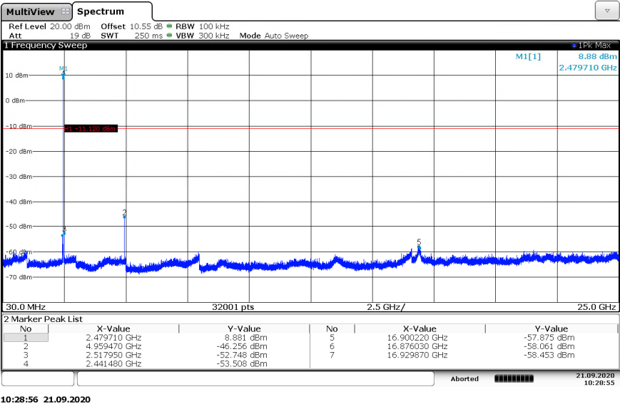
Figure 7.5.1.2-3: 30 MHz – 25 GHz – HCH
