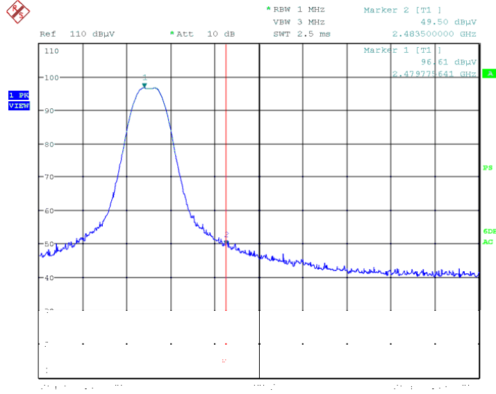
Figure 7.5.2.5-15: Emission Profile – High Channel Band Edge – Surface Mount
