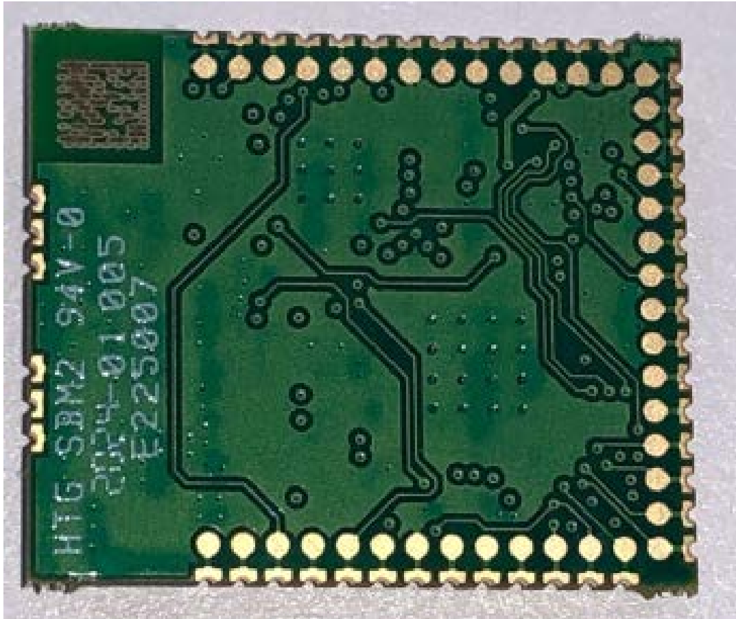
Figure 2: Back View
