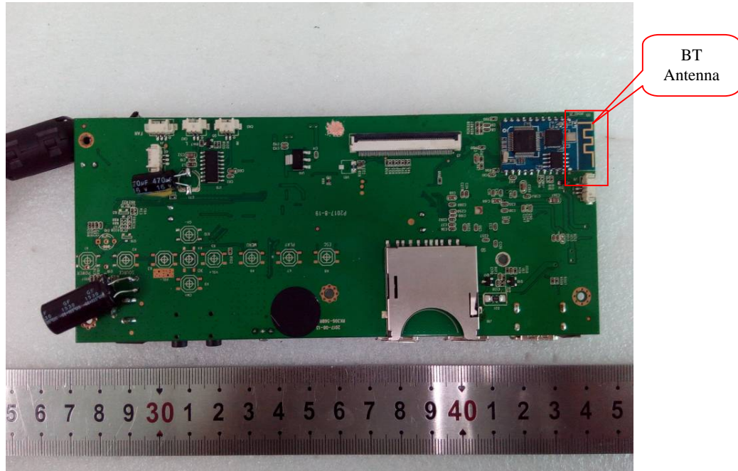
EUT – Mainboard Bottom Cover off View
