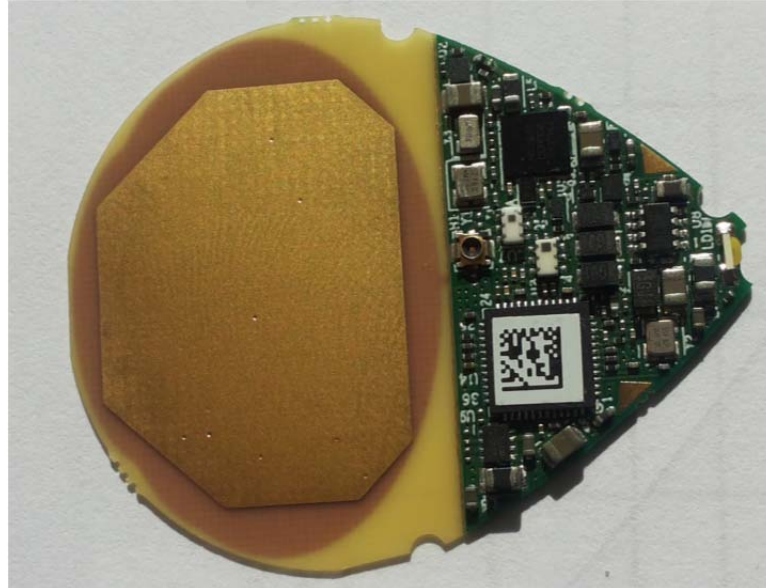
Photograph 7.6.1 Antenna assembly
