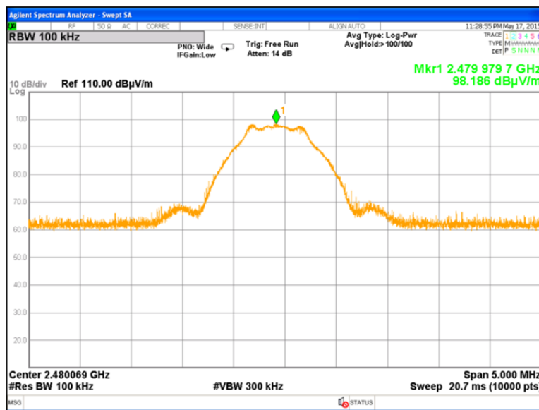
Plot 7.5.3 Peak spectral power density at high frequency zoomed at the peak
