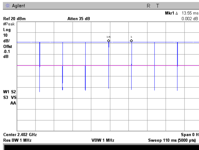
Plot 7.3.20 Transmission pulse period
