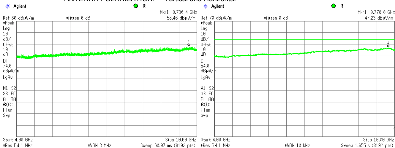
Plot 7.3.11 Radiated emission measurements from 4000 to 10000 MHz at the mid carrier frequency
