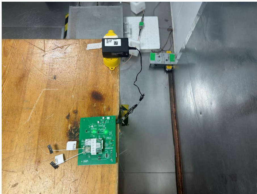
Test Photo 6-FPC Antenna
