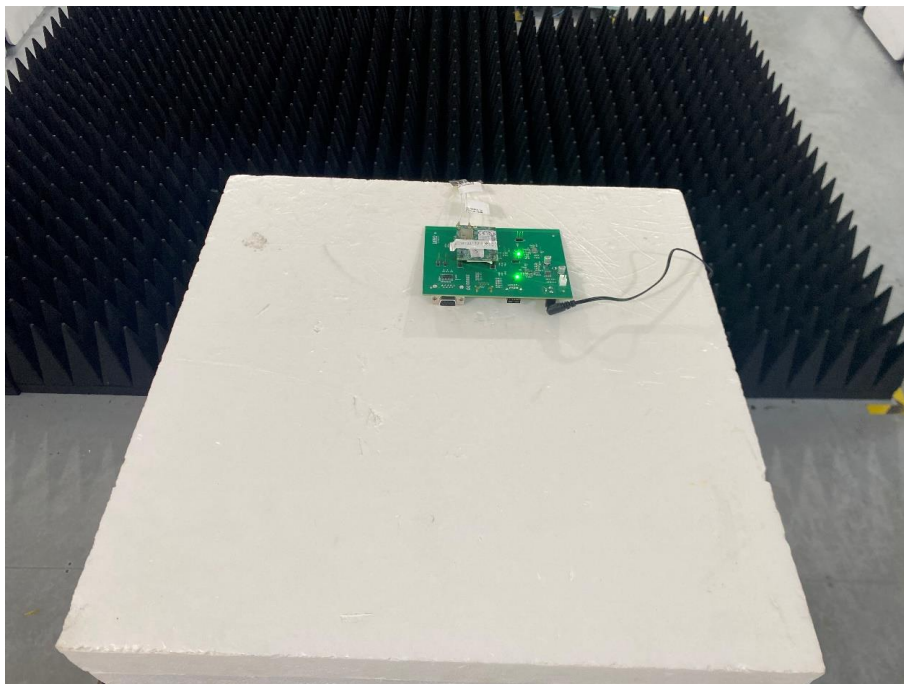
Close-up-FPC Antenna
