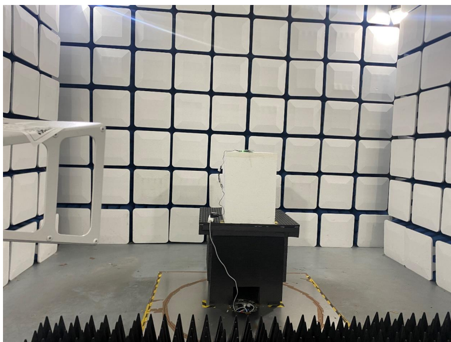
Above 1GHz-PCB Antenna
