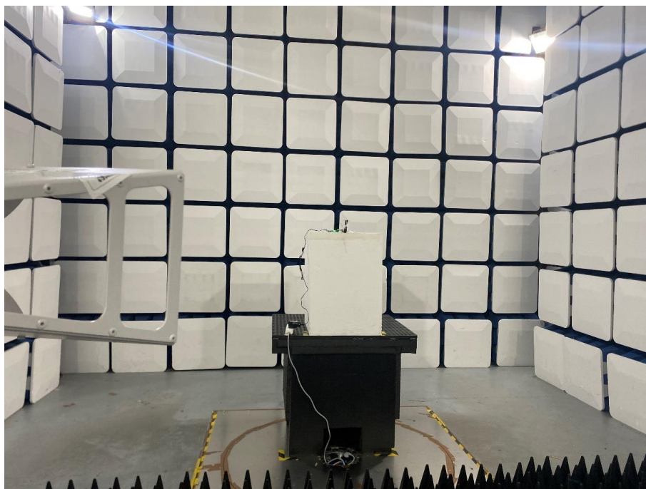
Above 1GHz-Rod Antenna
