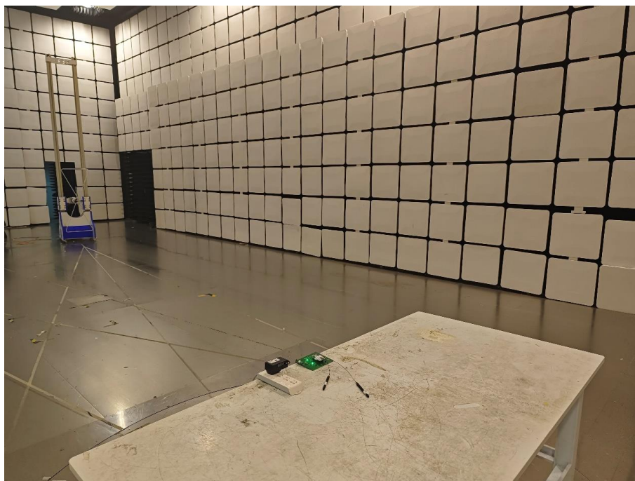
30MHz-1GHz-Rod Antenna
