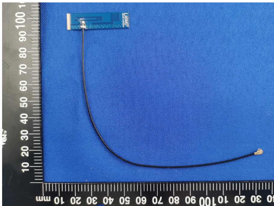
PCB Antenna (Model: LSANT-1C-180)
