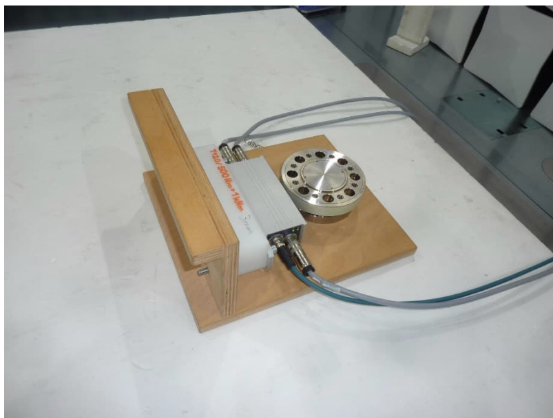
Test setup semi anechoic chamber (position 2)
