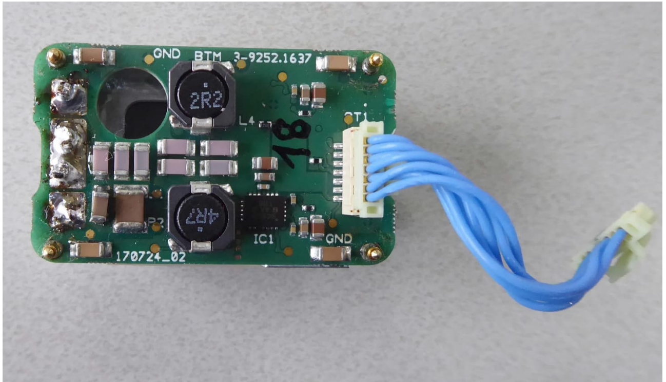
Power part (Coil Starter), bottom view
