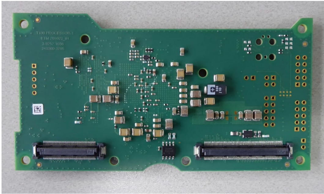
Processor PCB, bottom view
