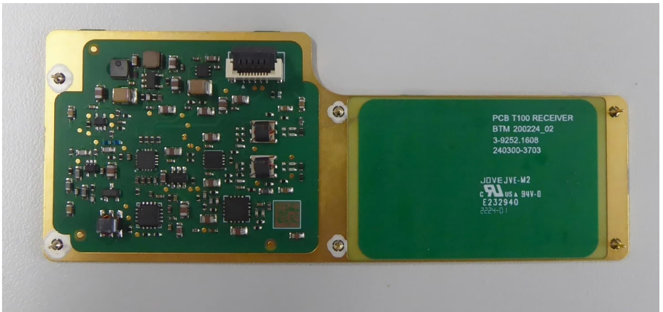
Receiver PCB, bottom view
