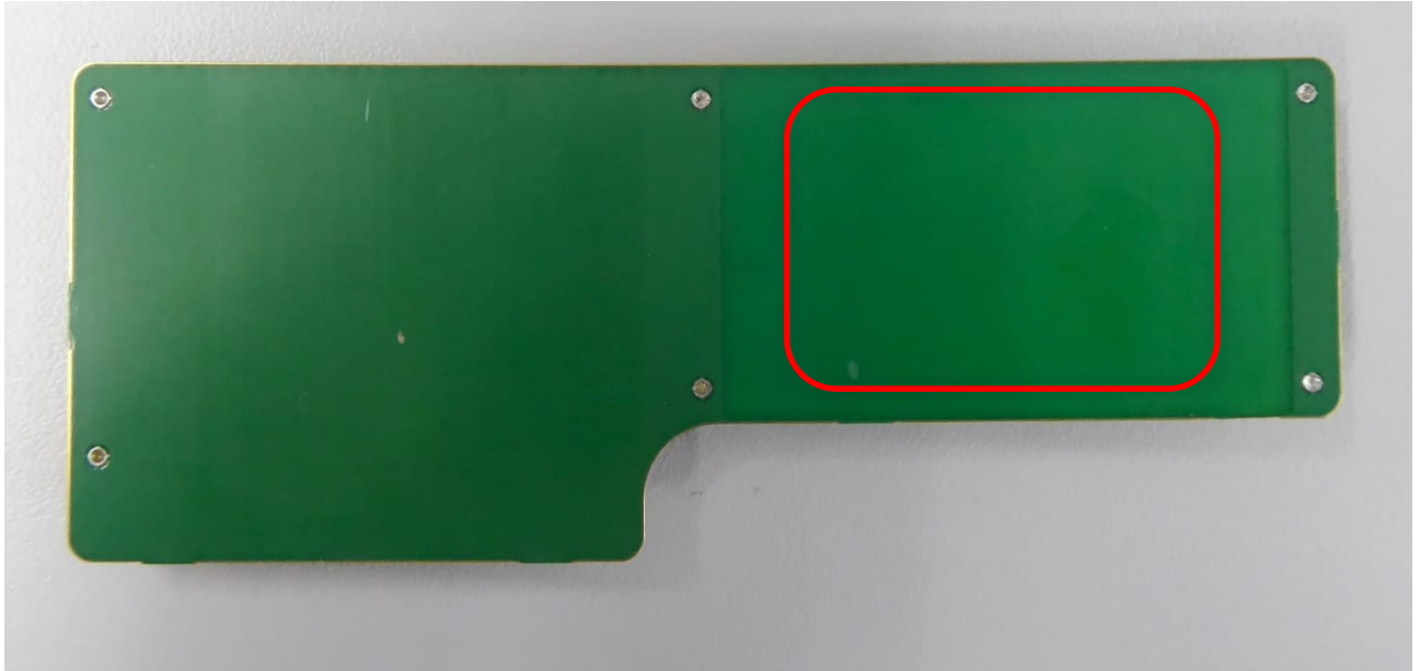
Receiver PCB, top view, antenna highlighted
