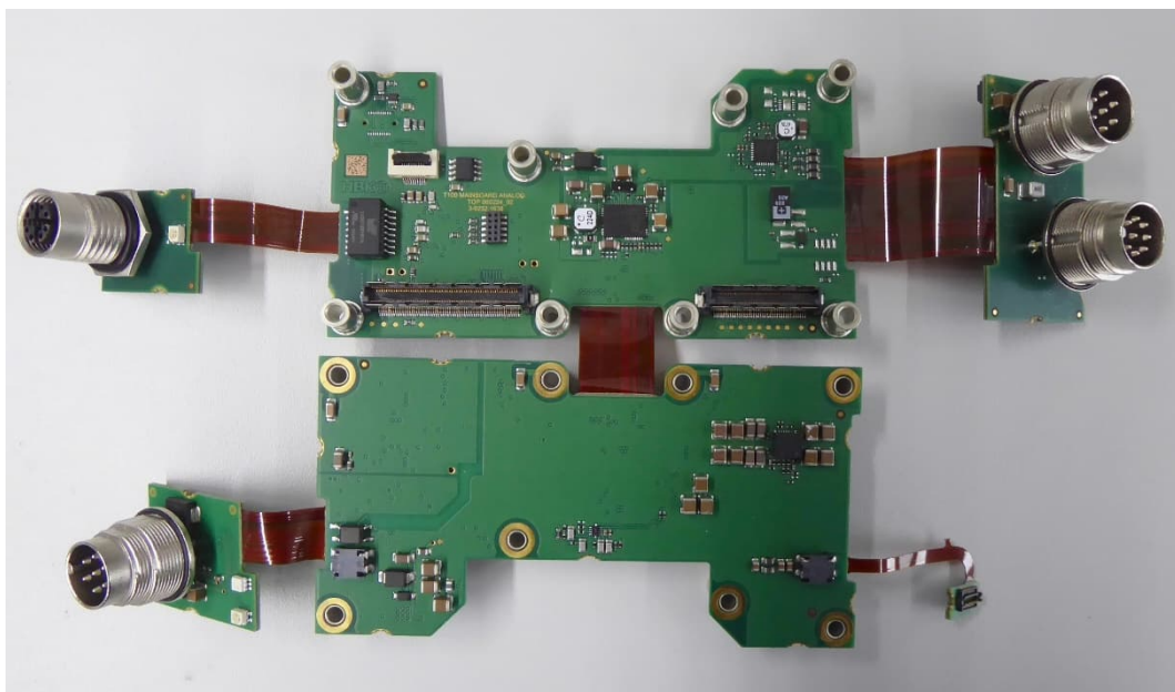
Analog PCB, top view
