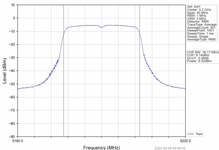
802.11n(HT20)_MCH_5200MHz_Ant1_NTNV
