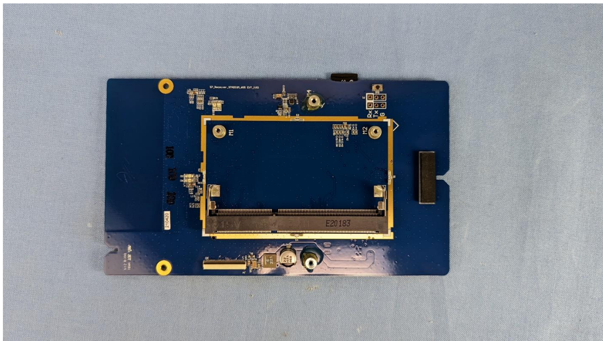
Main Board Top View Wireless Module Removed
