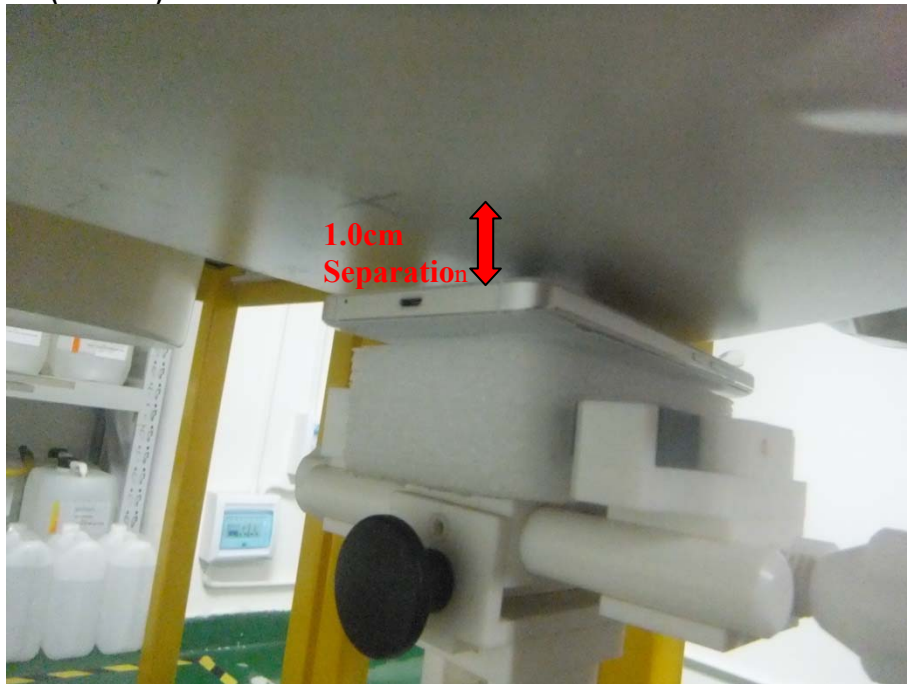
Body Setup Photo (LCD UP)
