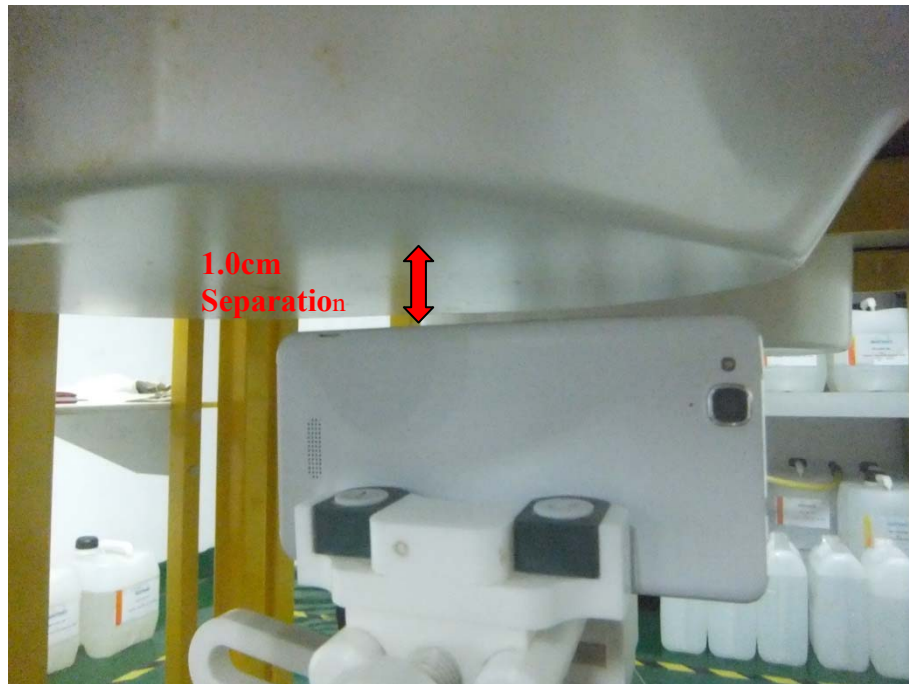
Body Setup Photo (RIGHT EDGE)
