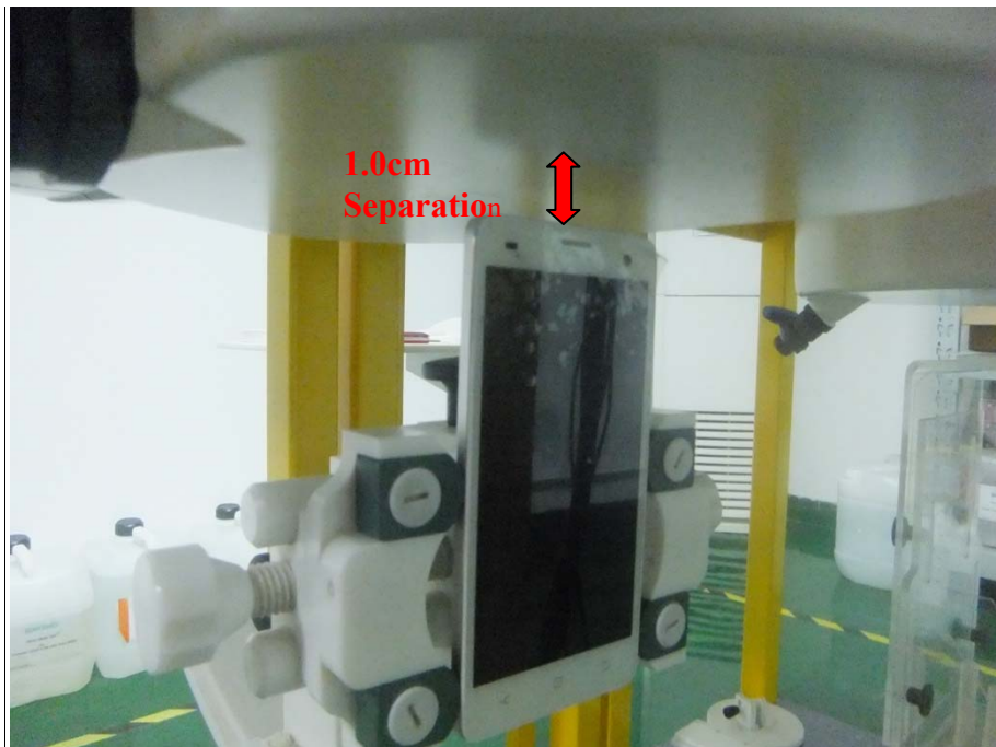
Body Setup Photo (Top EDGE)
