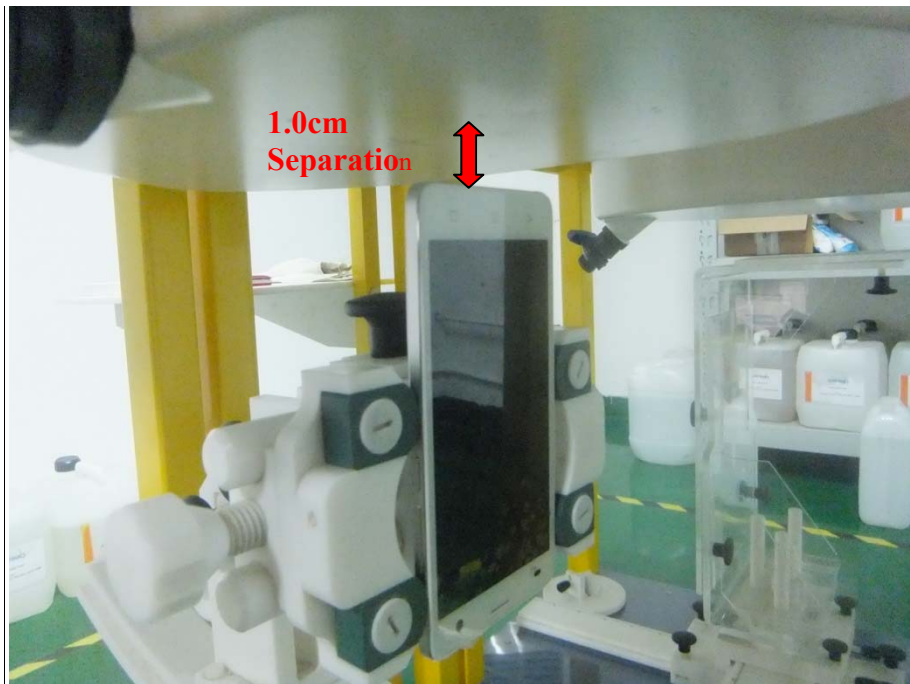
Body Setup Photo (BOTTOM EDGE)
