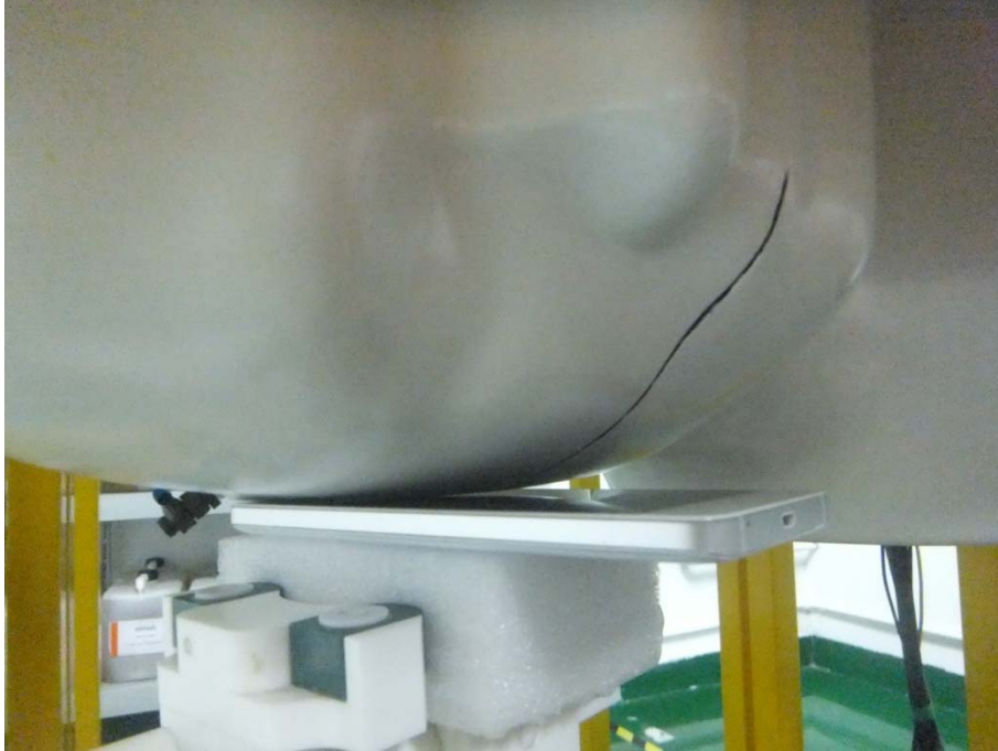
Right Head Touch View
