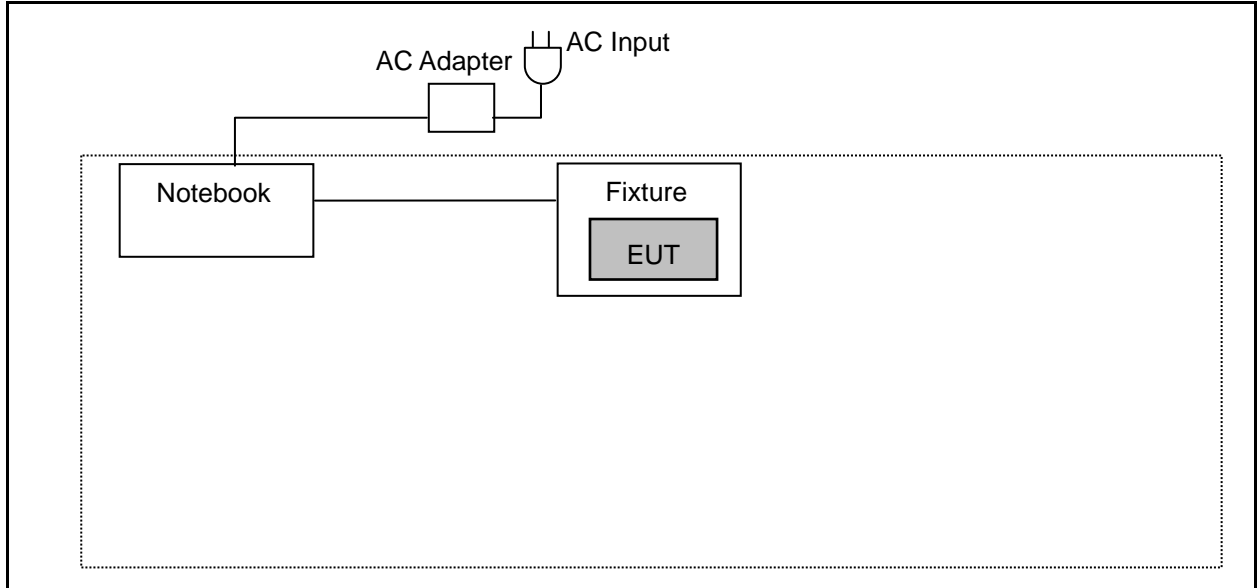
Radiated Emissions
