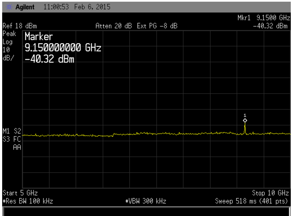
Figure 8. Antenna Conducted Emissions Mid, Part 3 GFSK Modulation
