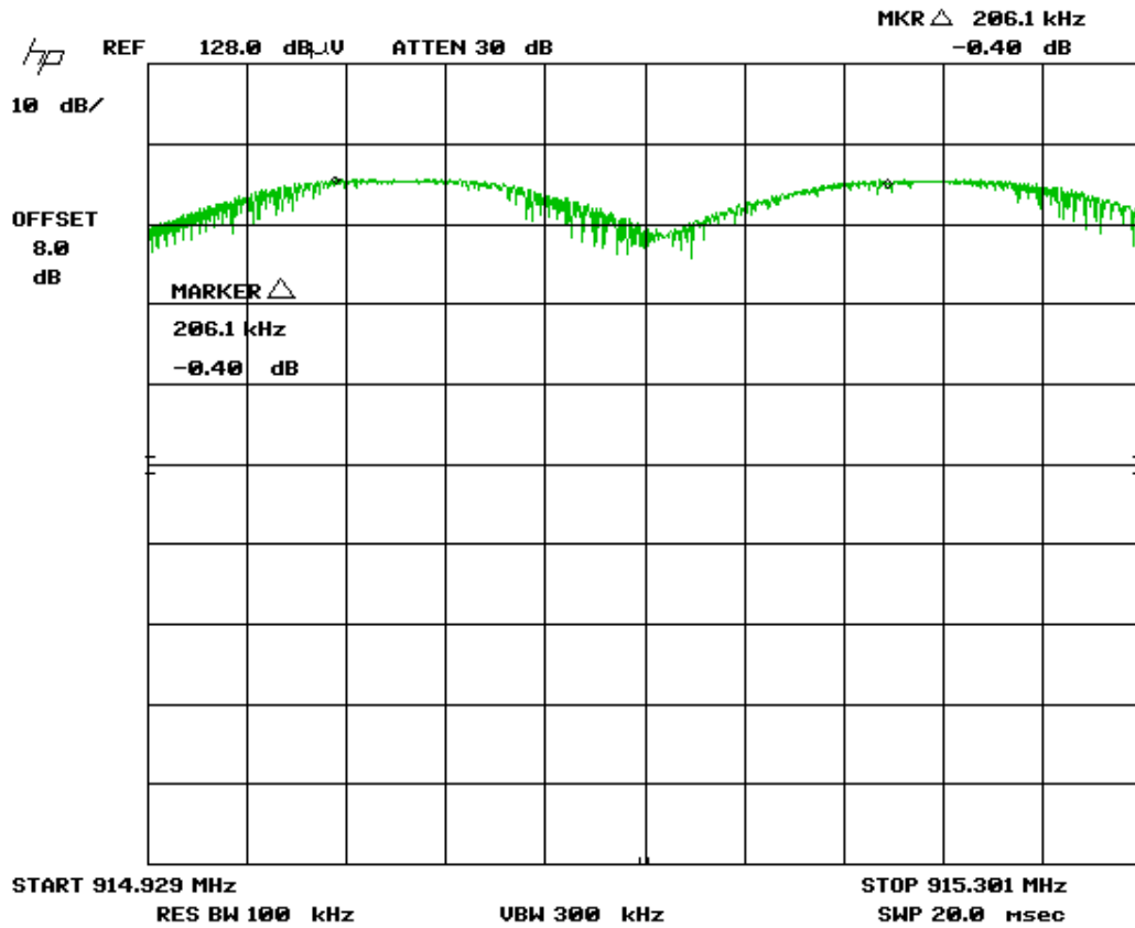
Figure 33. Channel Separation
