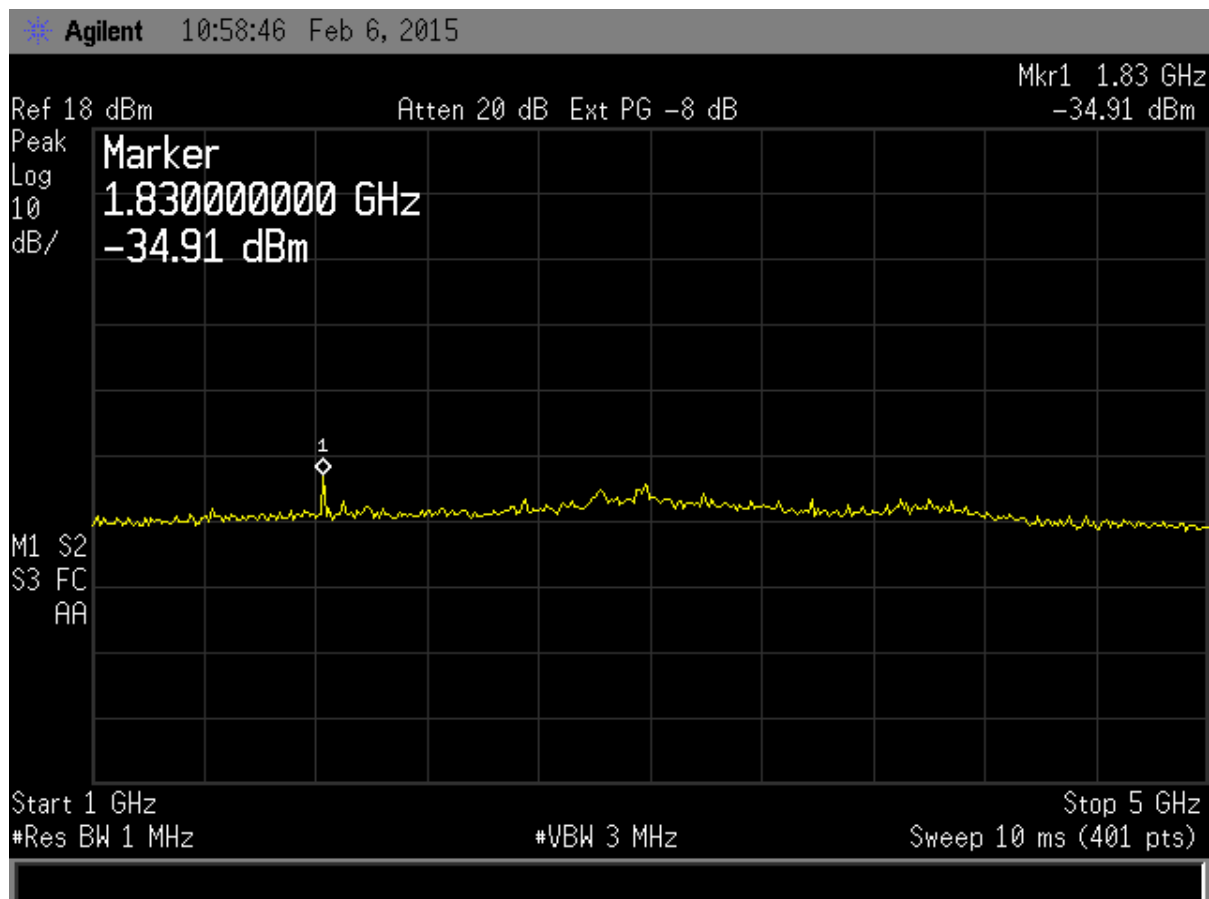
Figure 7. Antenna Conducted Emissions Mid, Part 2 GFSK modulation
