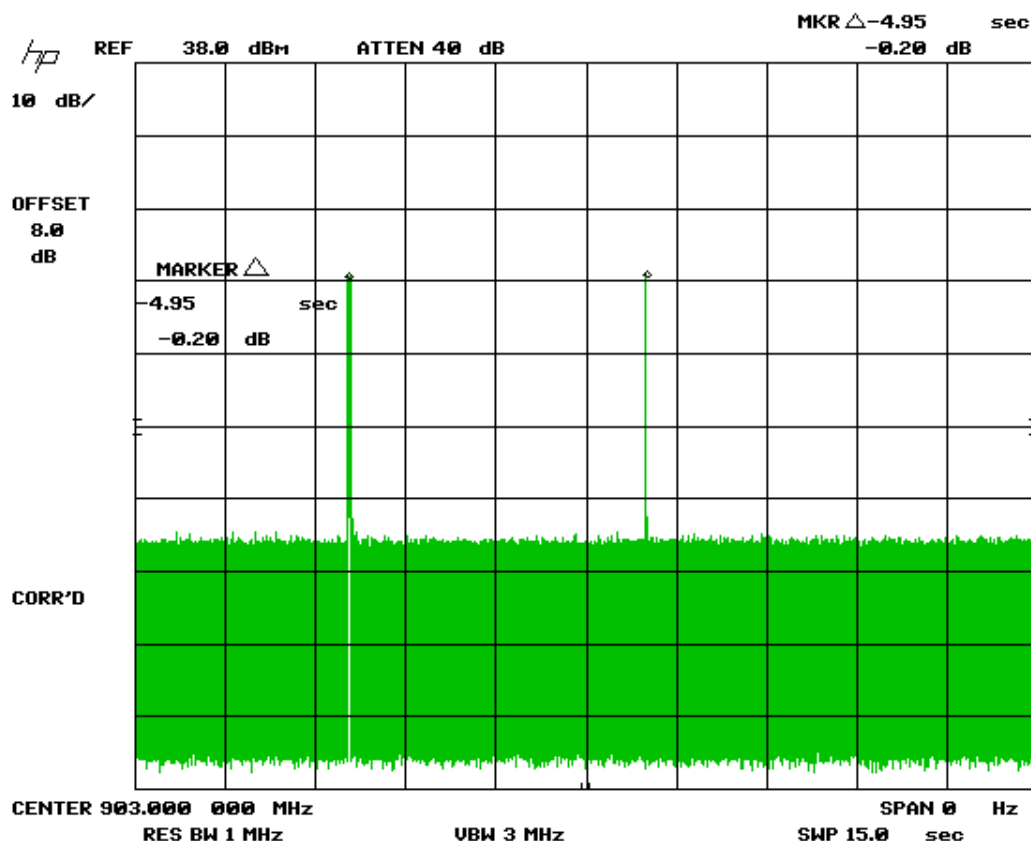
Figure 35. Time between Occupancy
