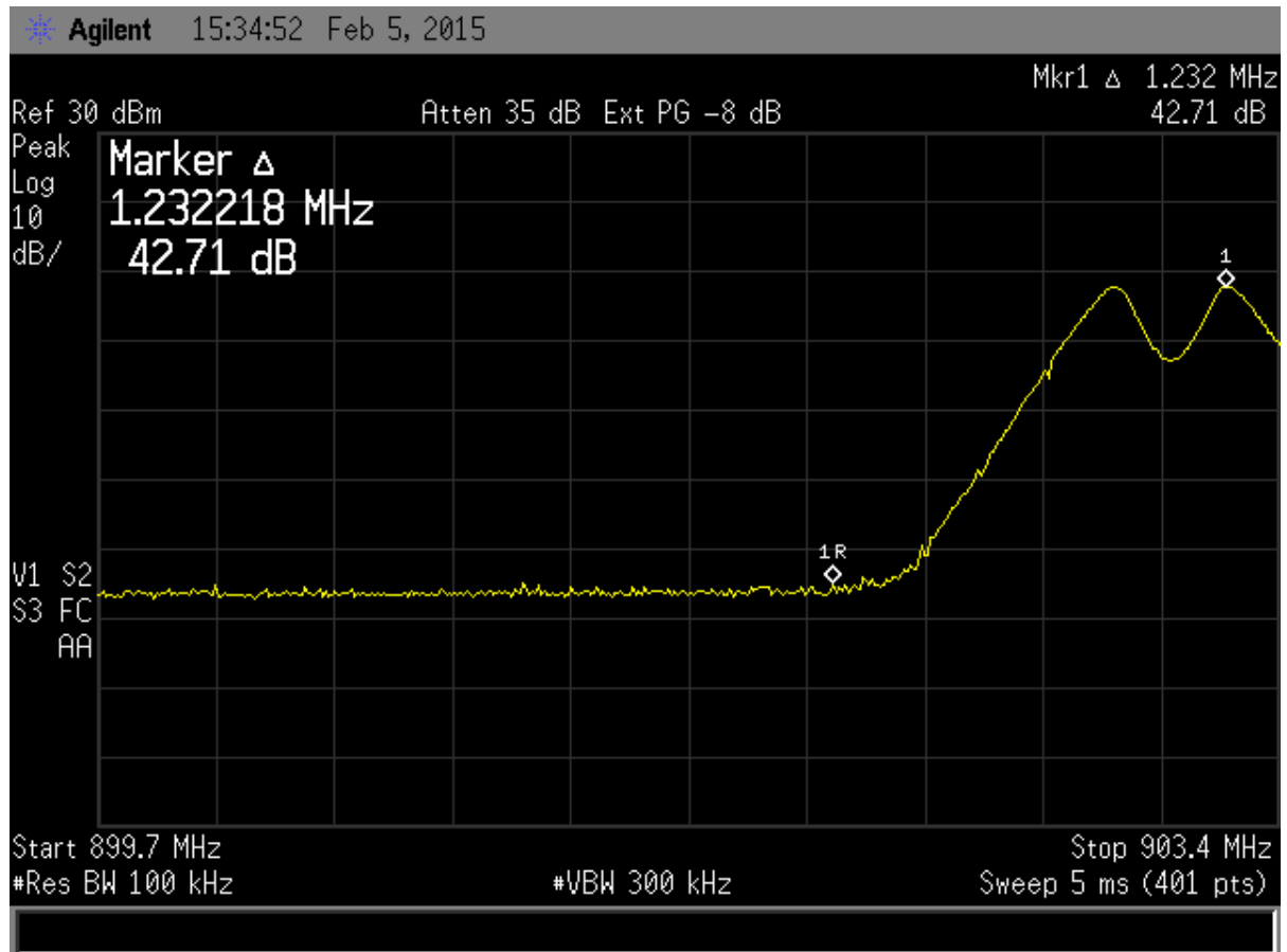
Figure 16. Band Edge Compliance, Low Channel Delta – Peak 2-FSK modulation
