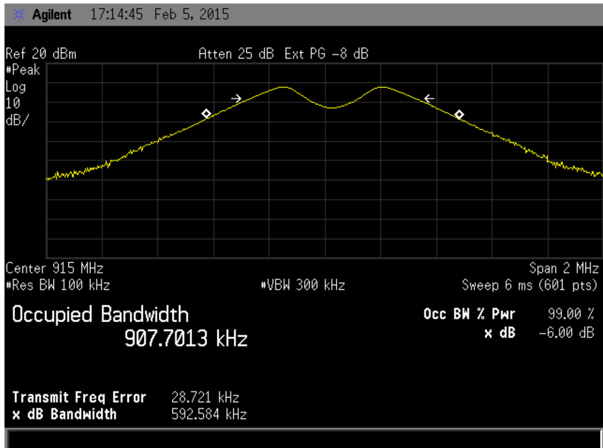
Figure 19. Six dB Bandwidth - 15.247 - Mid Channel
