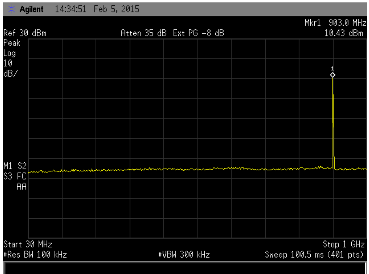
Figure 3. Antenna Conducted Emissions Low, Part 1 GFSK Modulation
