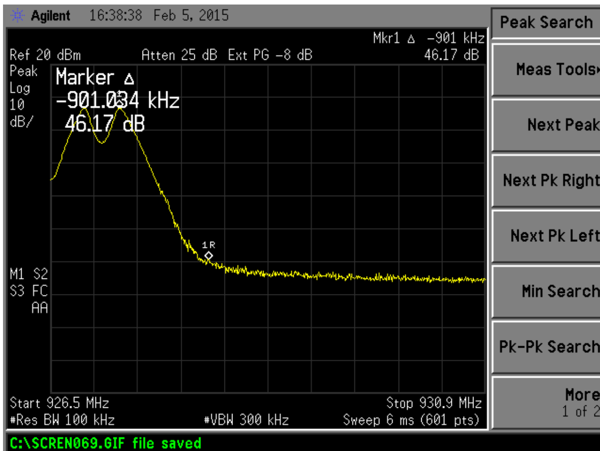
Figure 17. Band Edge Compliance, High Channel Delta – Peak 2-FSK Modulation
