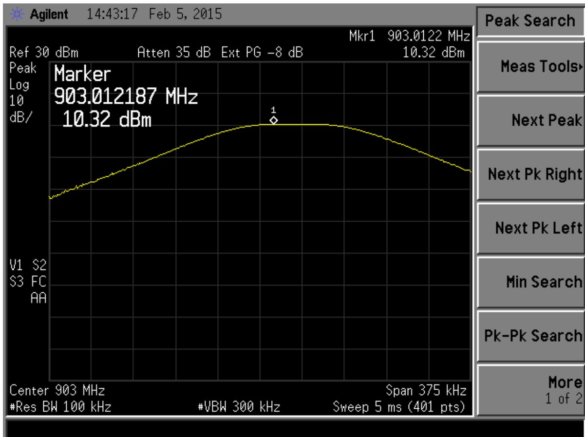
Figure 24. Peak Antenna Conducted Output Power, Low Channel
