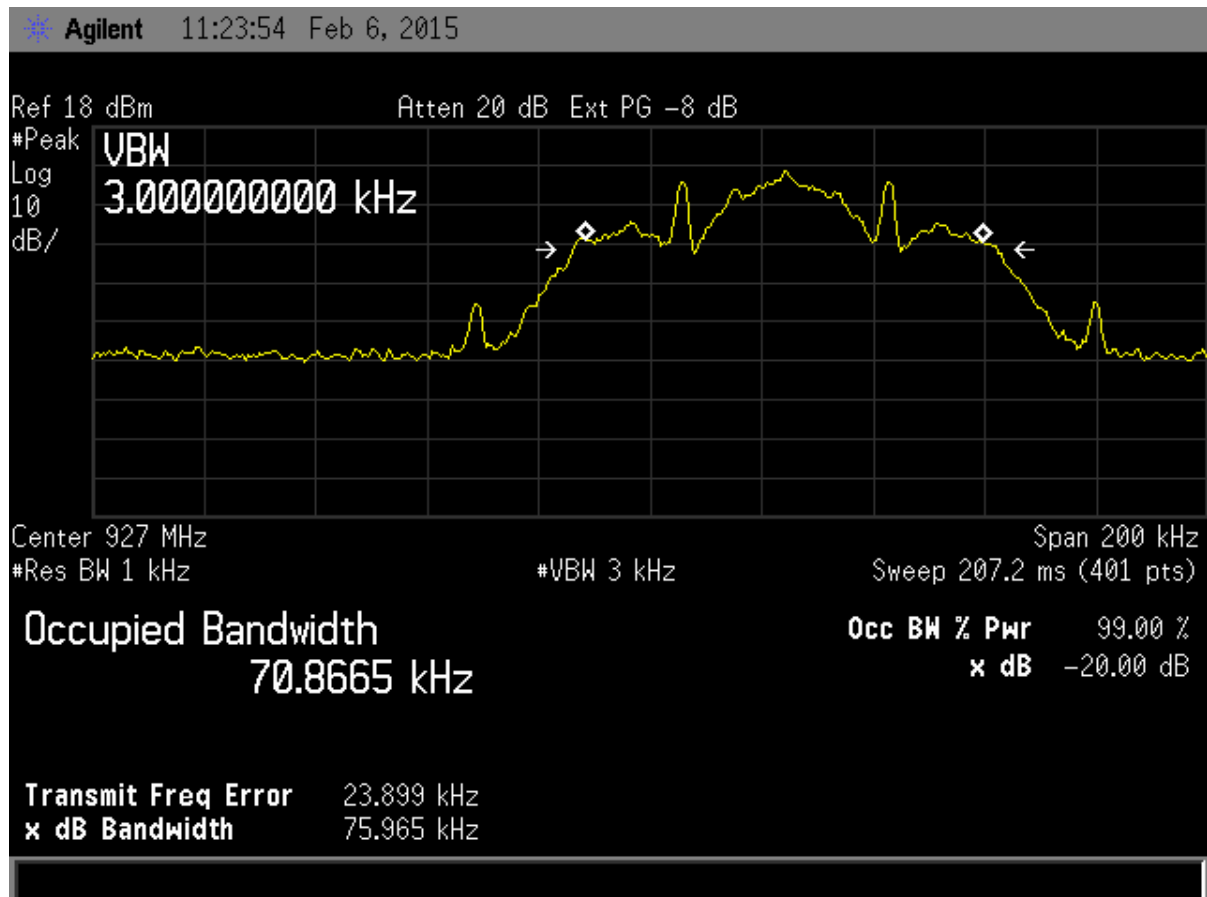
Figure 23. Twenty dB Bandwidth – High Channel
