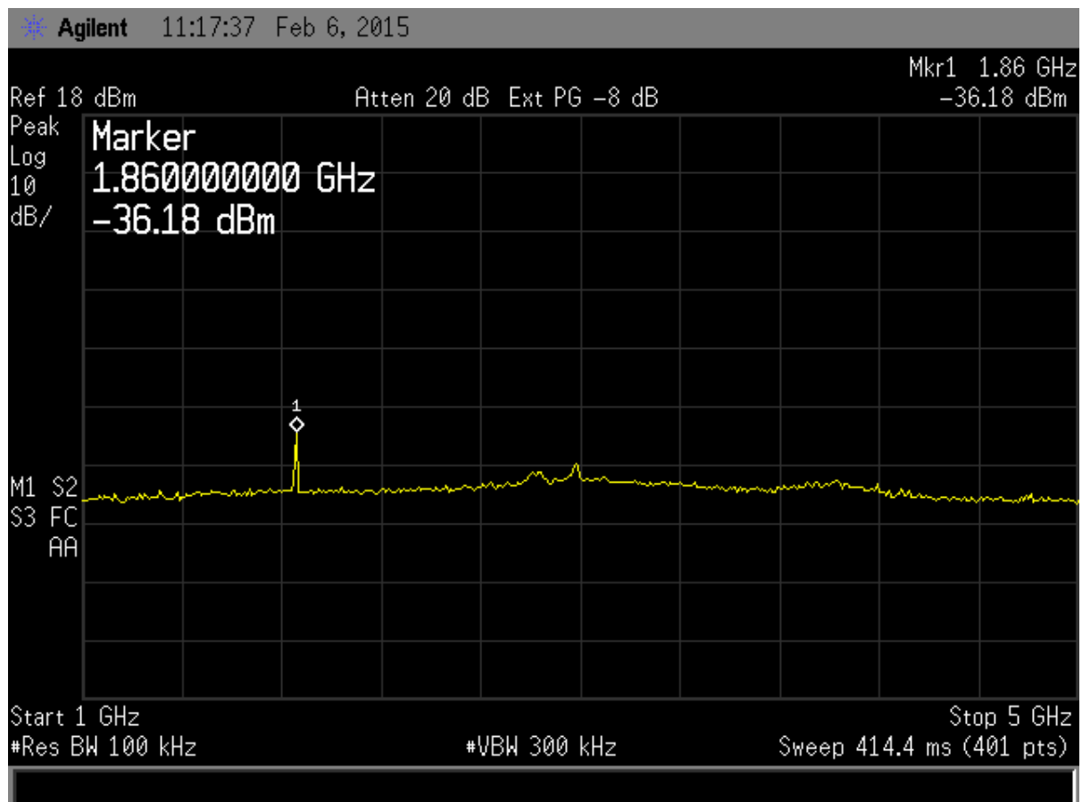
Figure 10. Antenna Conducted Emissions High, Part 2 GFSK modulation
