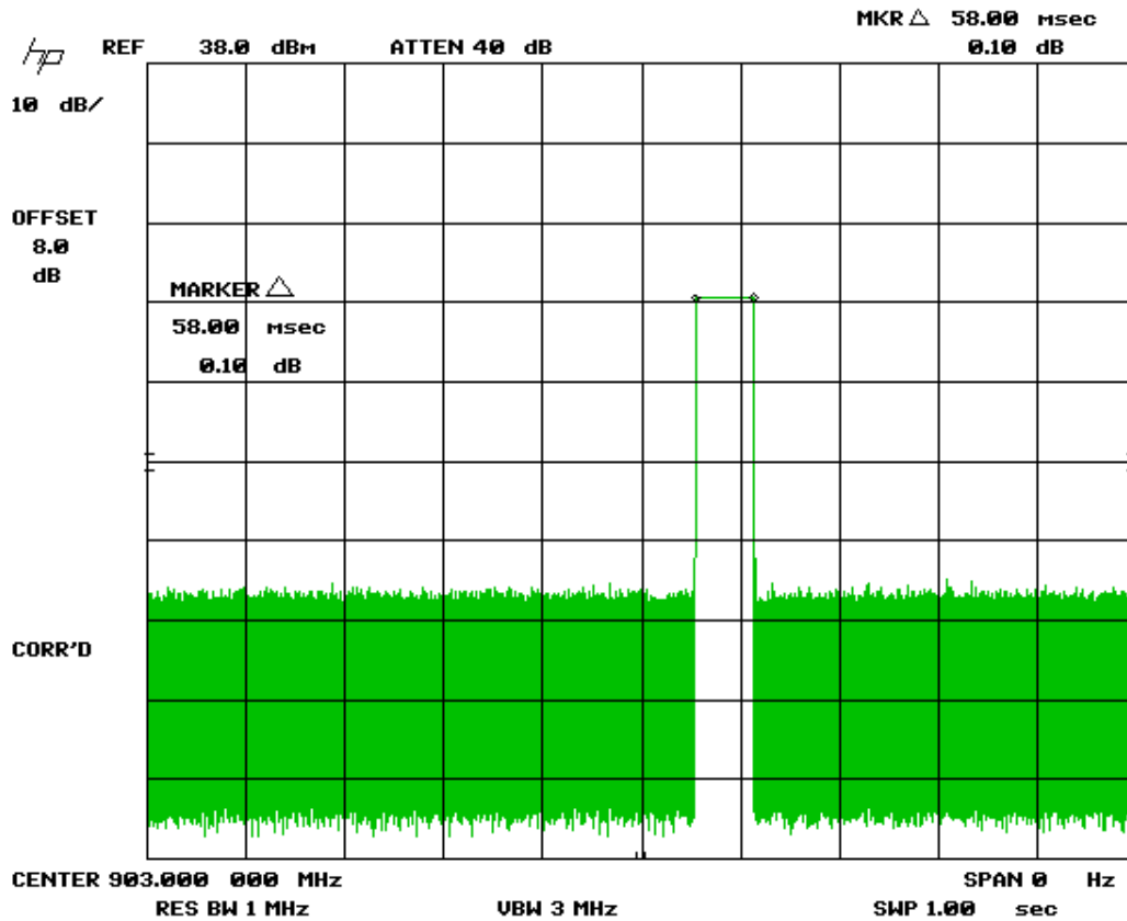
Figure 34. Time On
