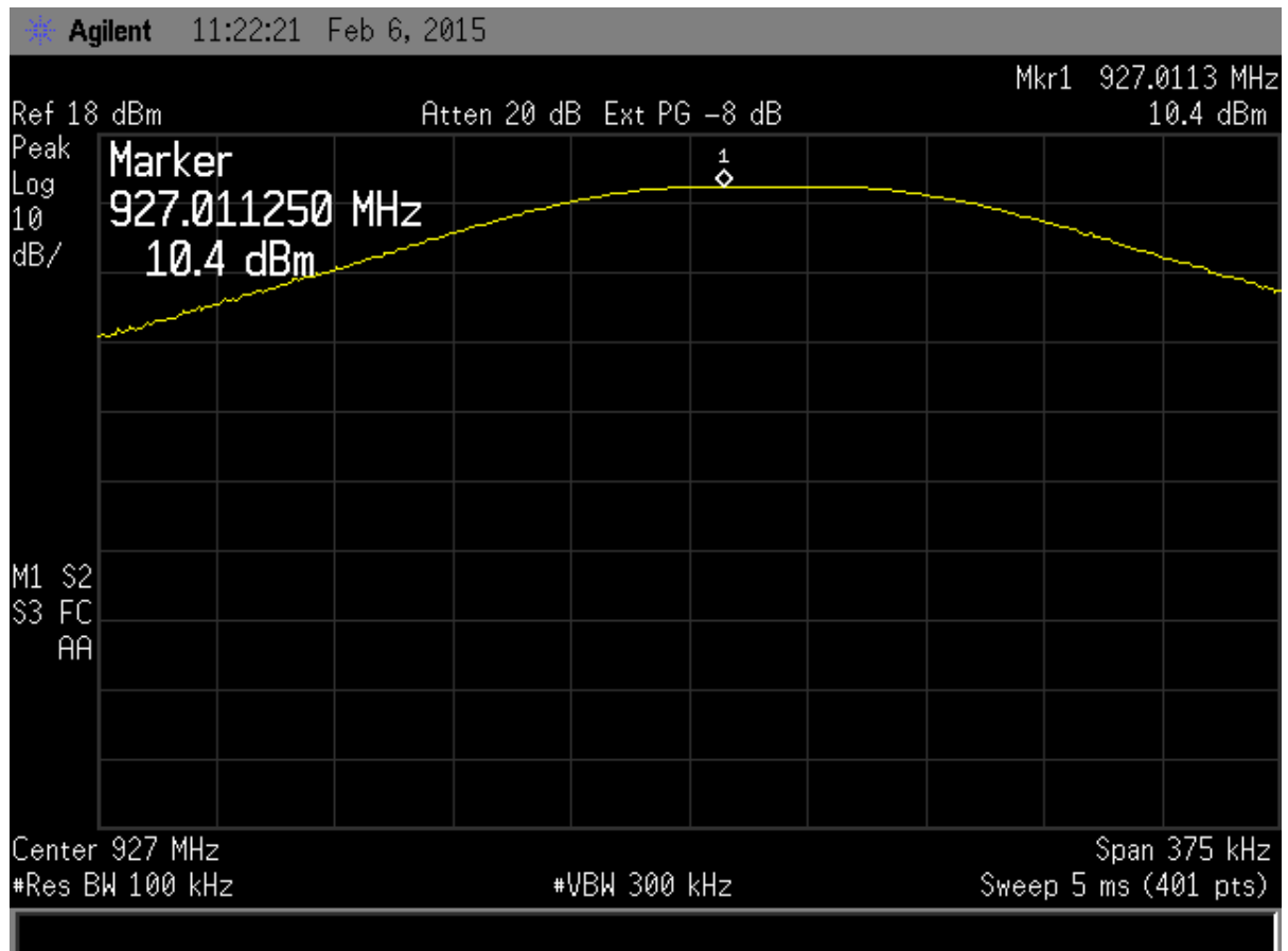
Figure 26. Peak Antenna Conducted Output Power, High Channel
