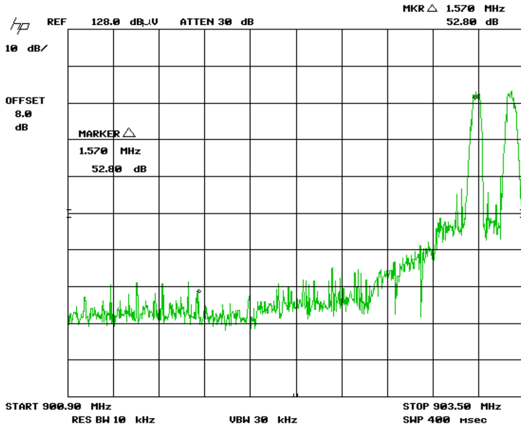
Figure 13. Band Edge Compliance, Low Channel Delta – Channel Hopping GFSK modulation
