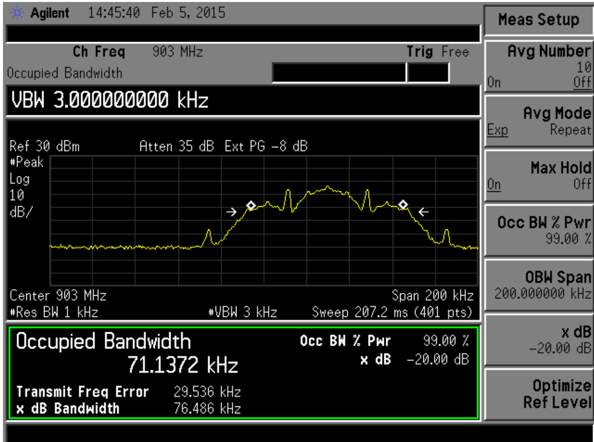
Figure 21. Twenty dB Bandwidth – Low Channel
