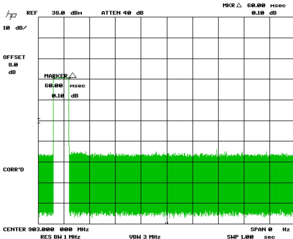
Figure 2. Transmitter Pulse Width in 1 Sec Period
