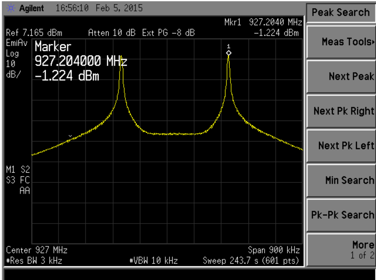
Figure 29. Peak Power Spectral Density, High Channel
