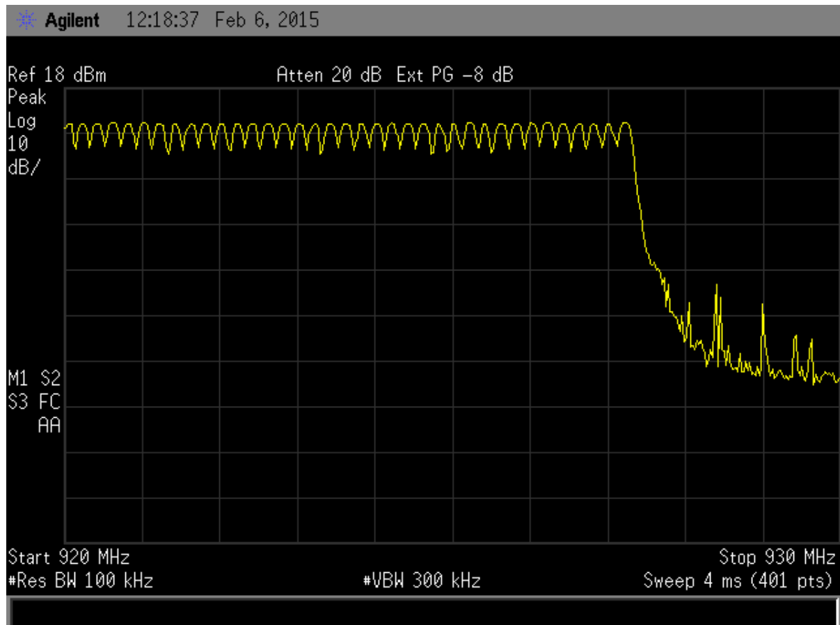
Figure 32. Hopping Channels 83 through 120
