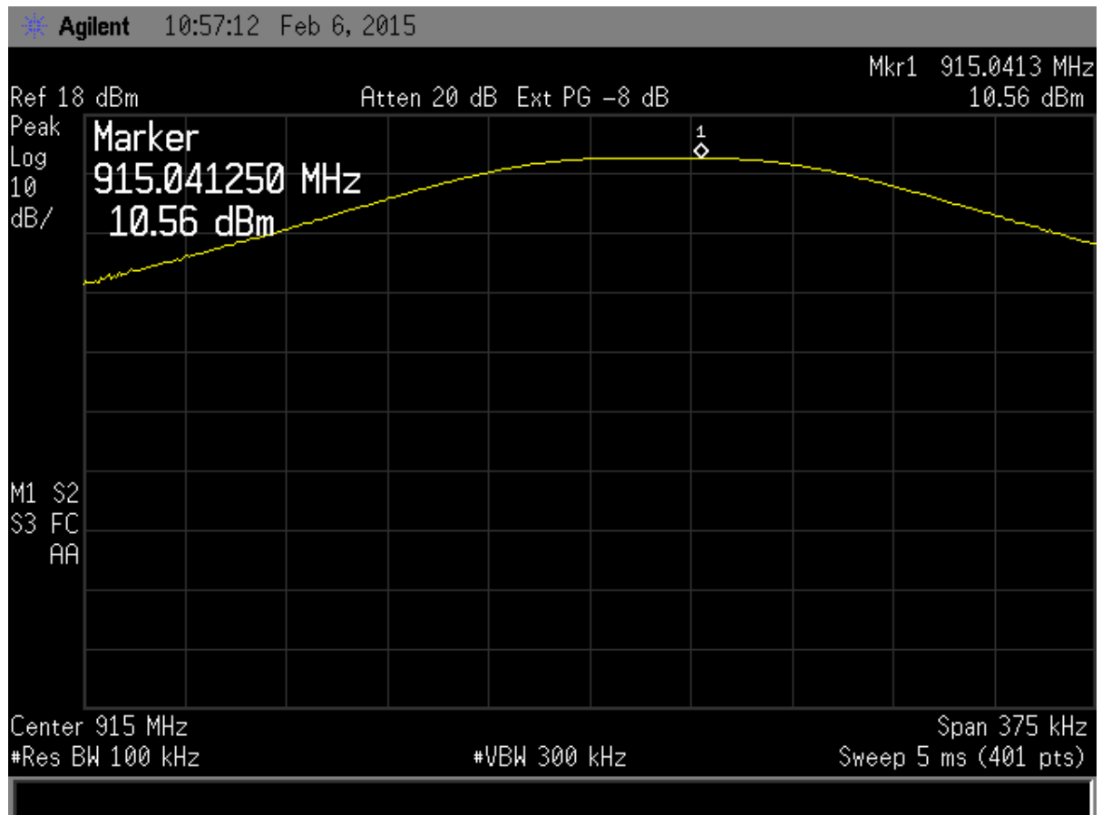
Figure 25. Peak Antenna Conducted Output Power, Mid Channel
