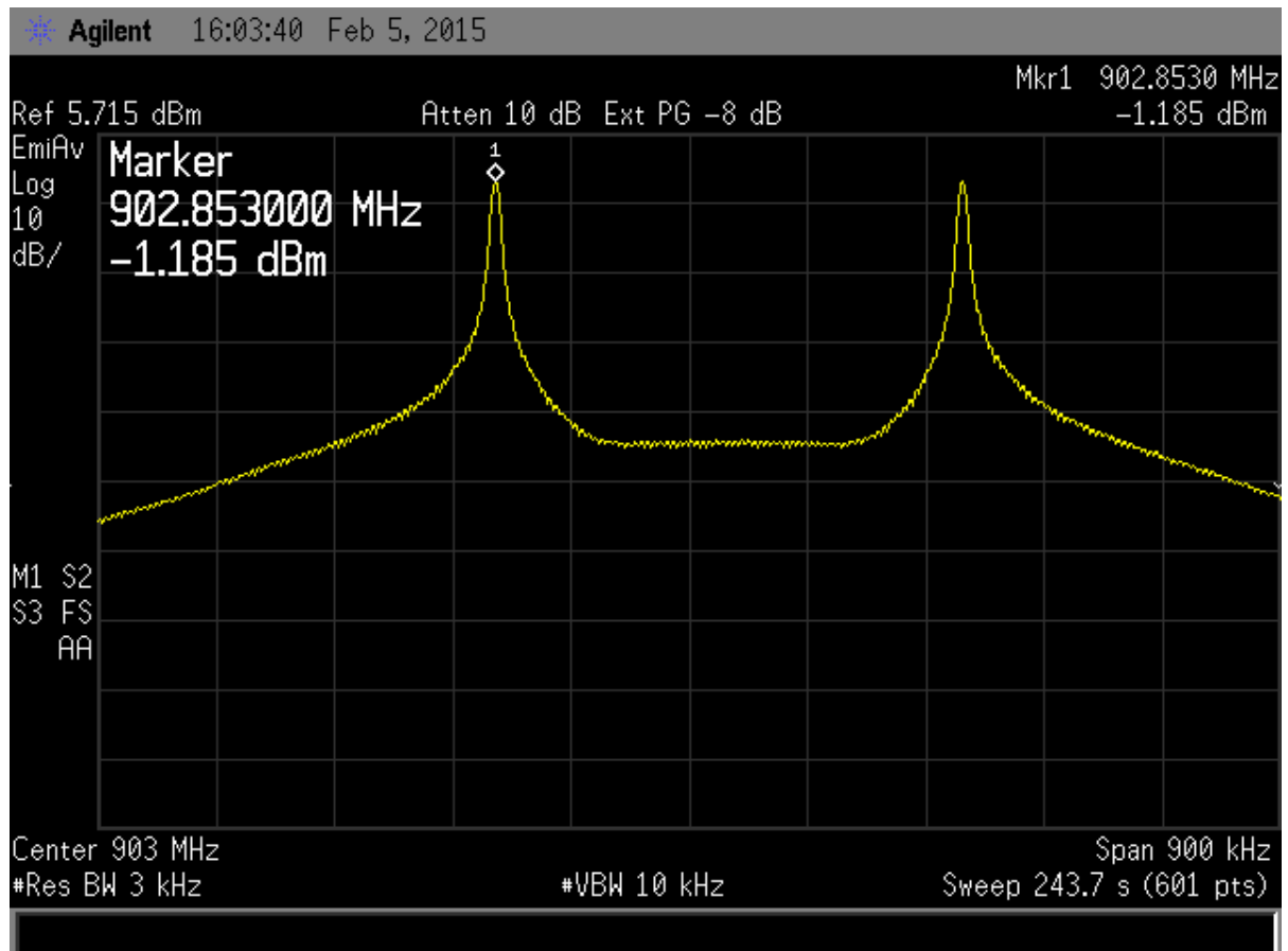
Figure 27. Peak Power Spectral Density, Low Channel
