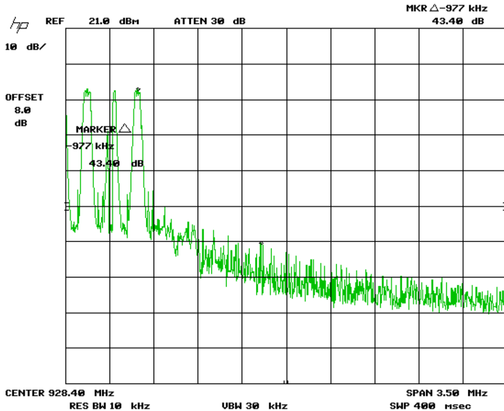
Figure 15. Band Edge Compliance, High Channel Delta – Channel Hopping GFSK modulation
