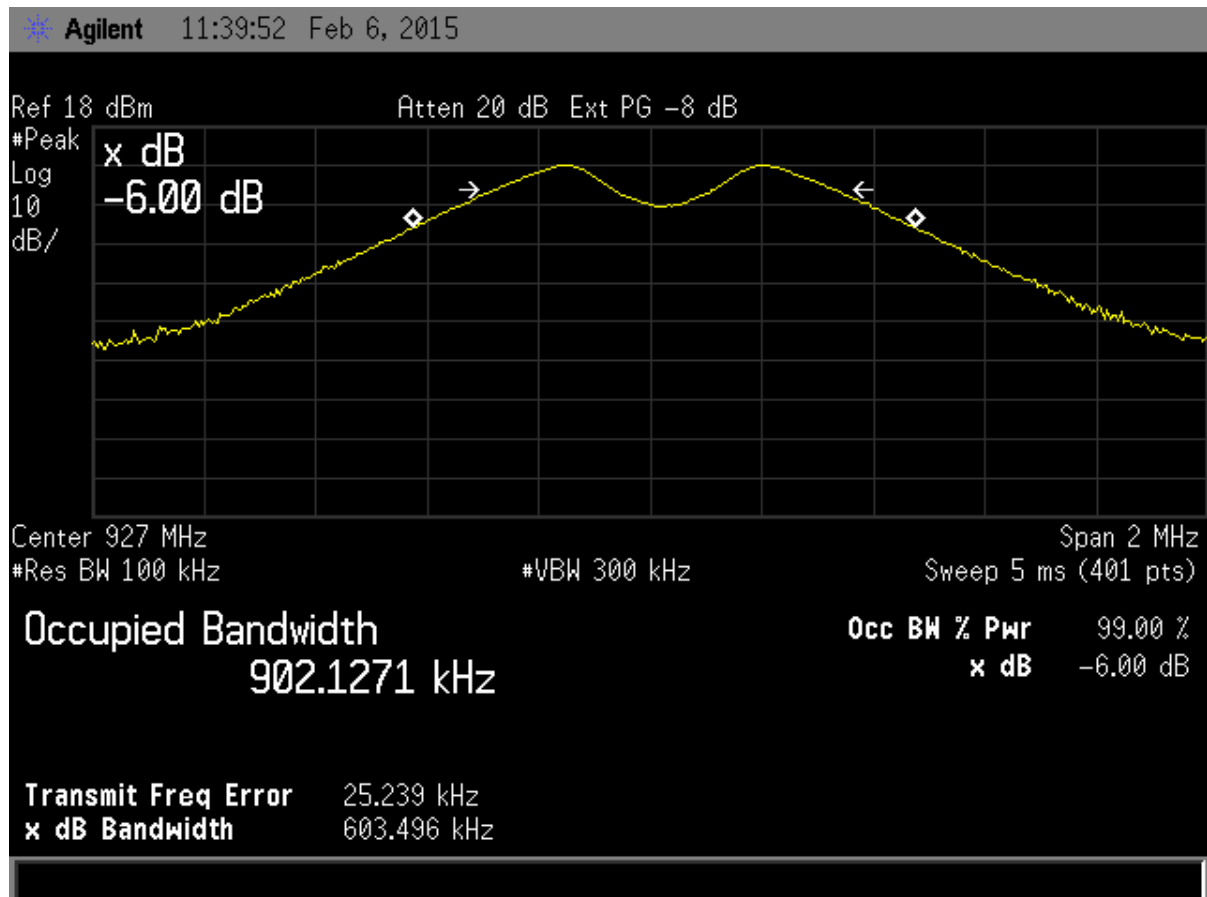
Figure 20. Six dB Bandwidth - 15.247 - High Channel
