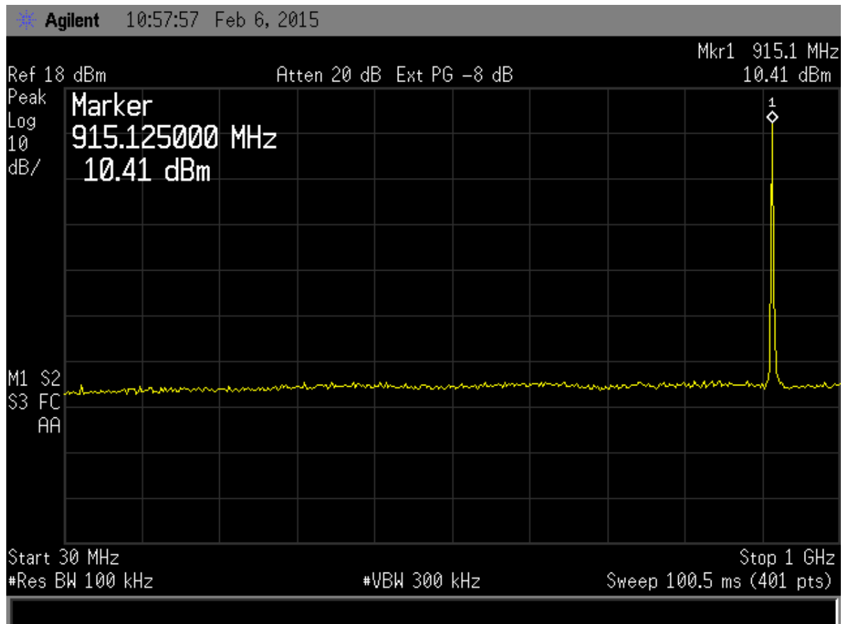
Figure 6. Antenna Conducted Emissions Mid, Part 1 GFSK Modulation
