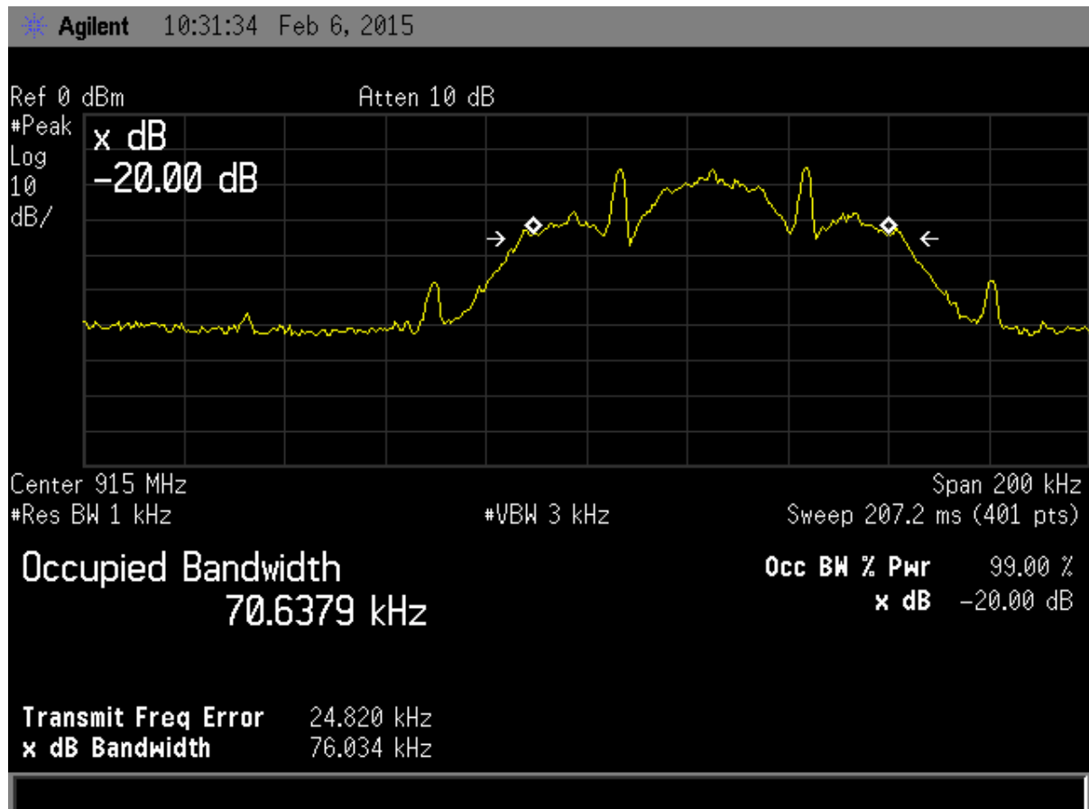
Figure 22. Twenty dB Bandwidth – Mid Channel
