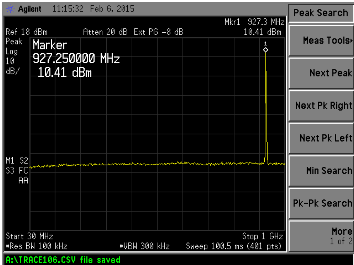
Figure 9. Antenna Conducted Emissions High, Part 1 GFSK modulation
