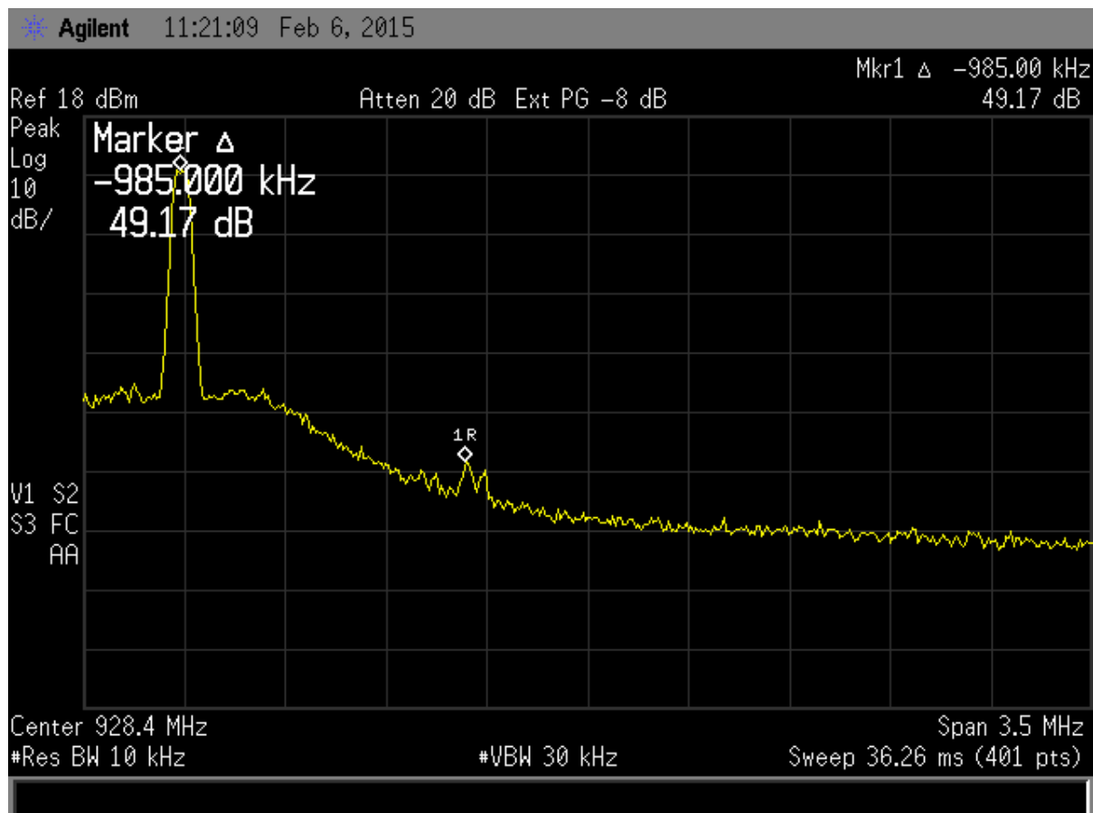
Figure 14. Band Edge Compliance, High Channel Delta – Continuous Transmission GFSK modulation
