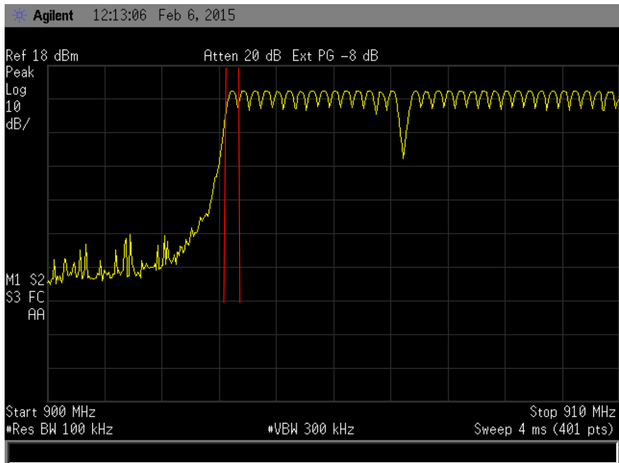
Figure 30. Hopping Channels 0 through 32
