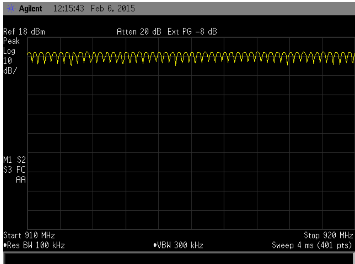
Figure 31. Hopping Channels 33 through 82
