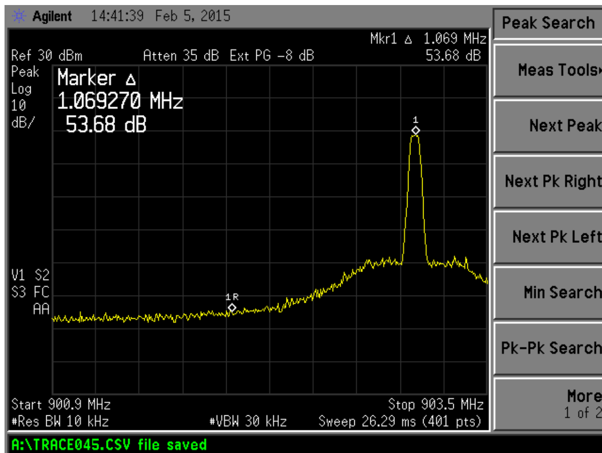
Figure 12. Band Edge Compliance, Low Channel Delta – Continuous Transmission GFSK modulation
