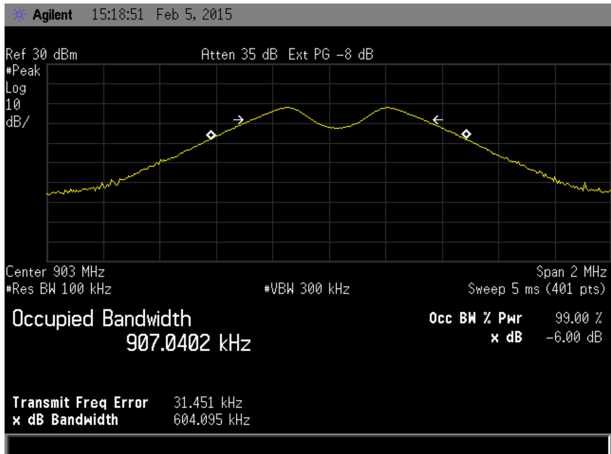
Figure 18. Six dB Bandwidth - 15.247 - Low Channel
