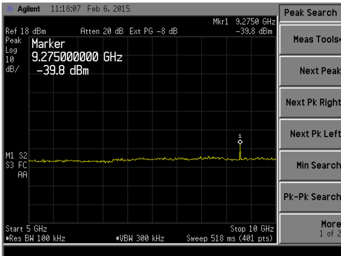
Figure 11. Antenna Conducted Emissions High, Part 3 GFSK modulation
