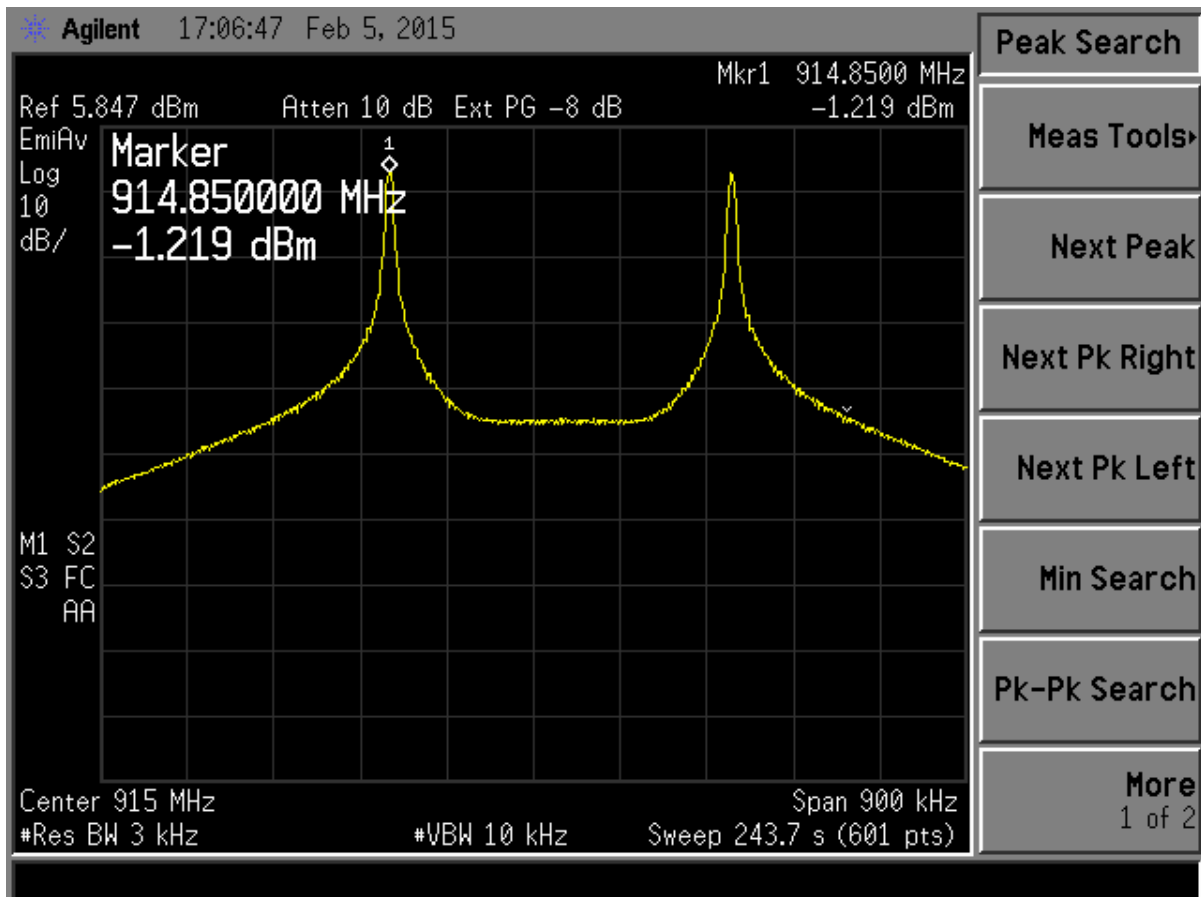
Figure 28. Peak Power Spectral Density, Mid Channel
