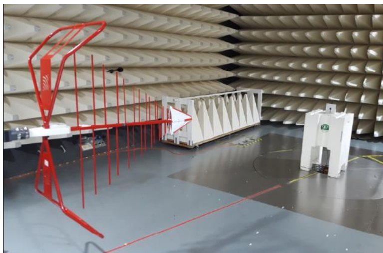
Figure B2: Radiated Low range Setup 30 – 960 MHz
