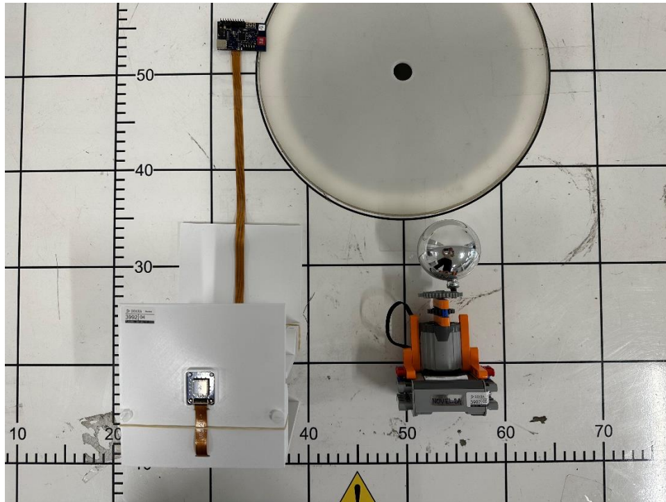
5. View of the DUT and accessories
