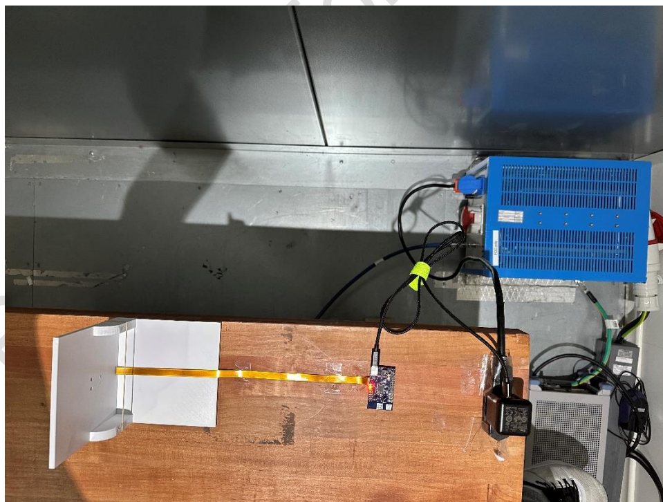
6. Conducted Emission Test Setup
