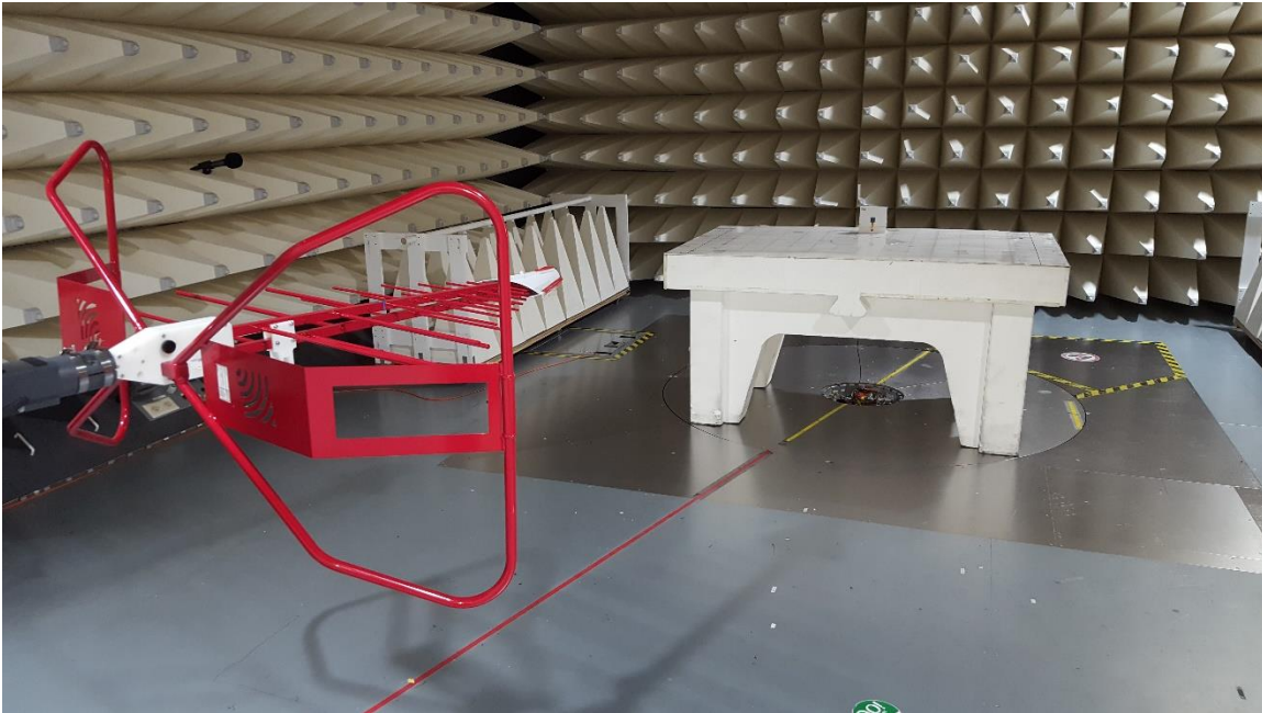
7. Low range Radiated Emission Test Setup
