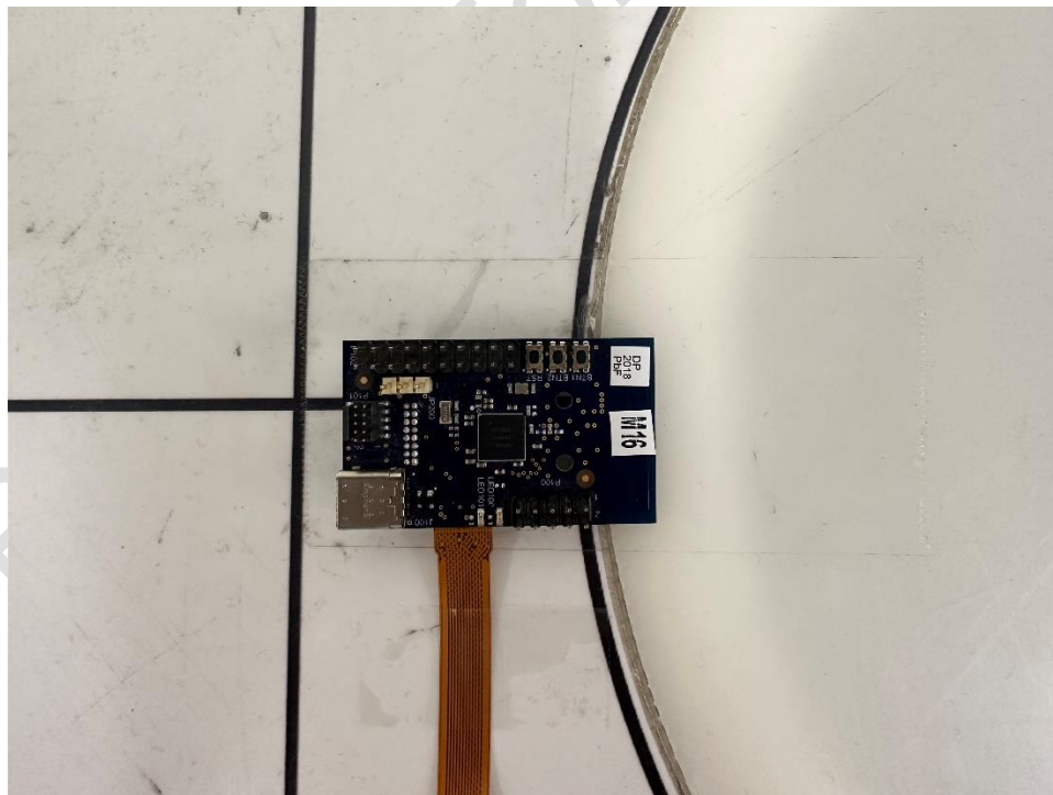
4. Detail view of the DUT Controller board (XTMCU06)
