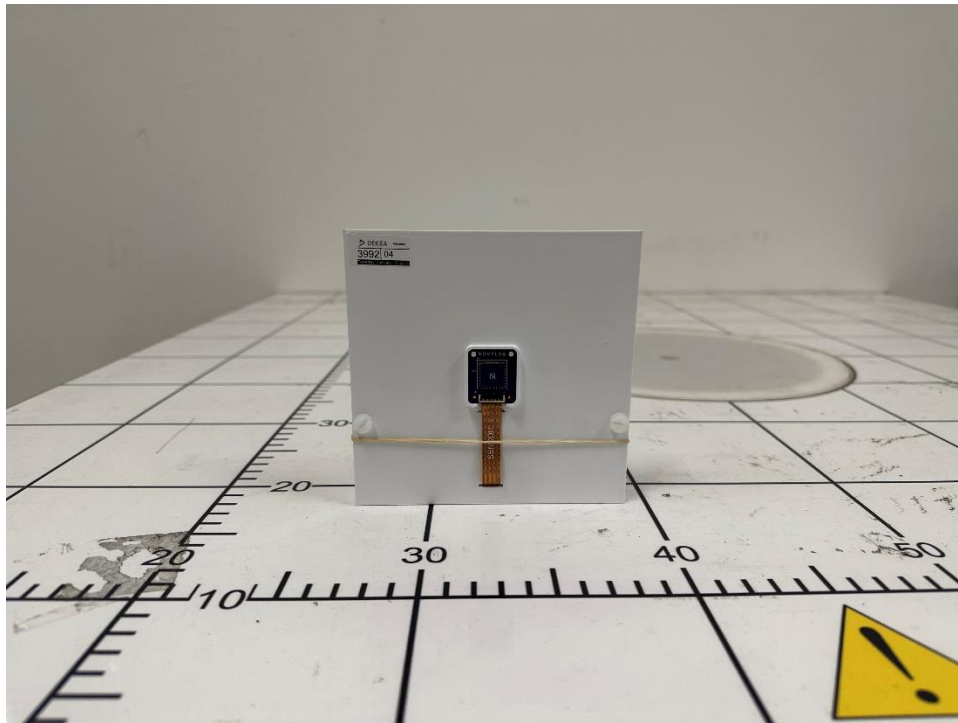
1. Front view of the DUT (X4F103 Module) with the Adapter Board (XTT007), and Stand
