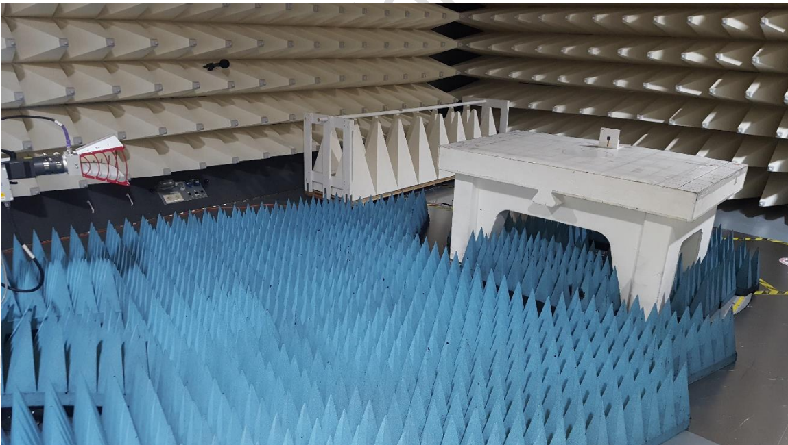
8. High range Radiated Emission Test Setup
