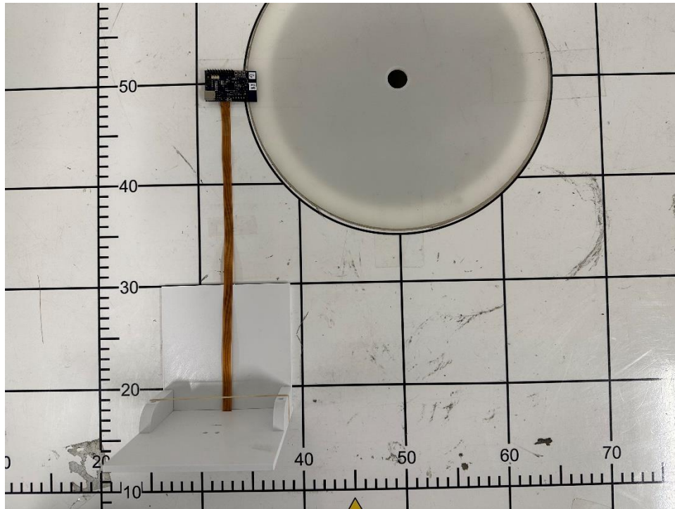
3. Top view of the Stand, Flex cable (FPC XTCBLP012), and Controller board (XTMCU06)
