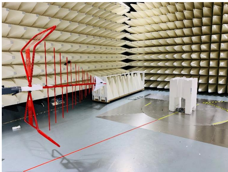
Figure B3: Radiated Low range Setup 30 – 960 MHz
