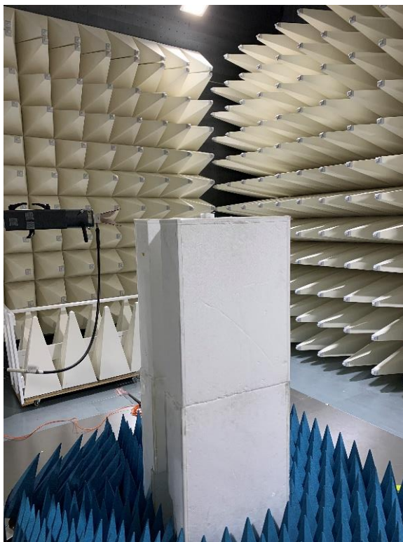
Figure B5: Radiated High range Setup 18 – 40 GHz
