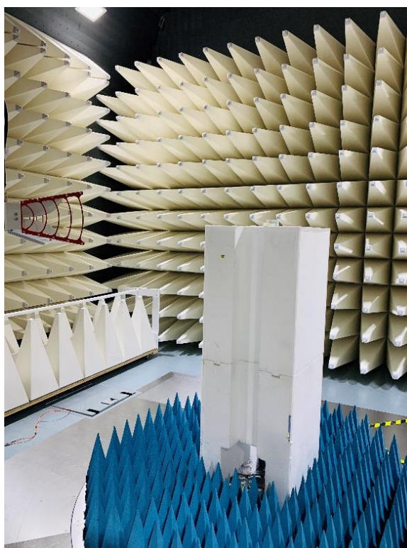
Figure B4: Radiated High range Setup 960 MHz – 18 GHz
