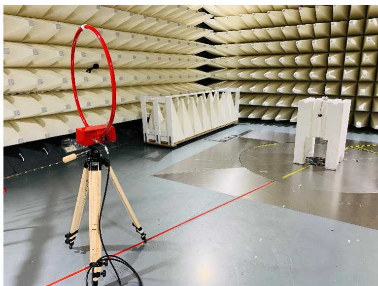
Figure B2: Radiated Low range Setup 9 kHz – 30 MHz.
