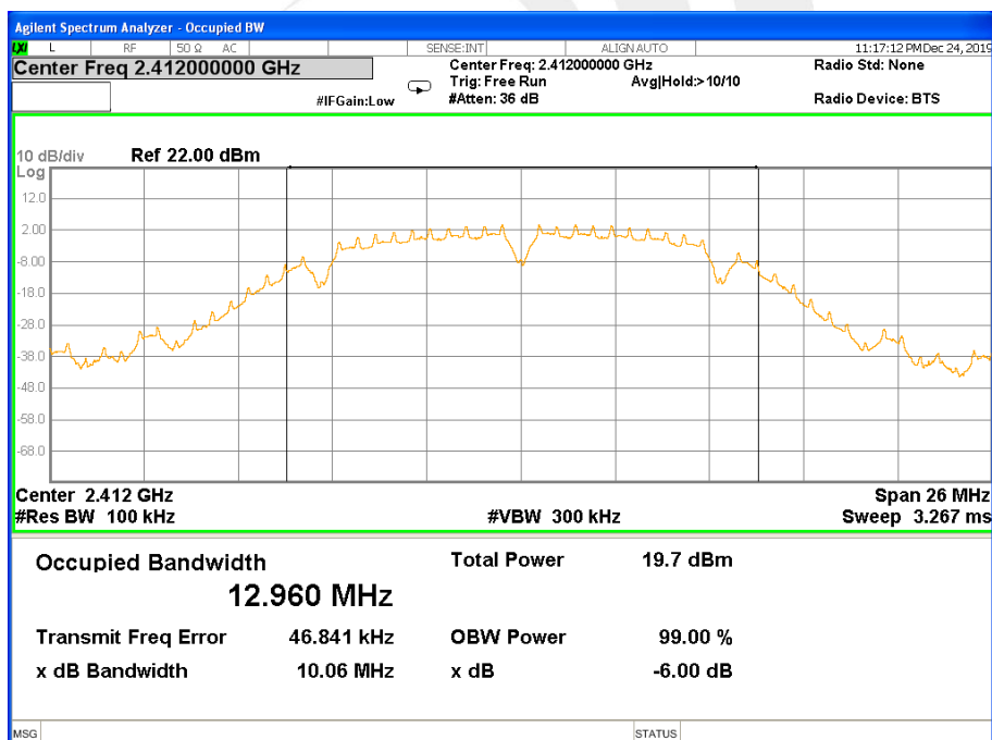
Antenna B 6dB Bandwidth TX CH 01
