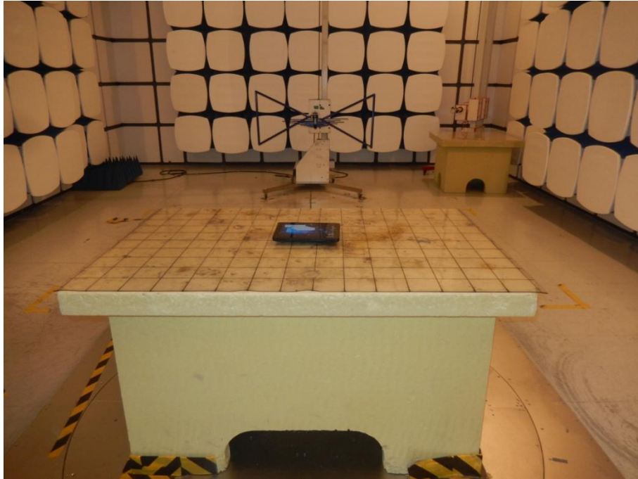
Radiated Measurement Photos 30MHz-1G
