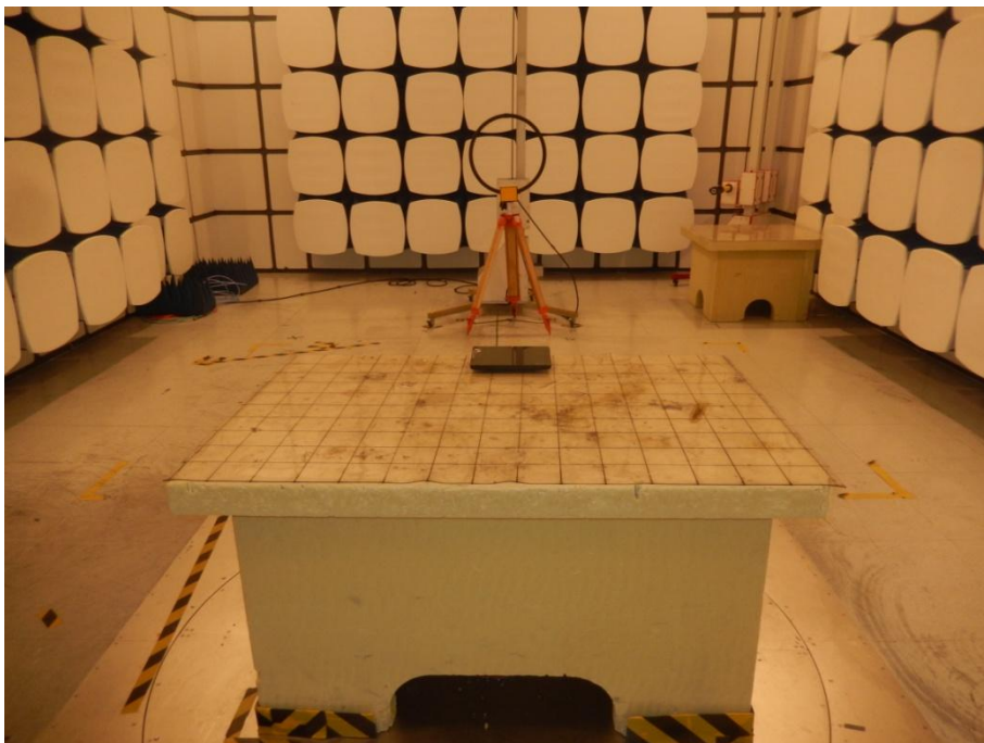
Radiated Measurement 9K-30MHz
