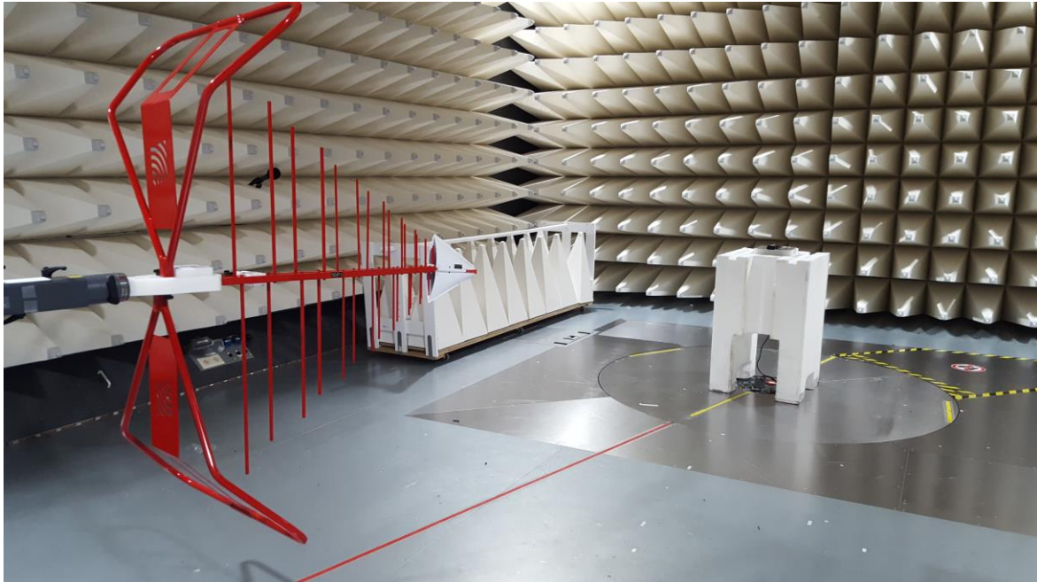
Figure C4. Radiated Setup – Low Range
