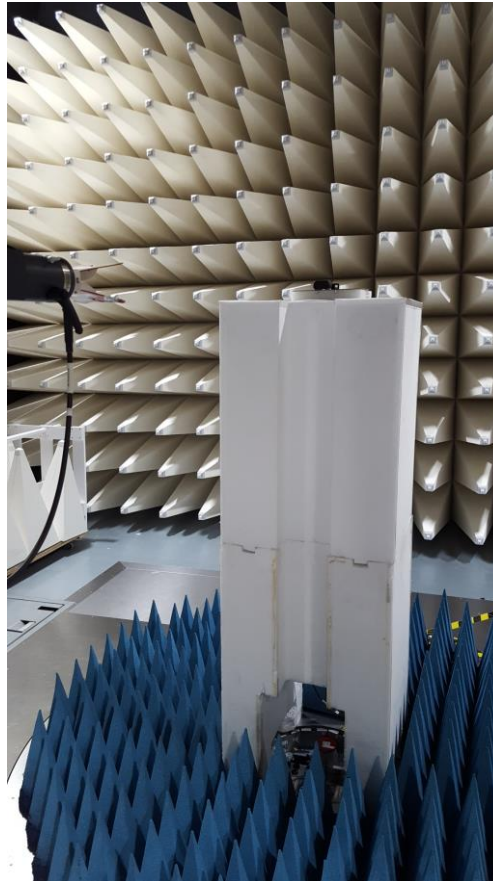
Figure C3. Radiated Setup – High Range
