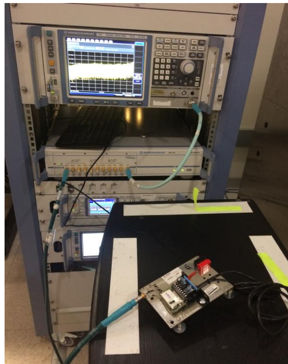
FigureC2. Conducted Test Setup
