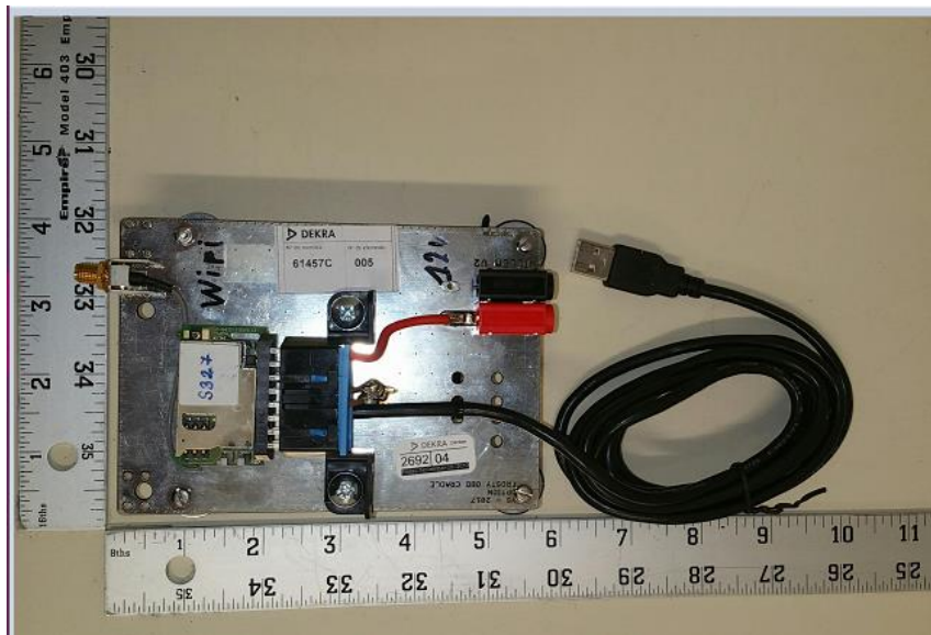
Figure C1: Conducted DUT
