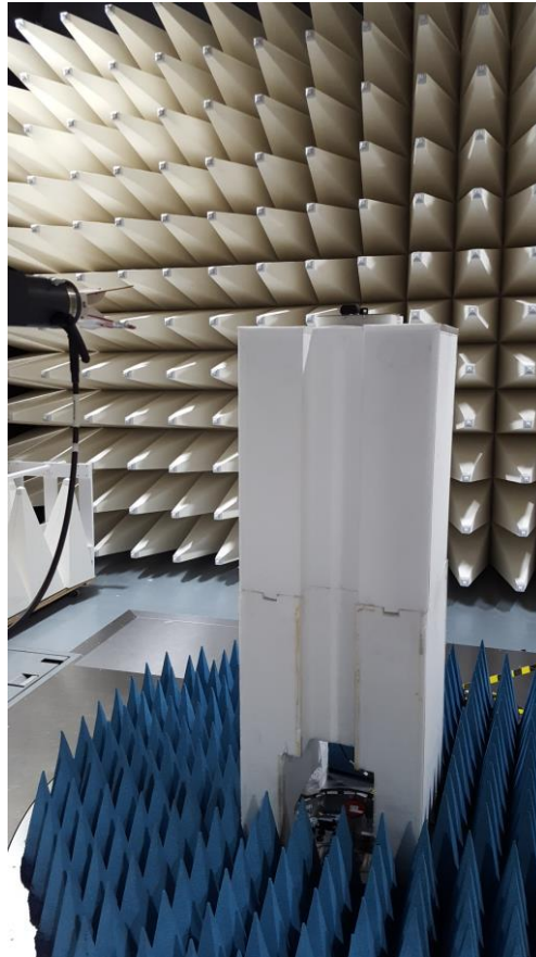
Figure C3. Radiated Setup – High Range
